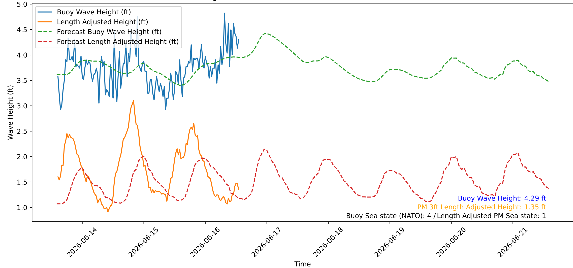
Wave Heights over Time for Red Beach at 2026-06-16 14:20:46
