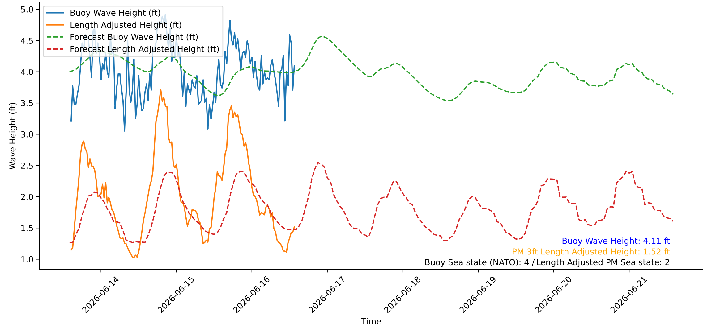
Wave Heights over Time for Green Beach at 2026-06-16 14:21:09
