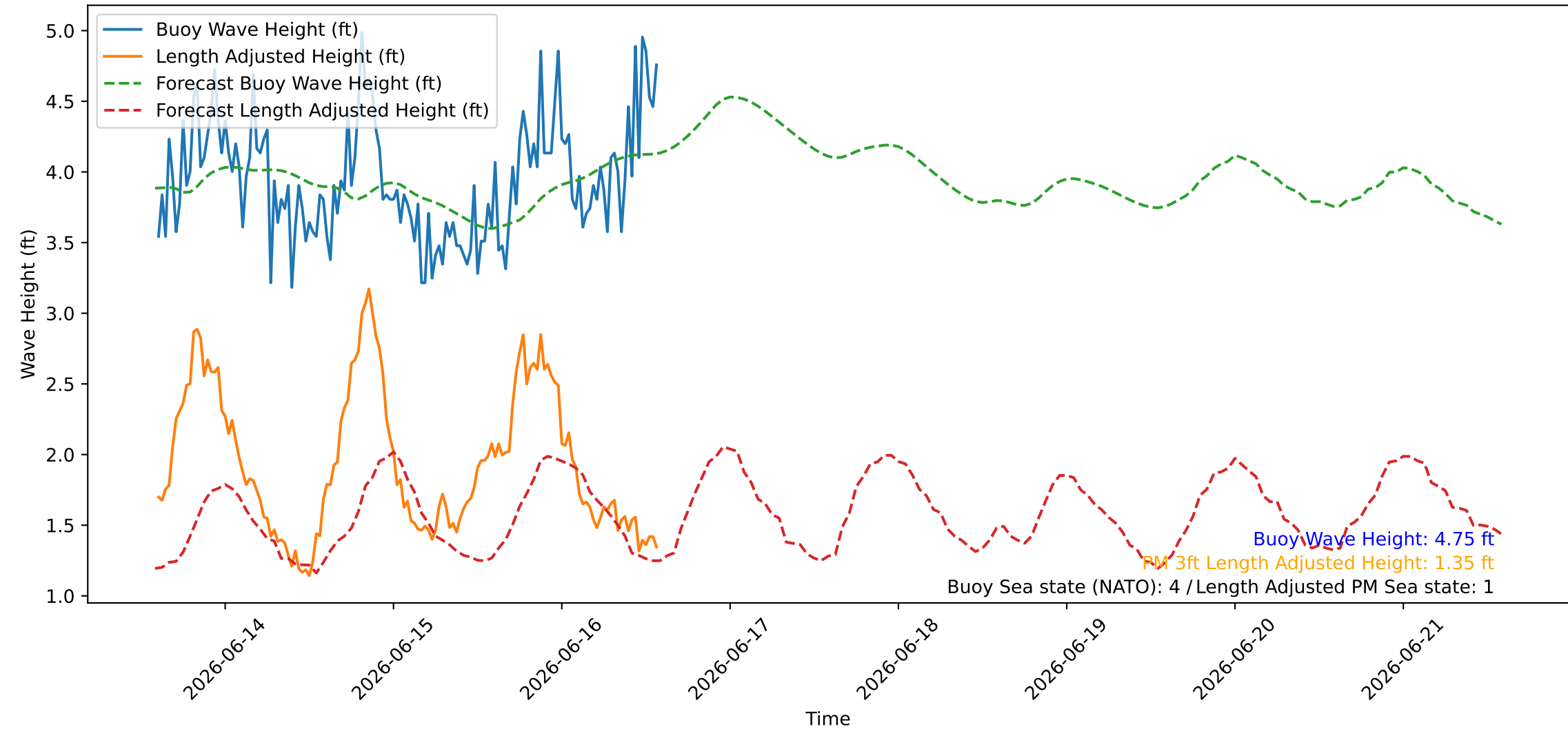
Wave Heights over Time for Oceanside Harbor at 2026-06-16 14:20:26
