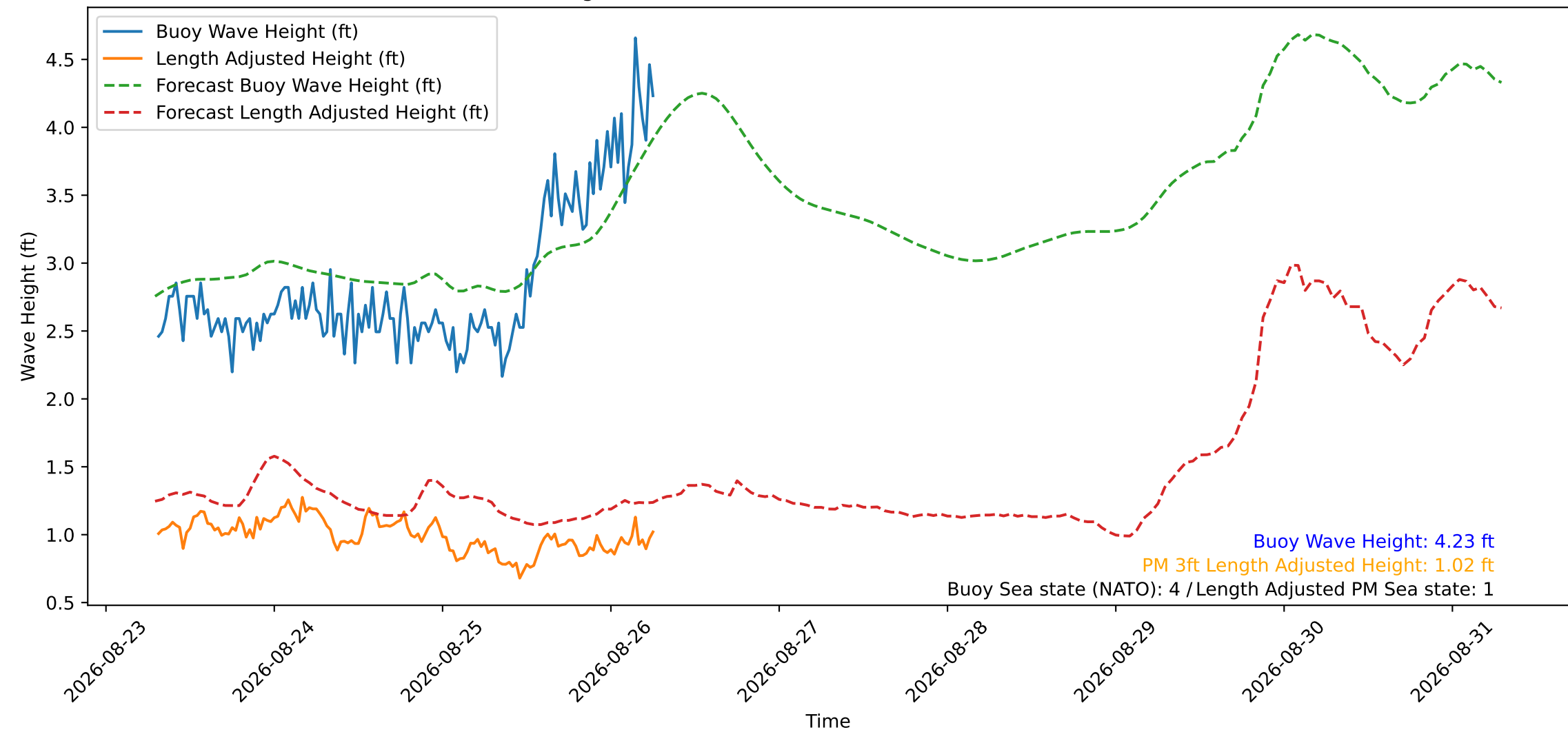
Wave Heights over Time for Red Beach at 2026-08-26 07:00:51
