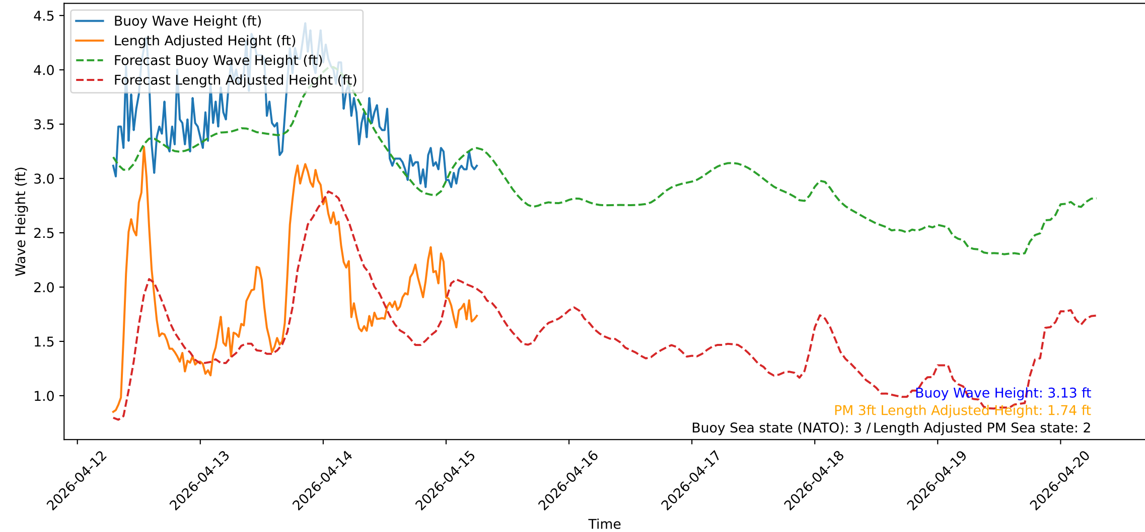
Wave Heights over Time for Red Beach at 2026-04-15 06:50:51
