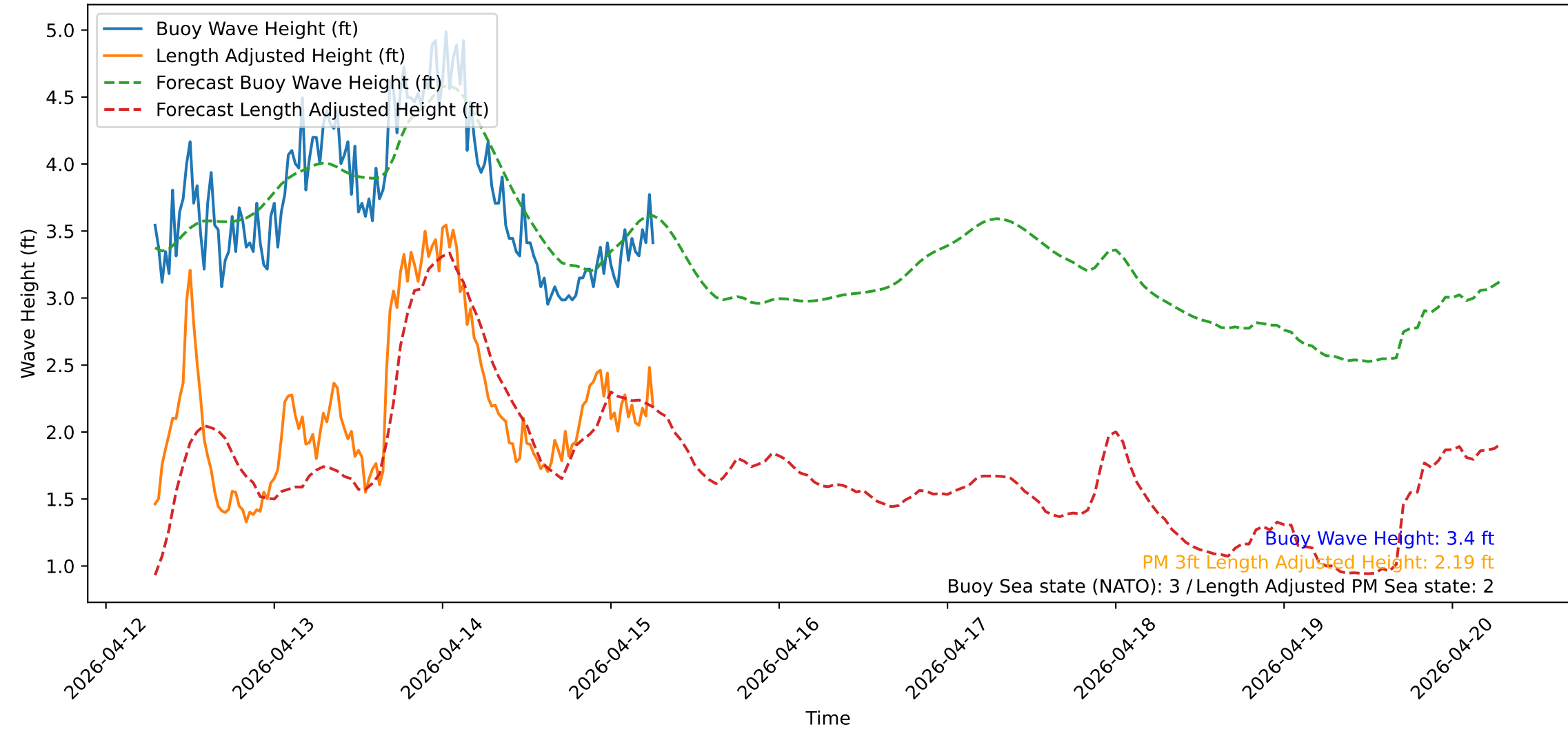
Wave Heights over Time for Green Beach at 2026-04-15 06:51:13
