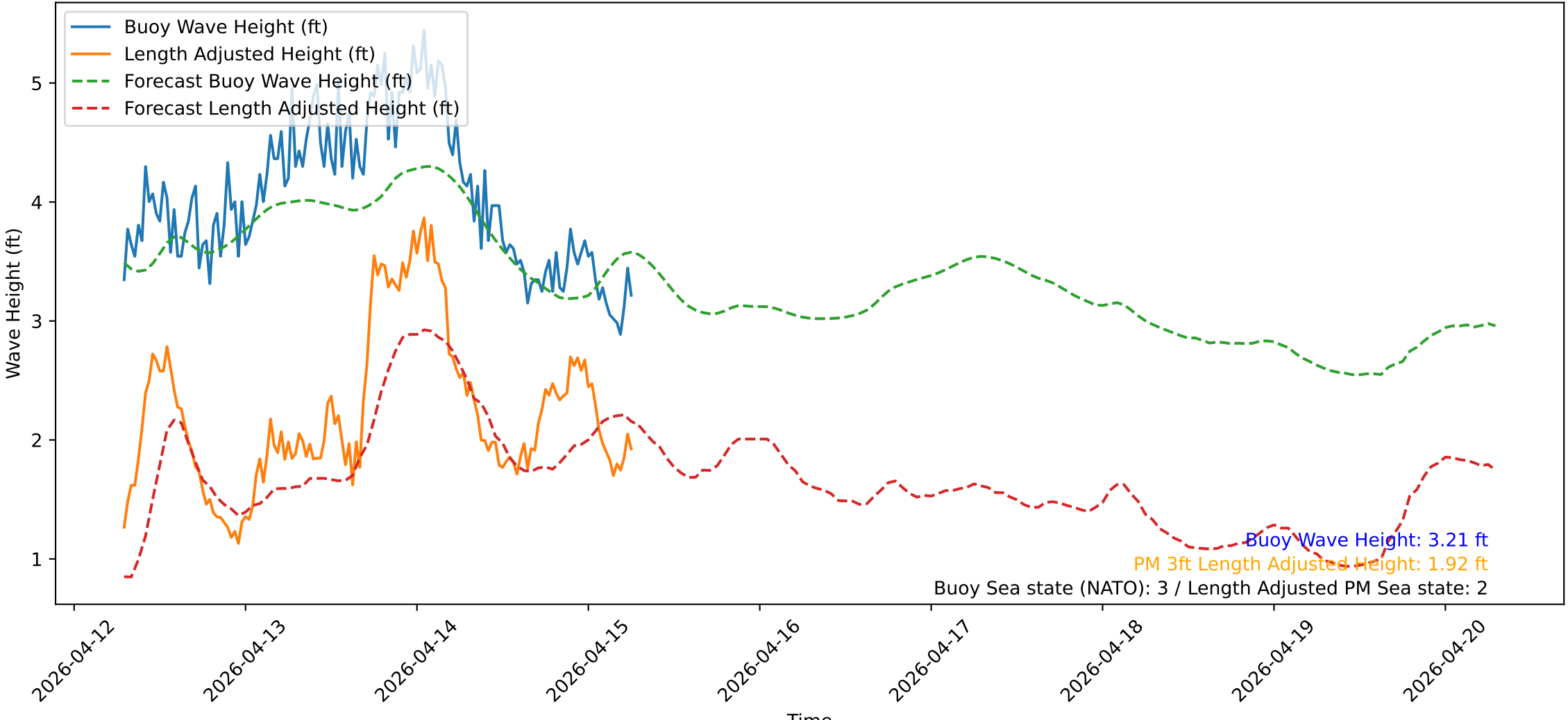
Wave Heights over Time for Oceanside Harbor at 2026-04-15 06:50:31
