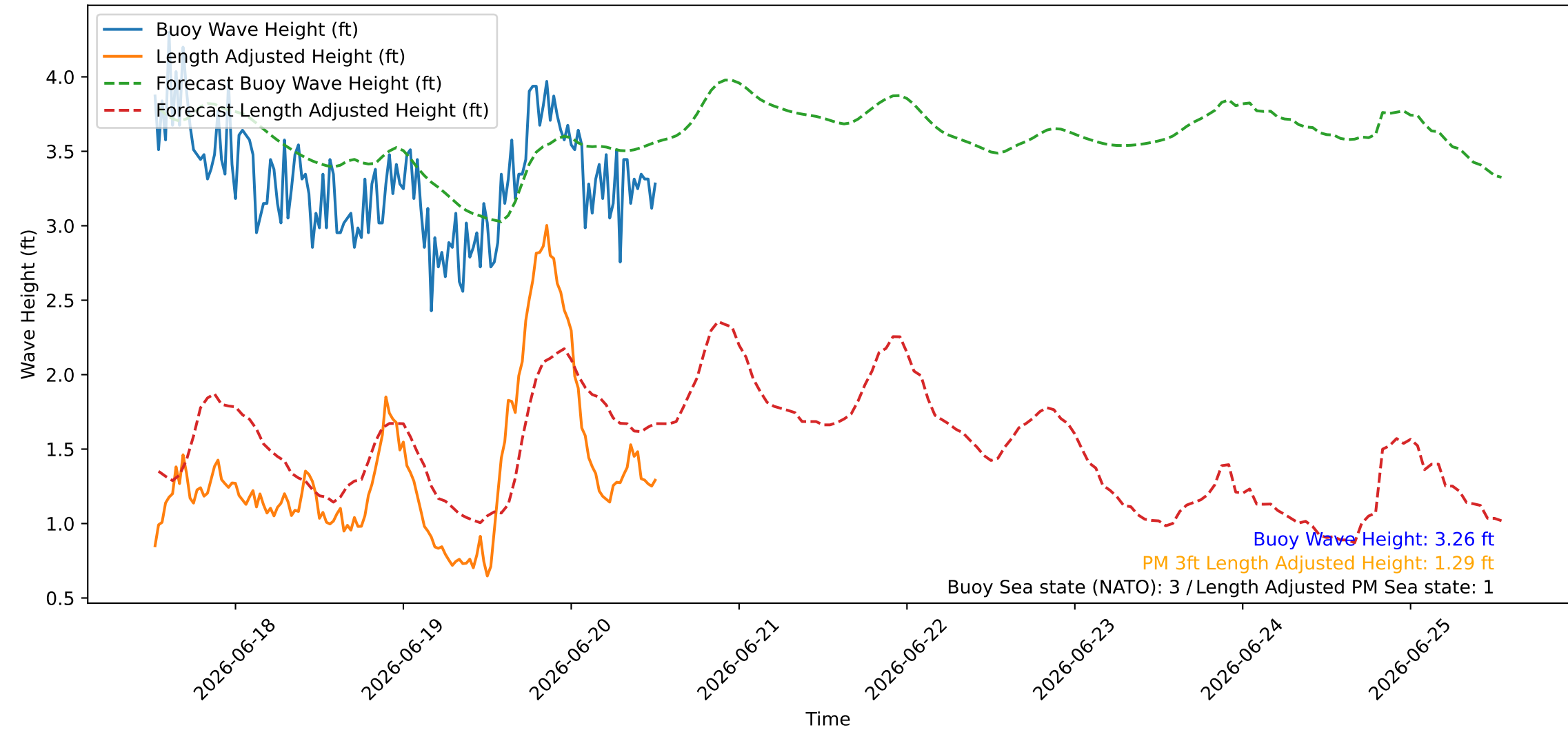
Wave Heights over Time for Green Beach at 2026-06-20 12:41:08
