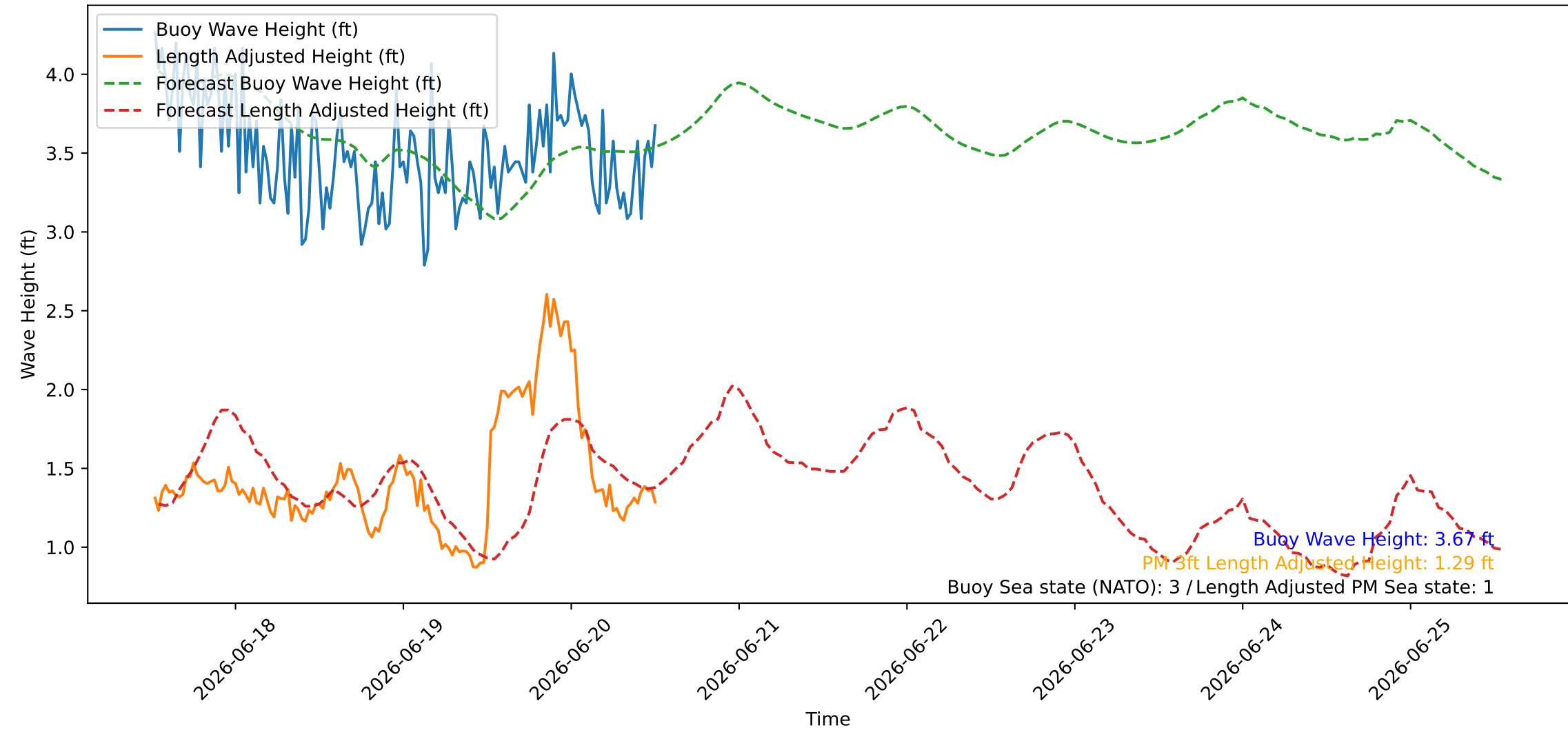
Wave Heights over Time for Oceanside Harbor at 2026-06-20 12:40:27
