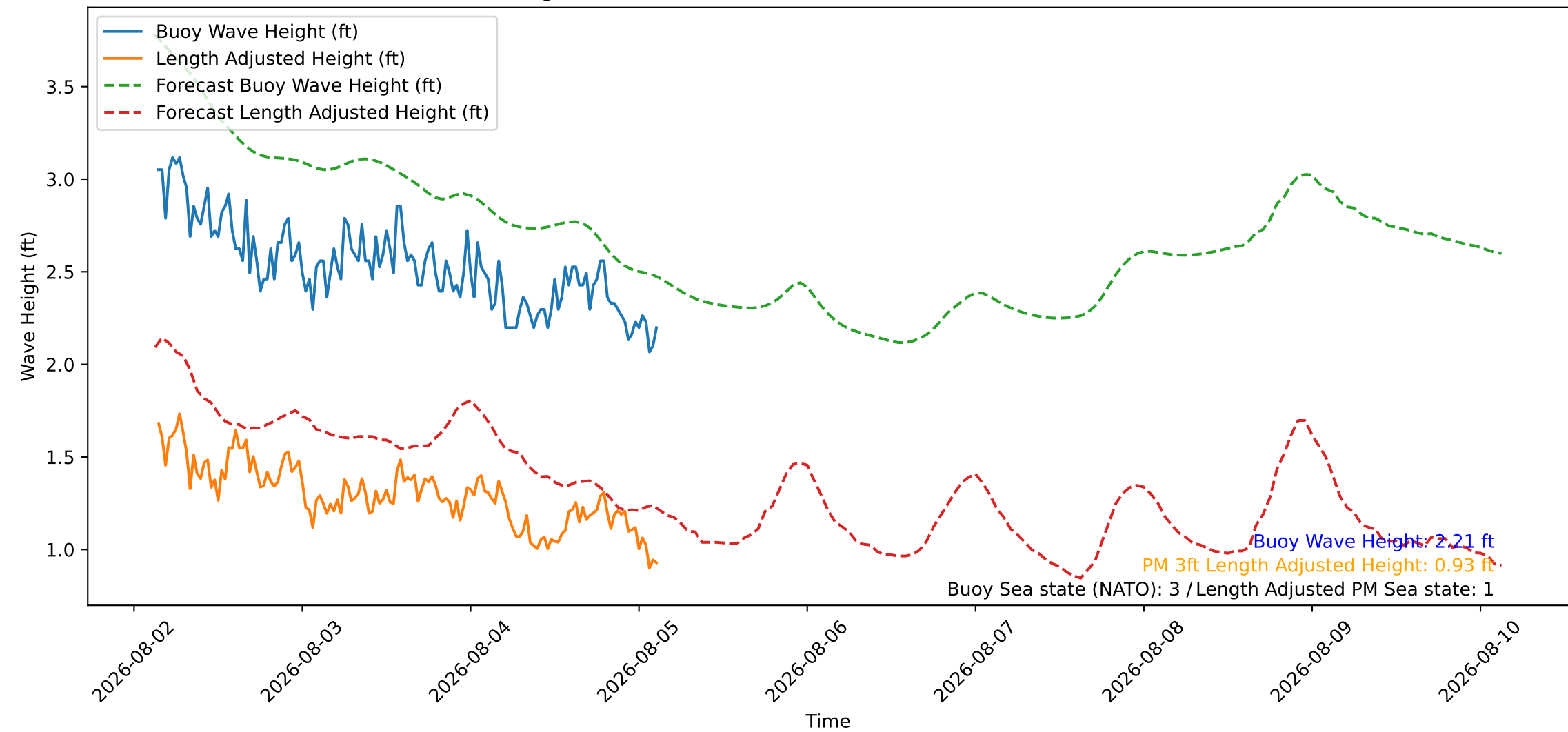
Wave Heights over Time for Oceanside Harbor at 2026-08-05 03:20:26
