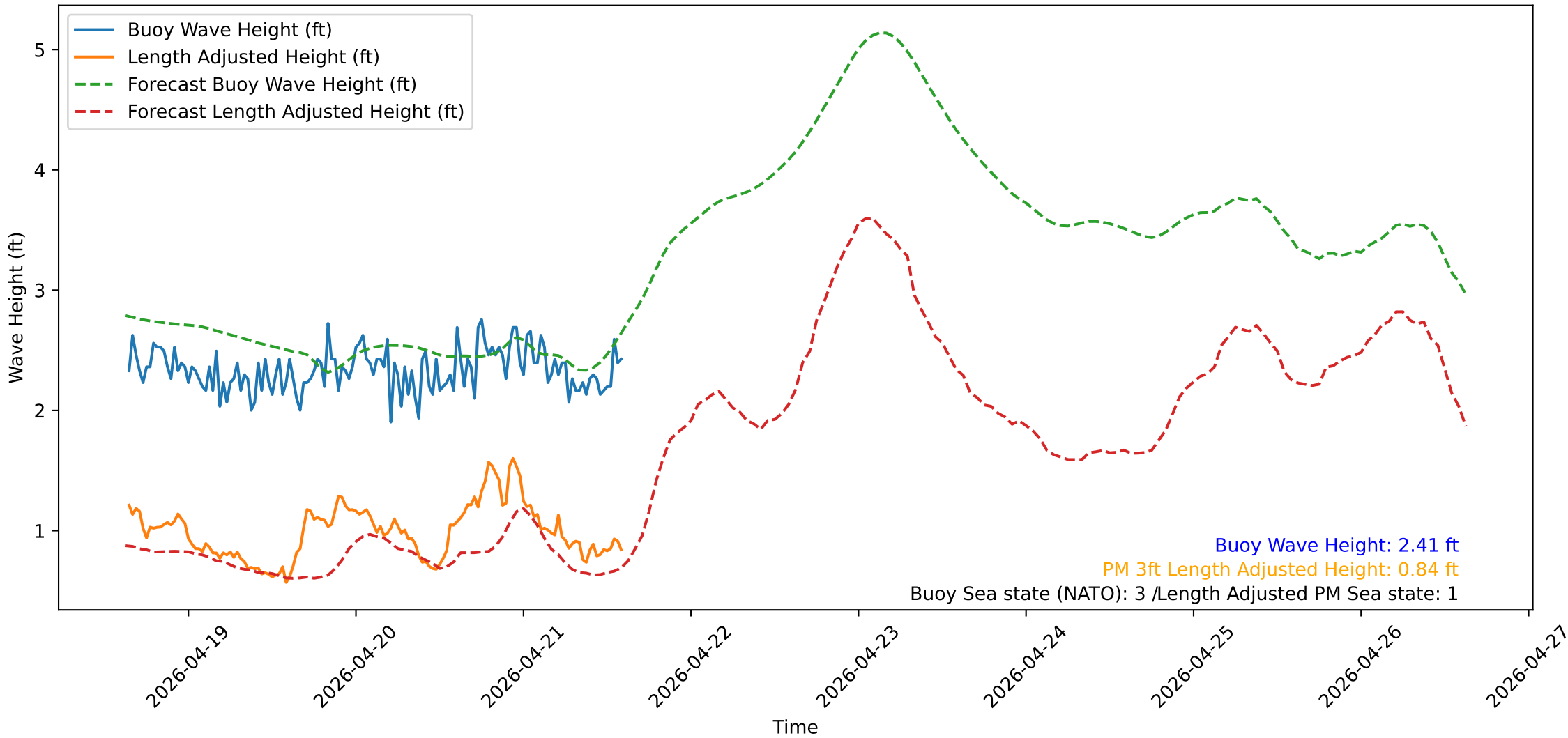
Wave Heights over Time for Oceanside Harbor at 2026-04-21 15:20:31
