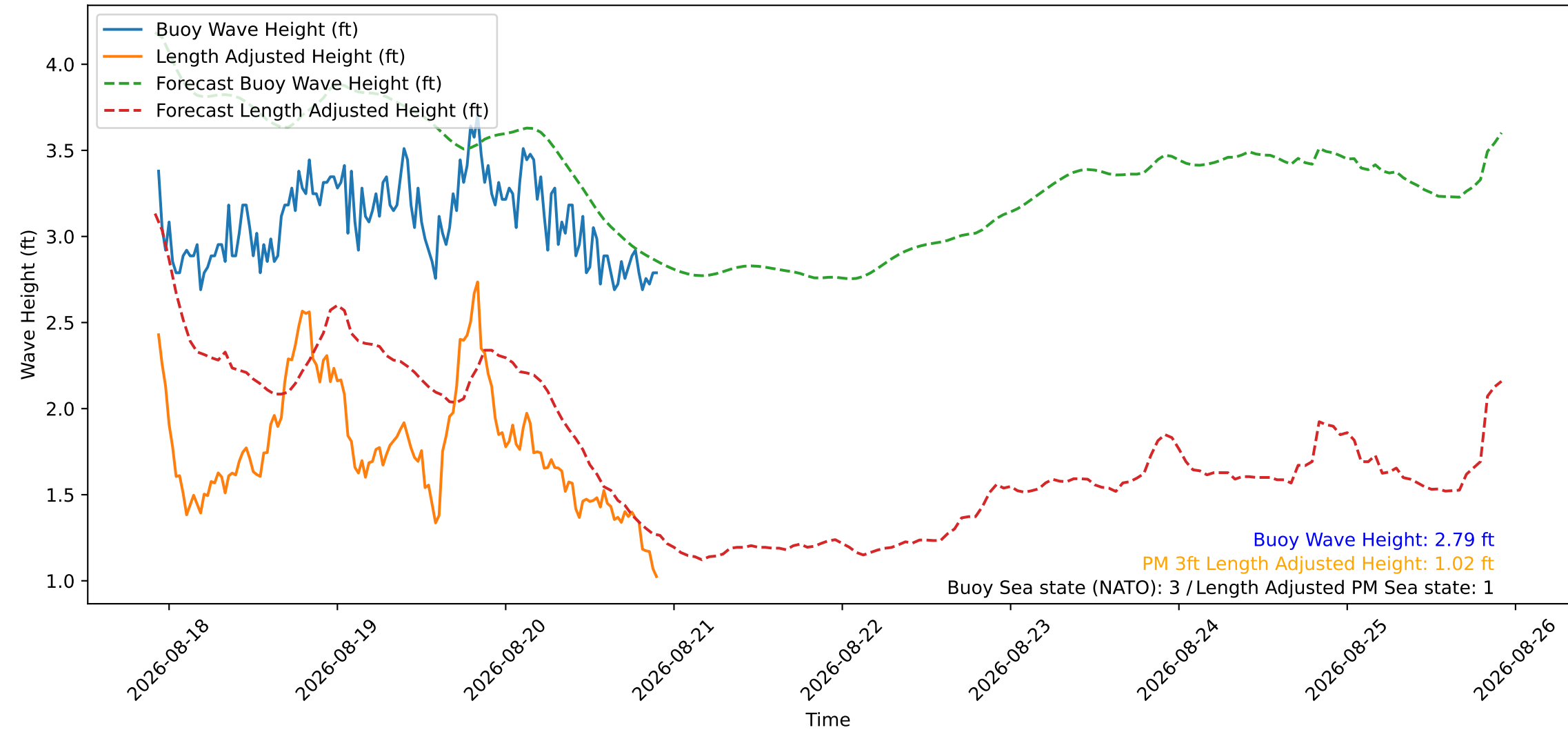
Wave Heights over Time for Green Beach at 2026-08-20 22:21:11
