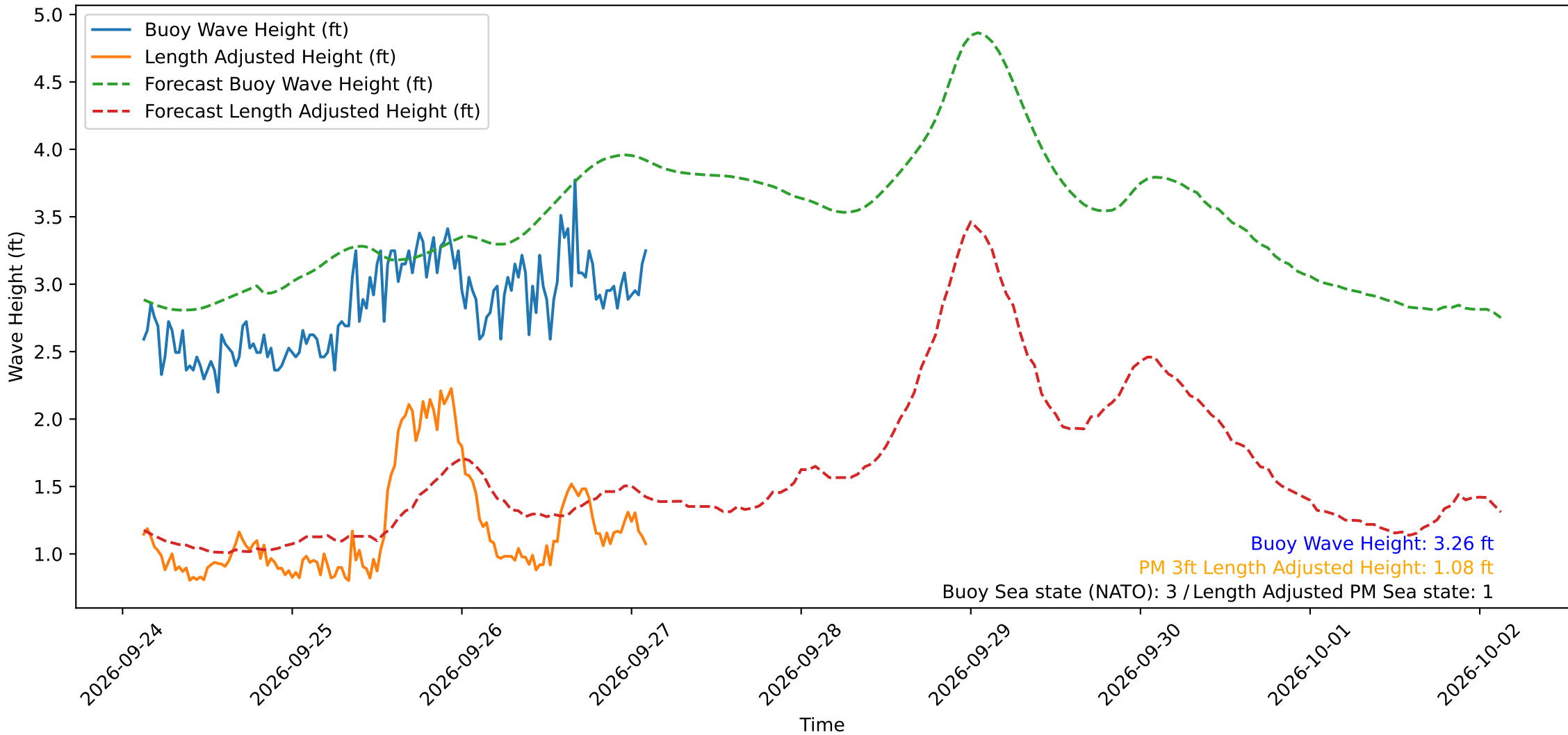
Wave Heights over Time for Oceanside Harbor at 2026-09-27 03:00:29
