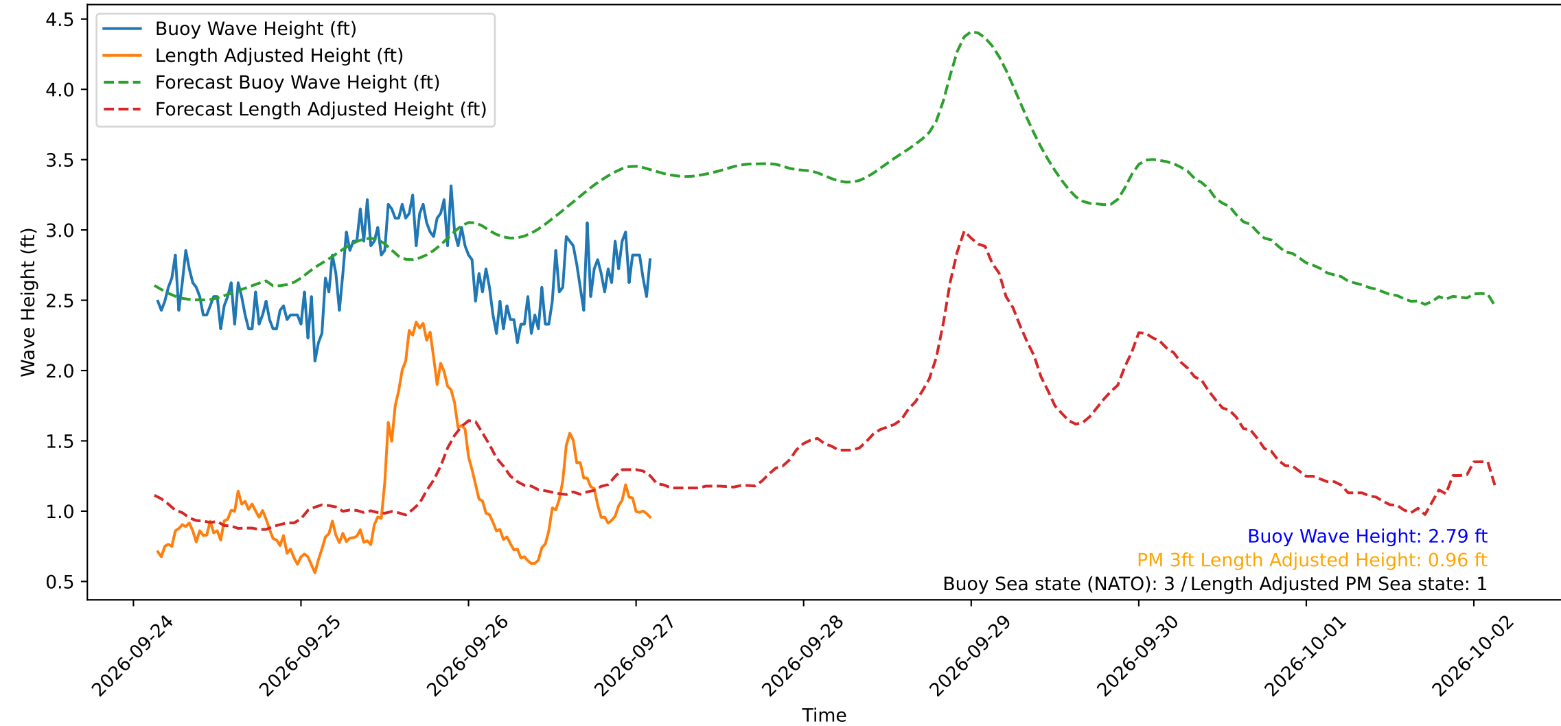
Wave Heights over Time for Red Beach at 2026-09-27 03:00:50
