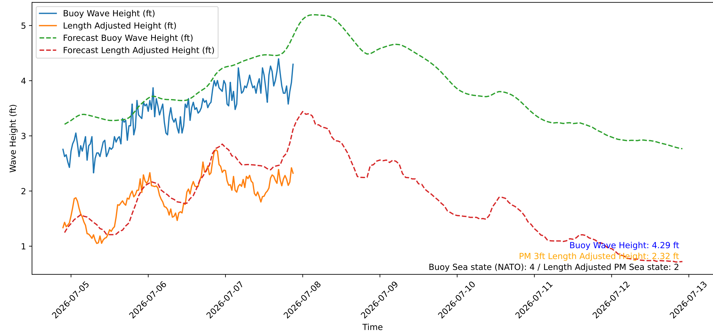
Wave Heights over Time for Oceanside Harbor at 2026-07-07 21:30:27
