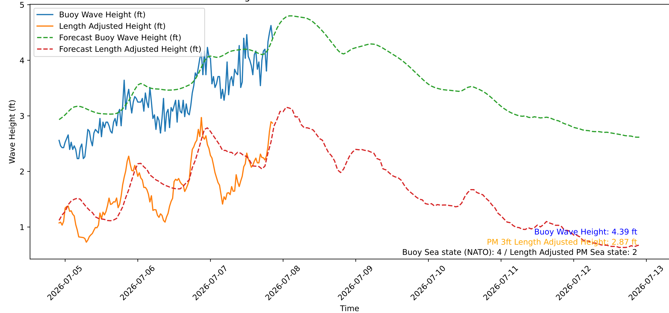
Wave Heights over Time for Red Beach at 2026-07-07 21:30:46
