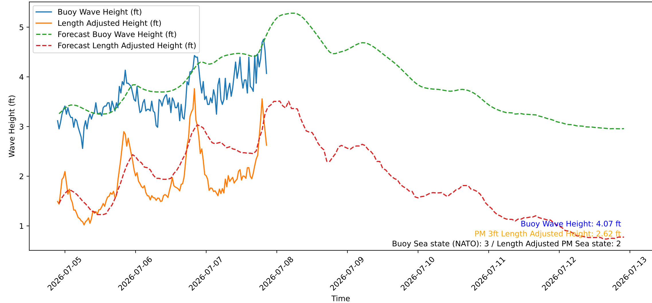
Wave Heights over Time for Green Beach at 2026-07-07 21:31:08
