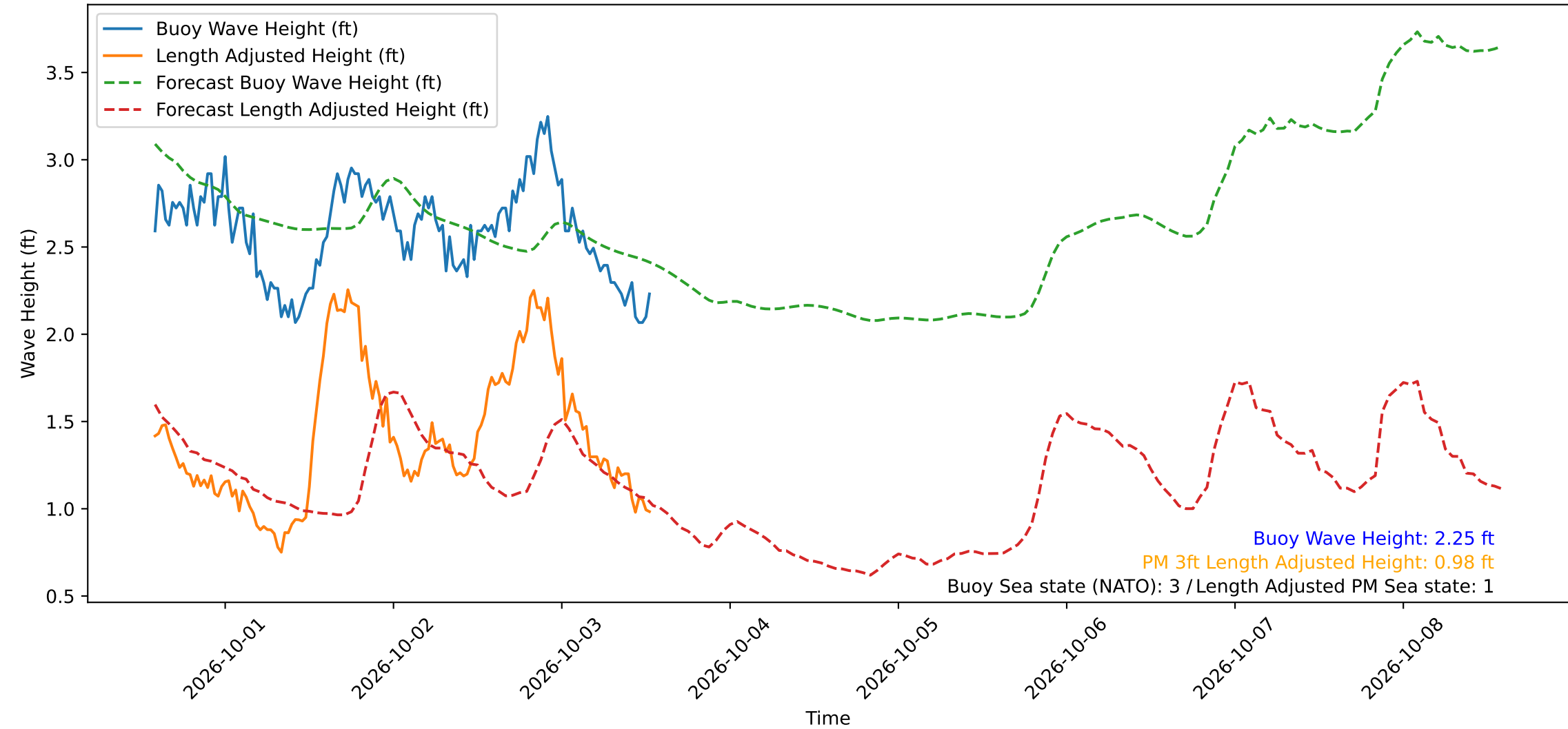
Wave Heights over Time for Red Beach at 2026-10-03 13:30:49
