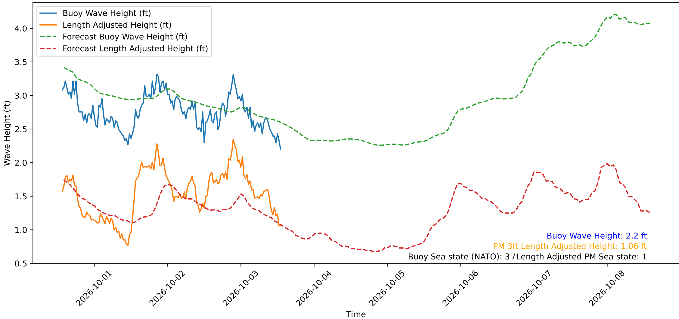
Wave Heights over Time for Oceanside Harbor at 2026-10-03 13:30:29
