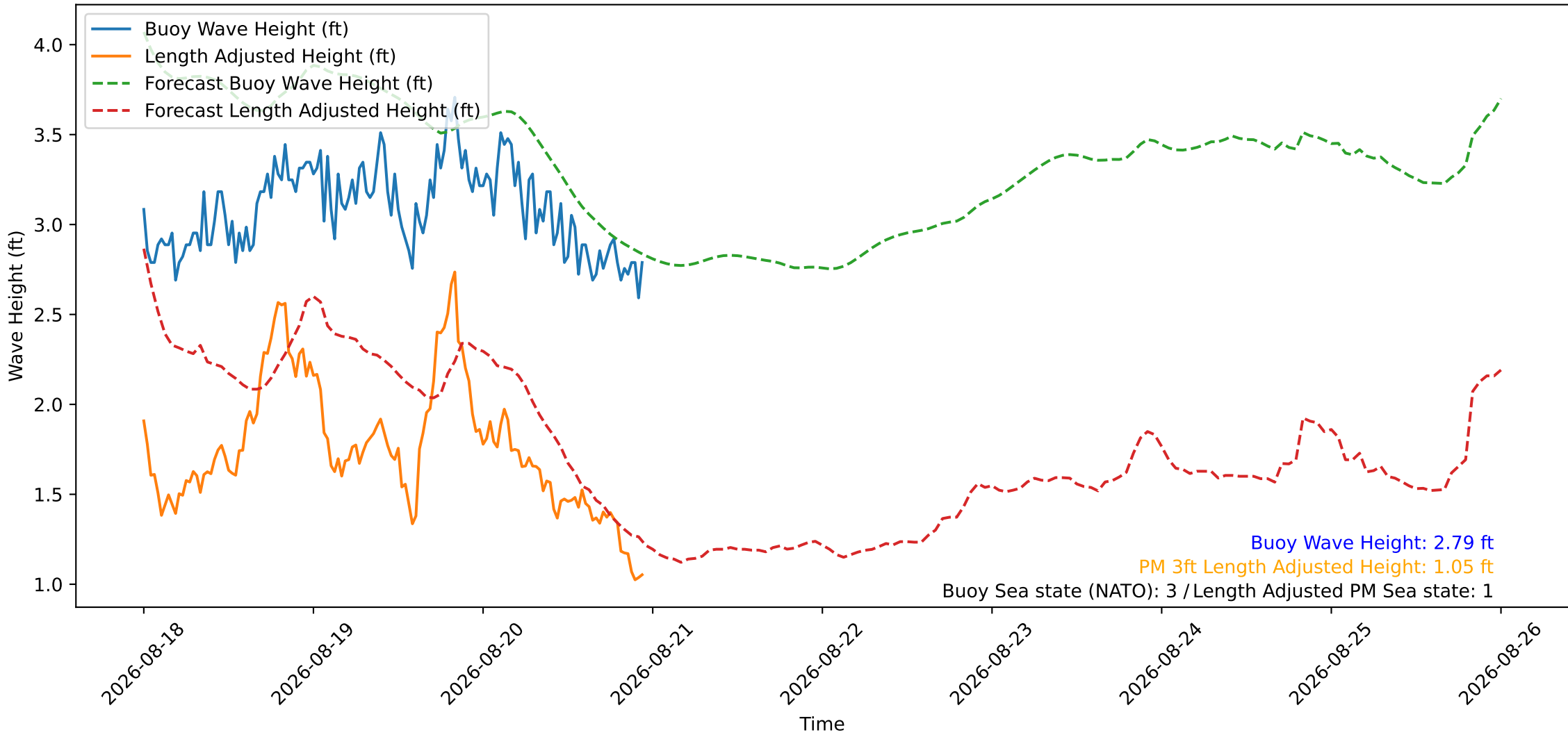
Wave Heights over Time for Green Beach at 2026-08-20 23:31:09
