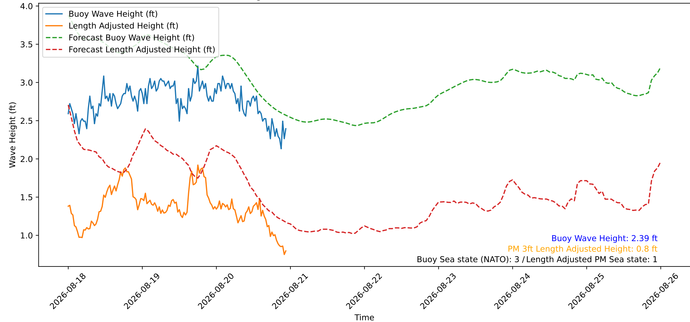
Wave Heights over Time for Red Beach at 2026-08-20 23:30:46
