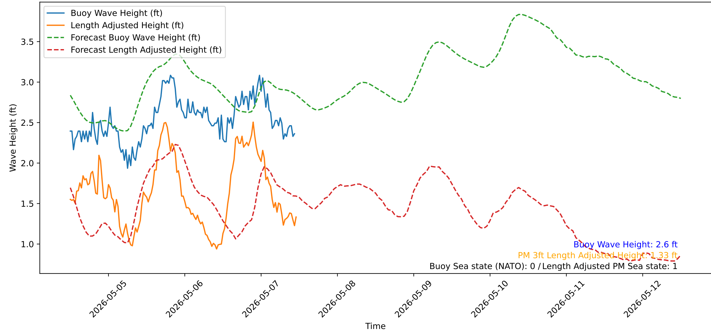
Wave Heights over Time for Red Beach at 2026-05-07 11:50:52
