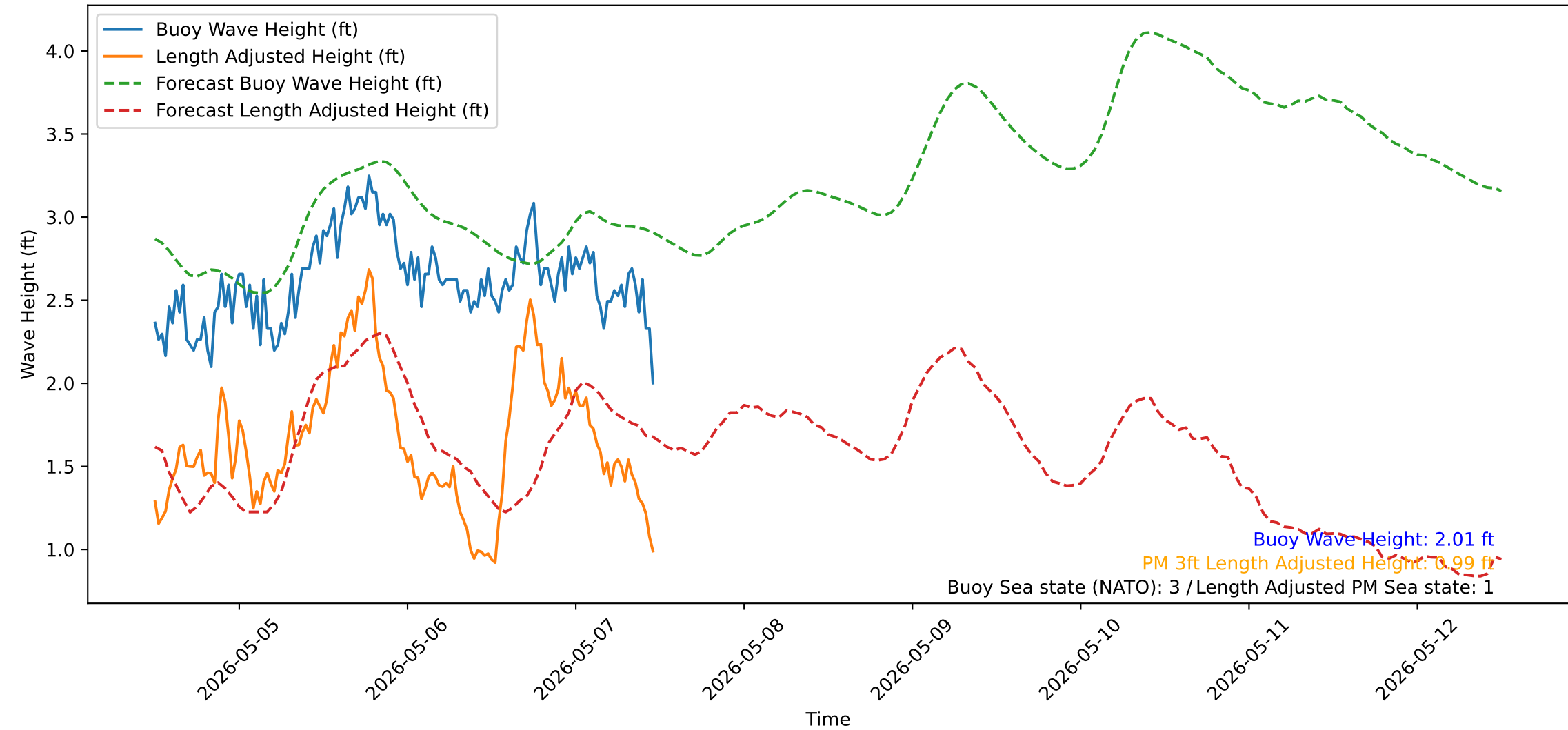
Wave Heights over Time for Oceanside Harbor at 2026-05-07 11:50:31
