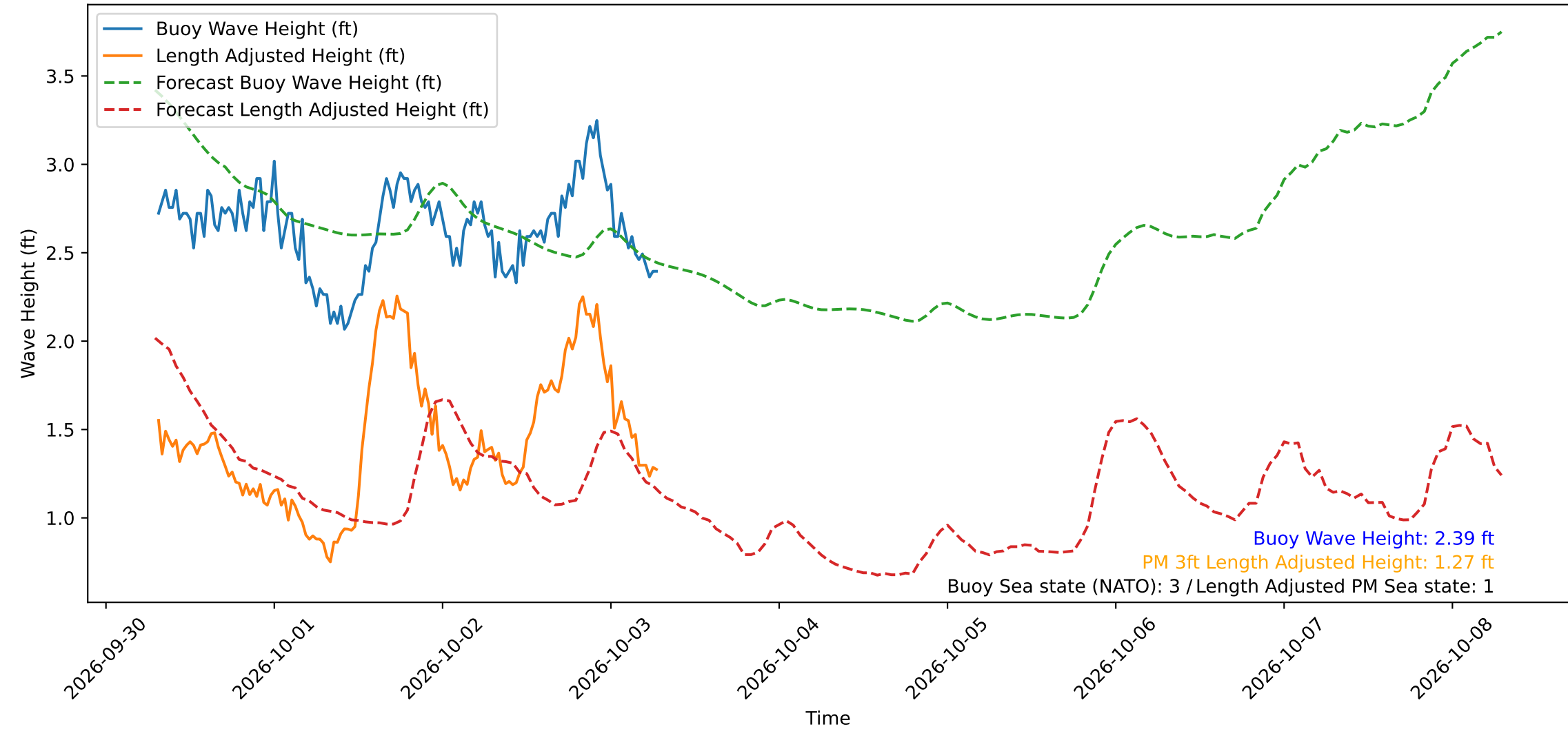
Wave Heights over Time for Red Beach at 2026-10-03 07:20:50
