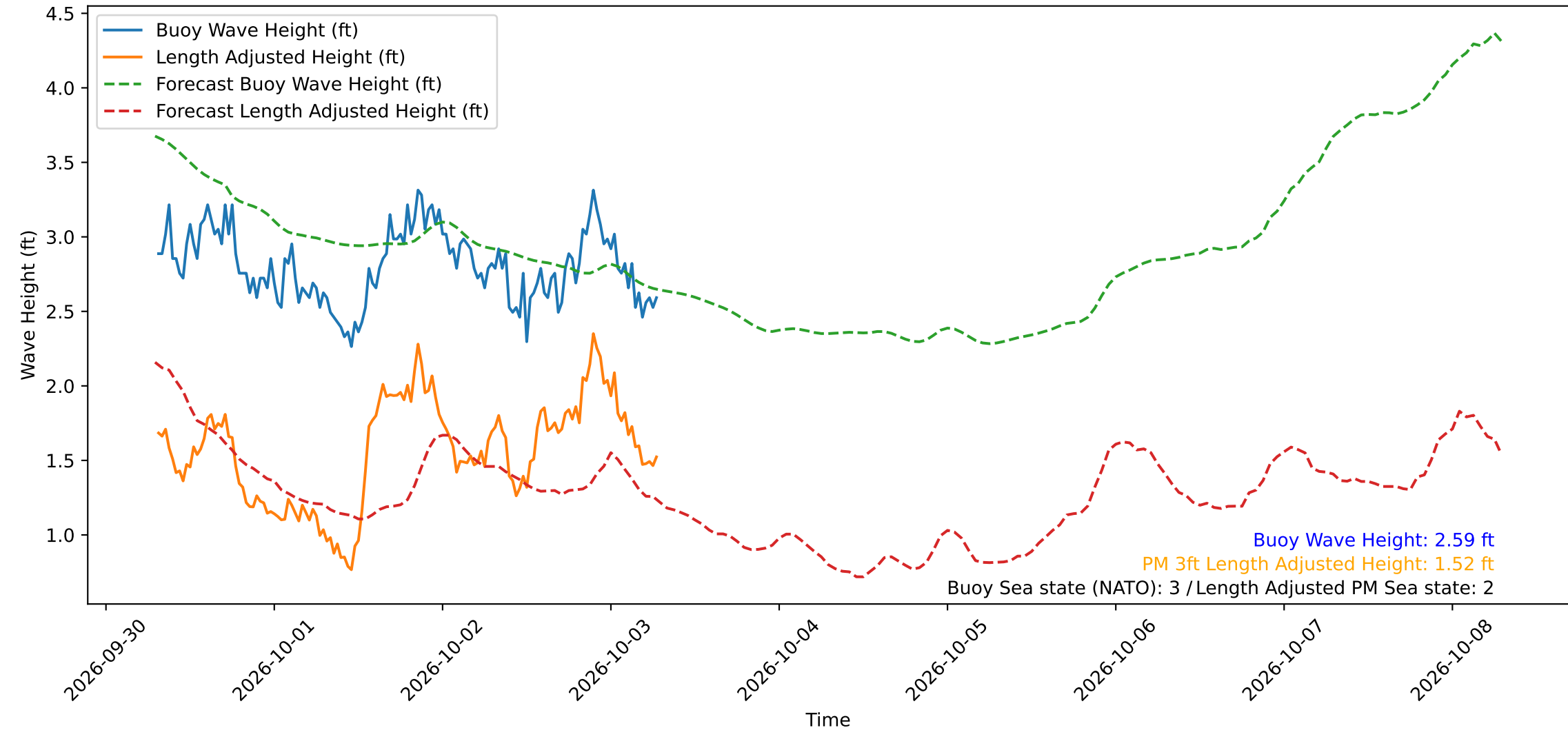
Wave Heights over Time for Oceanside Harbor at 2026-10-03 07:20:29
