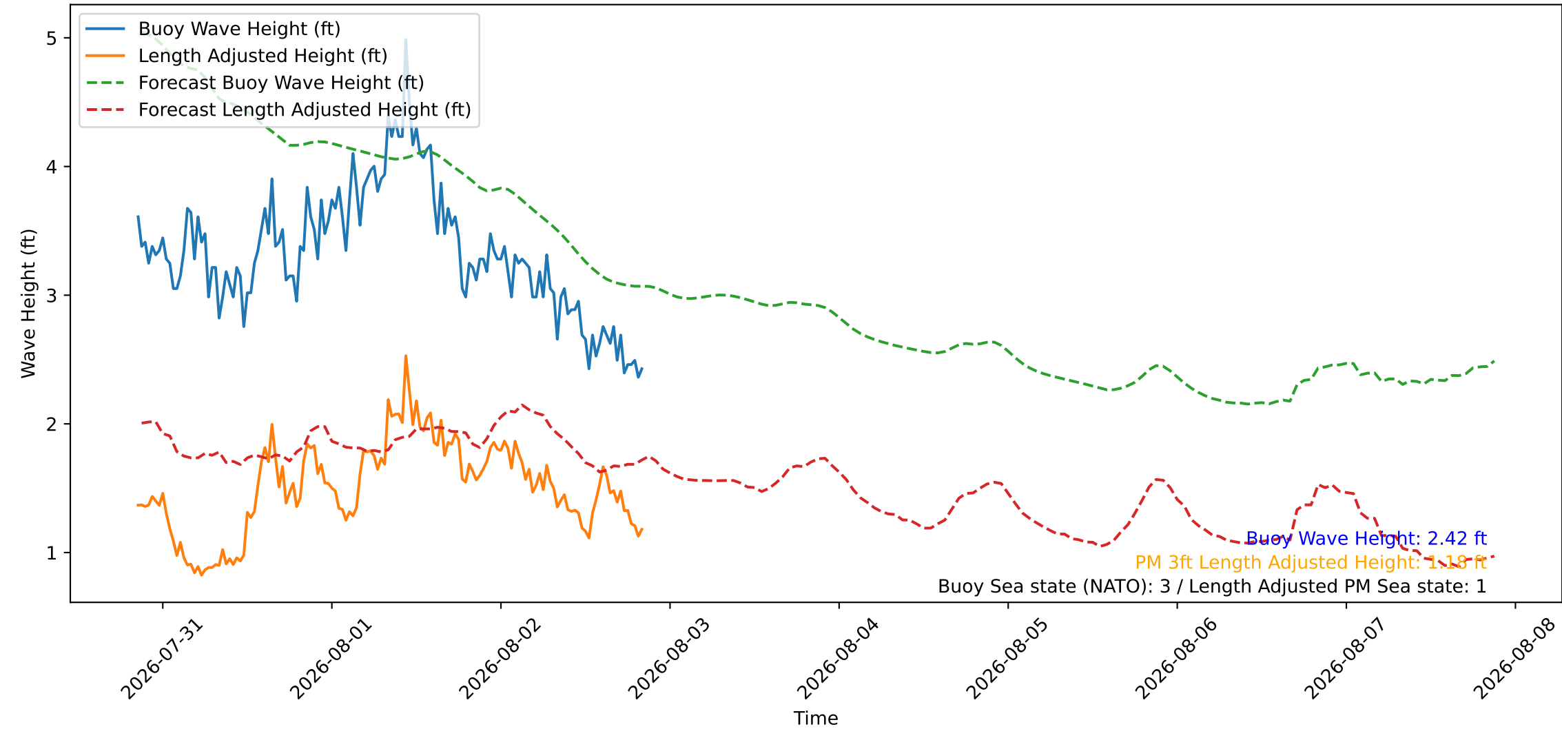
Wave Heights over Time for Green Beach at 2026-08-02 20:41:08
