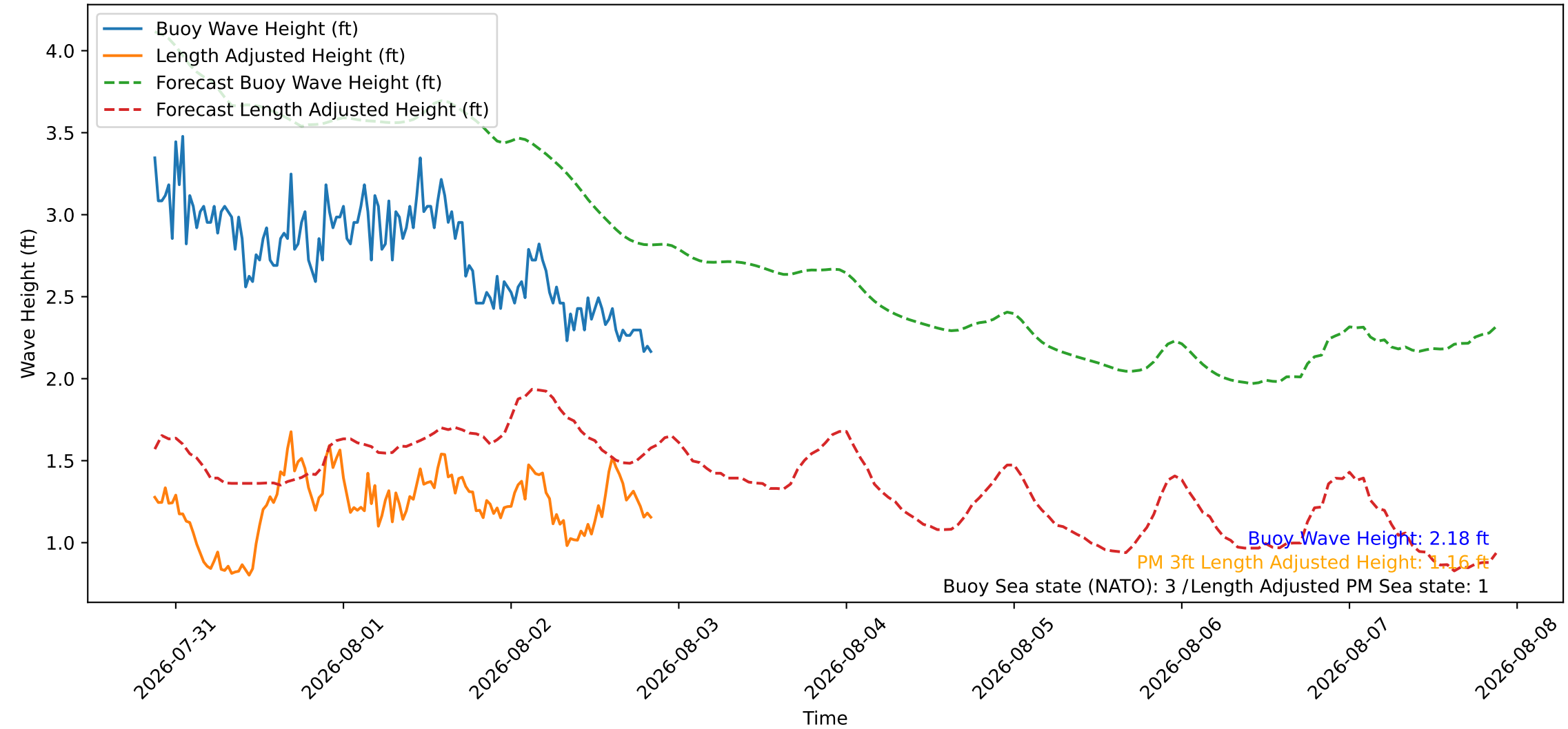
Wave Heights over Time for Red Beach at 2026-08-02 20:40:46
