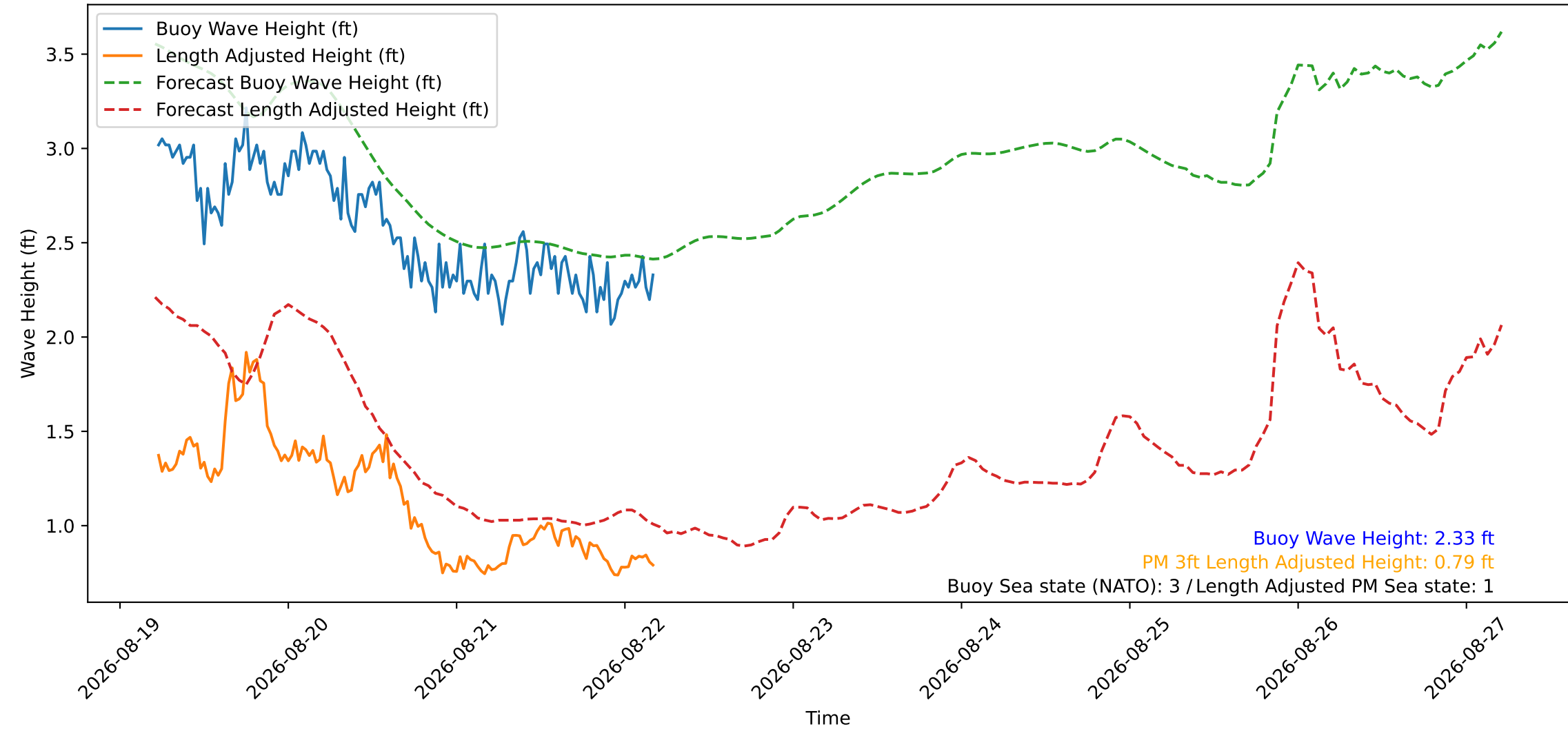
Wave Heights over Time for Red Beach at 2026-08-22 05:00:50
