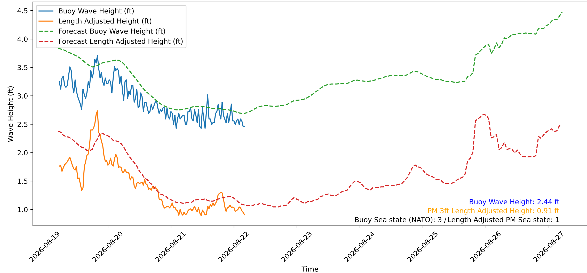
Wave Heights over Time for Green Beach at 2026-08-22 05:01:12
