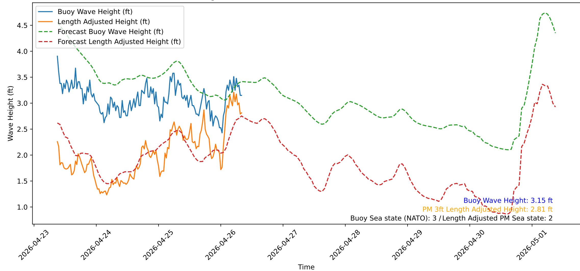
Wave Heights over Time for Green Beach at 2026-04-26 09:01:12
