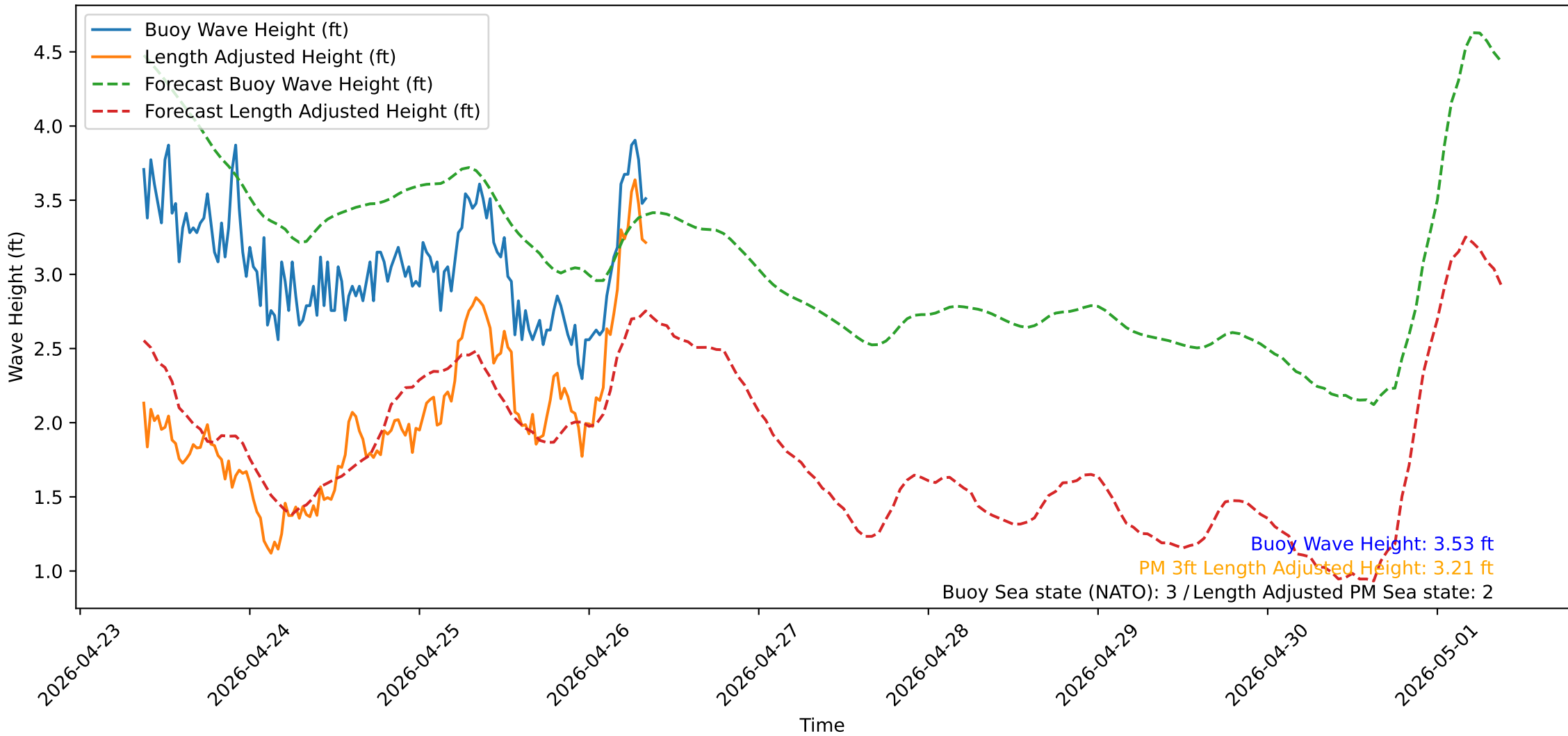
Wave Heights over Time for Oceanside Harbor at 2026-04-26 09:00:31
