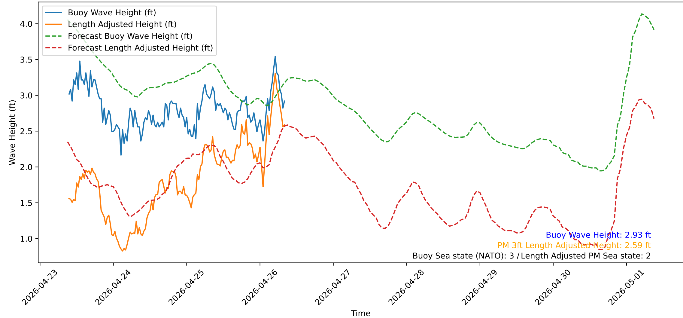
Wave Heights over Time for Red Beach at 2026-04-26 09:00:50
