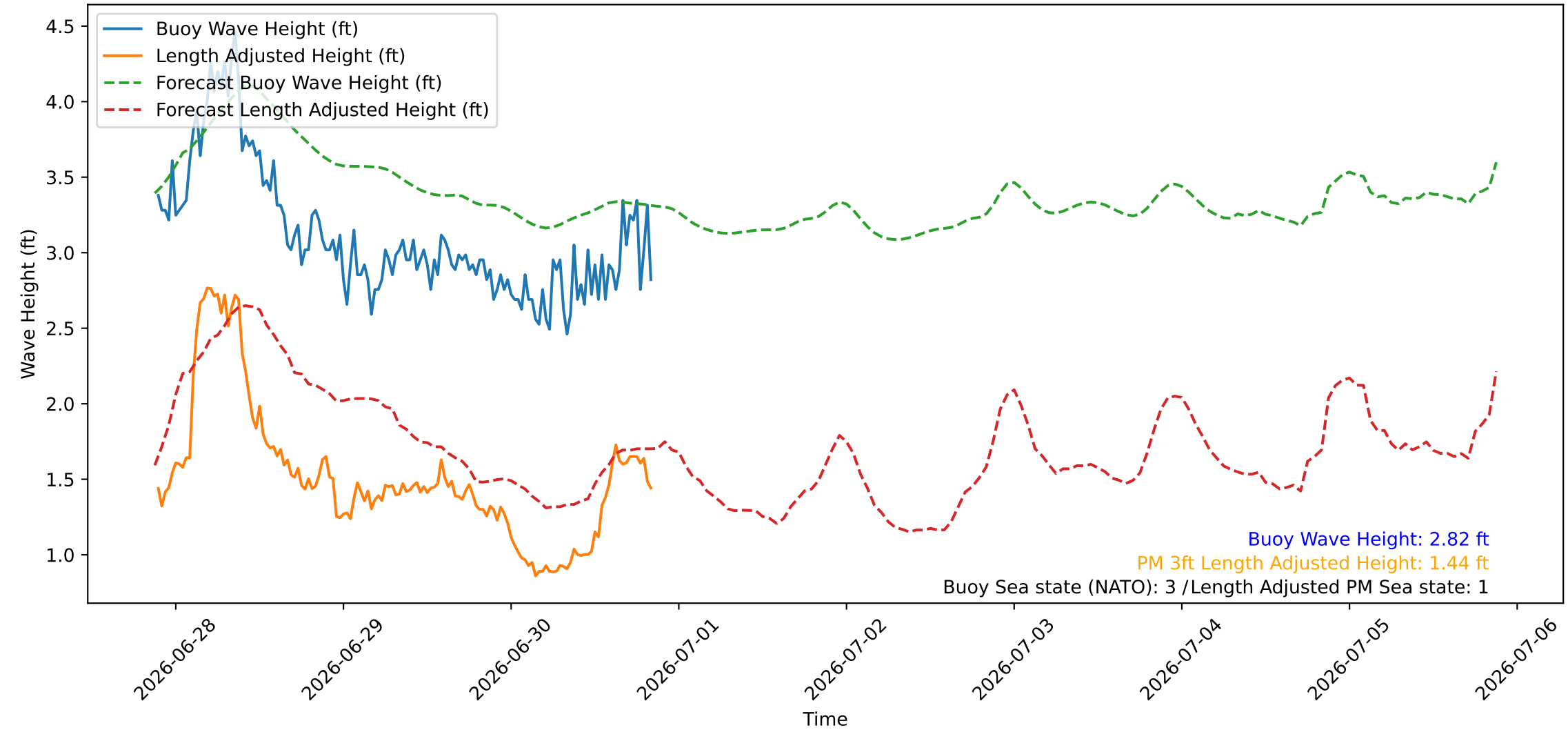
Wave Heights over Time for Red Beach at 2026-06-30 21:00:45
