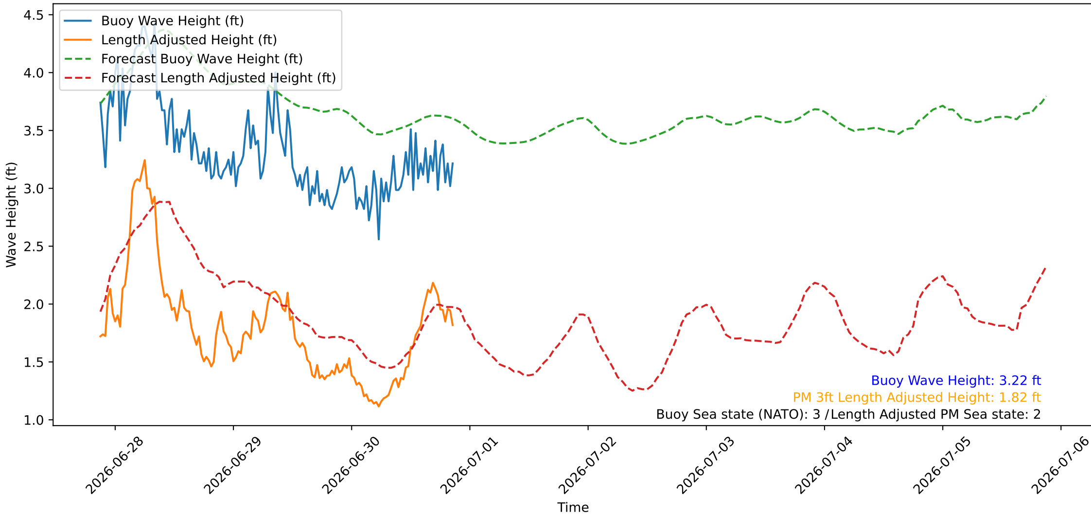
Wave Heights over Time for Oceanside Harbor at 2026-06-30 21:00:26
