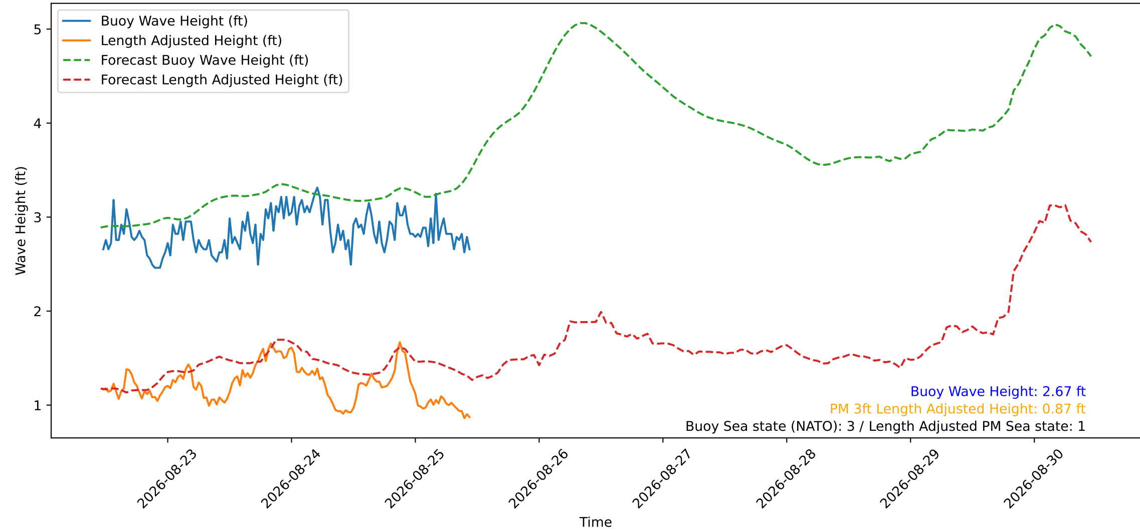
Wave Heights over Time for Green Beach at 2026-08-25 11:21:16
