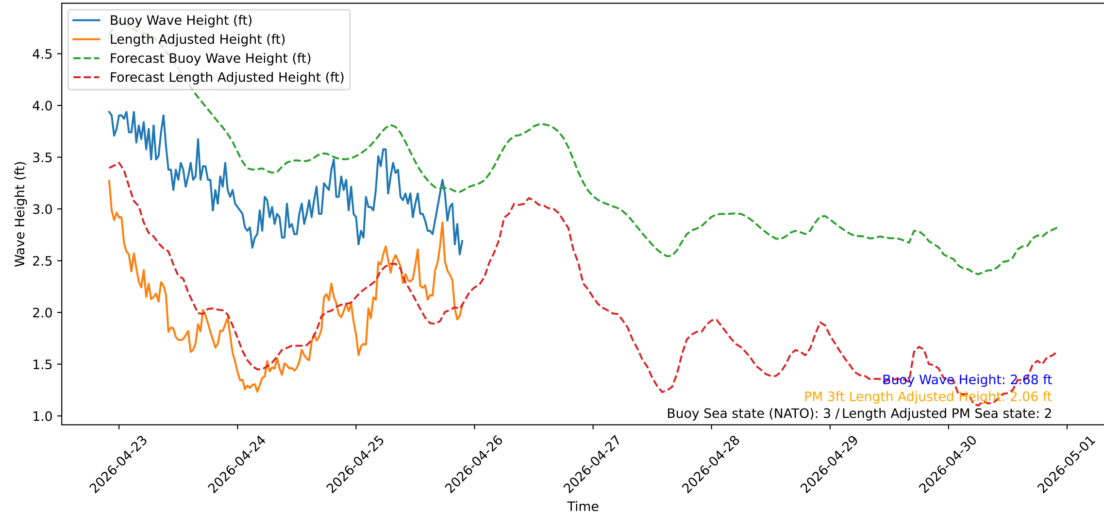
Wave Heights over Time for Green Beach at 2026-04-25 22:11:12
