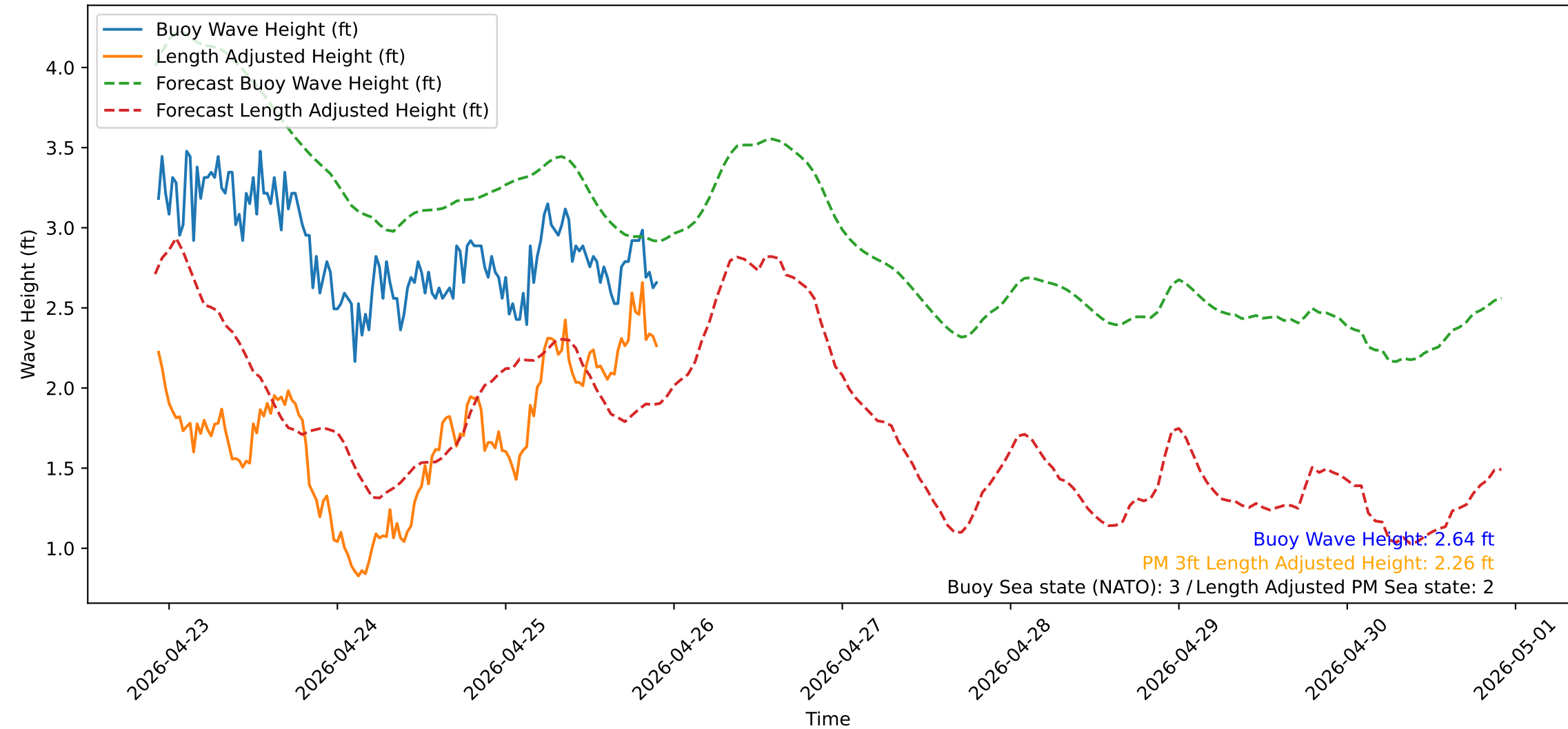
Wave Heights over Time for Red Beach at 2026-04-25 22:10:50
