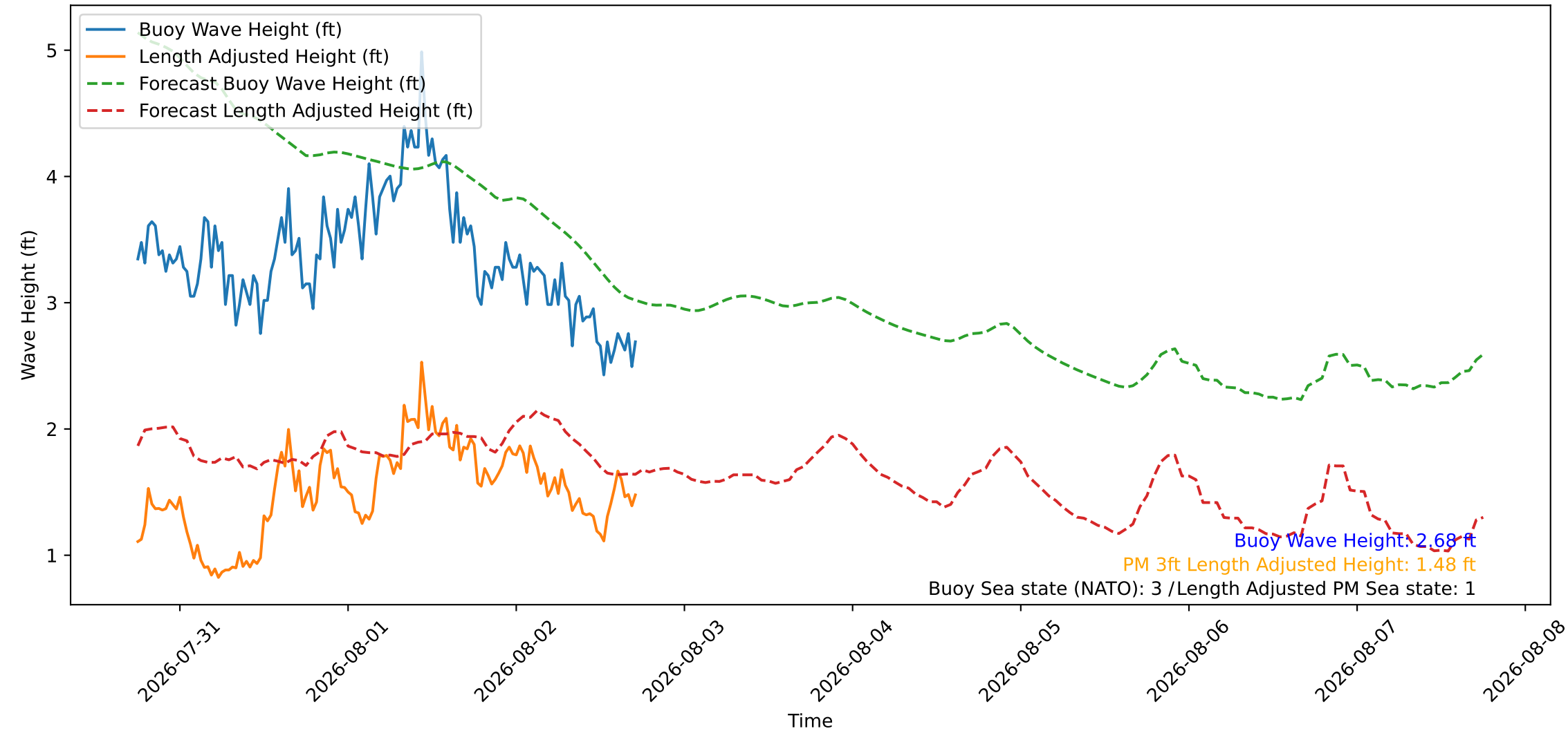
Wave Heights over Time for Green Beach at 2026-08-02 18:01:08
