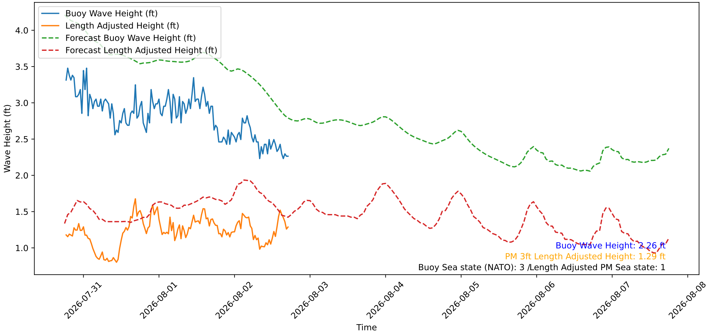
Wave Heights over Time for Red Beach at 2026-08-02 18:00:45
