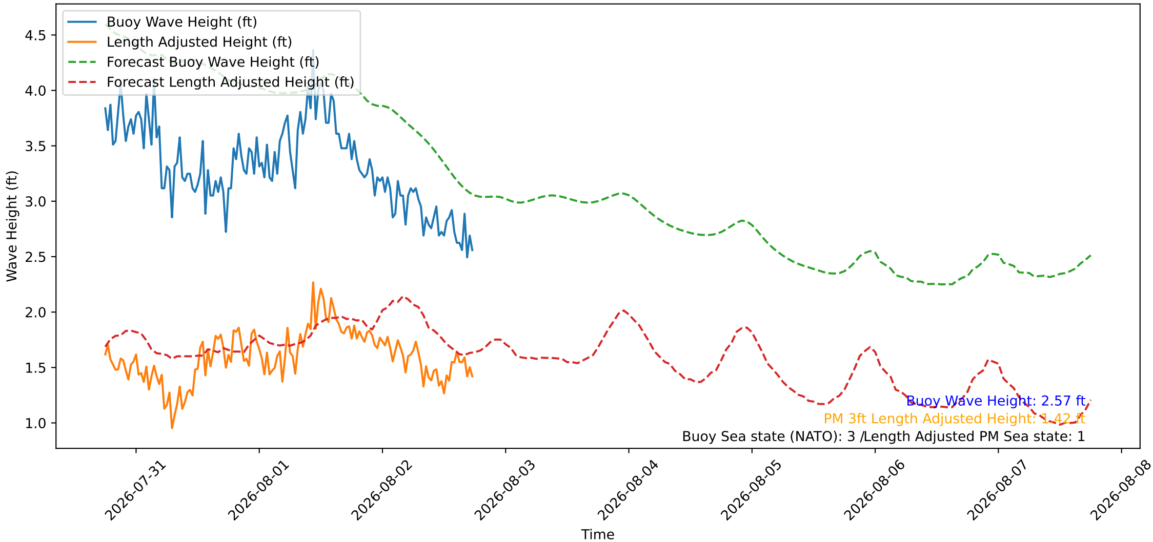
Wave Heights over Time for Oceanside Harbor at 2026-08-02 18:00:26
