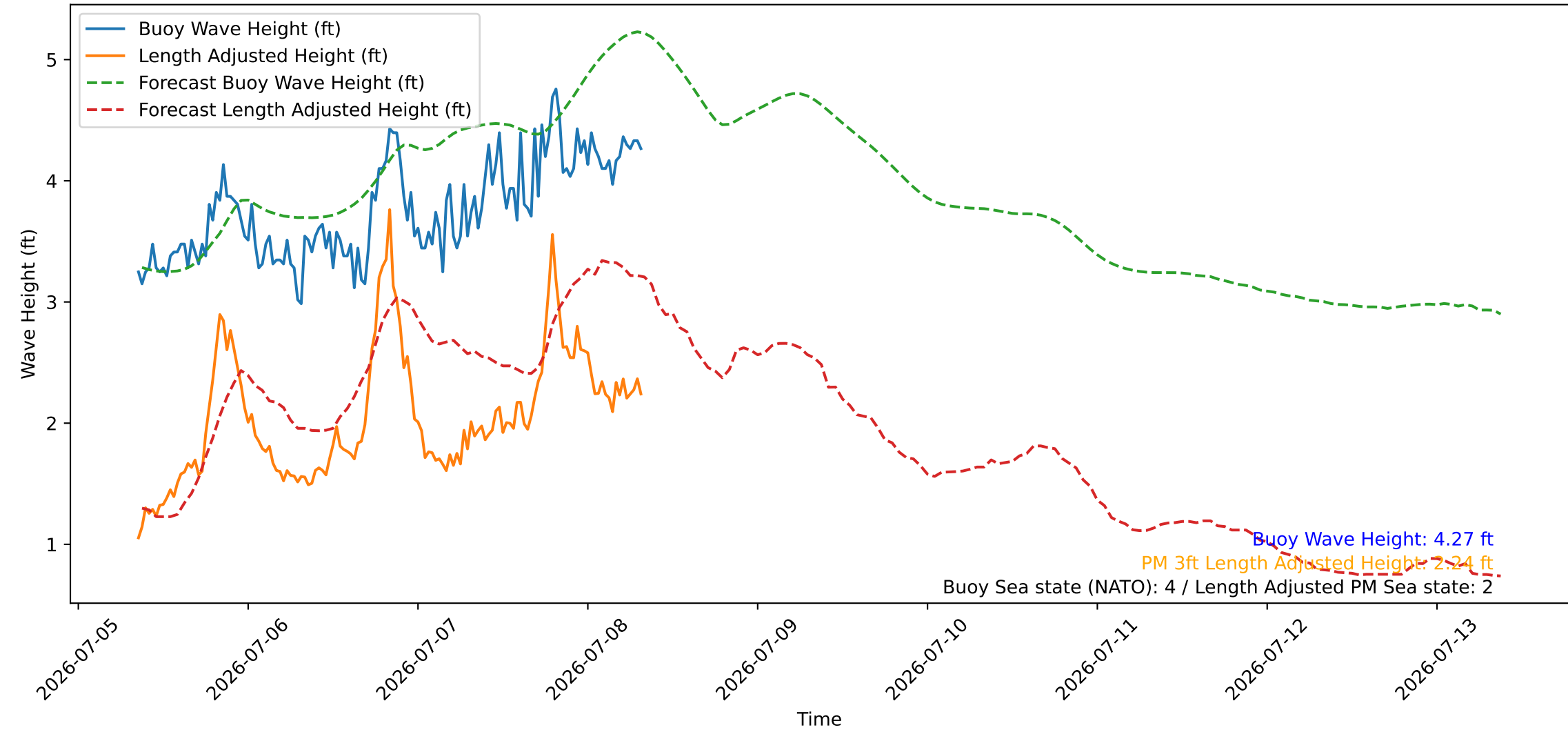
Wave Heights over Time for Green Beach at 2026-07-08 08:31:07
