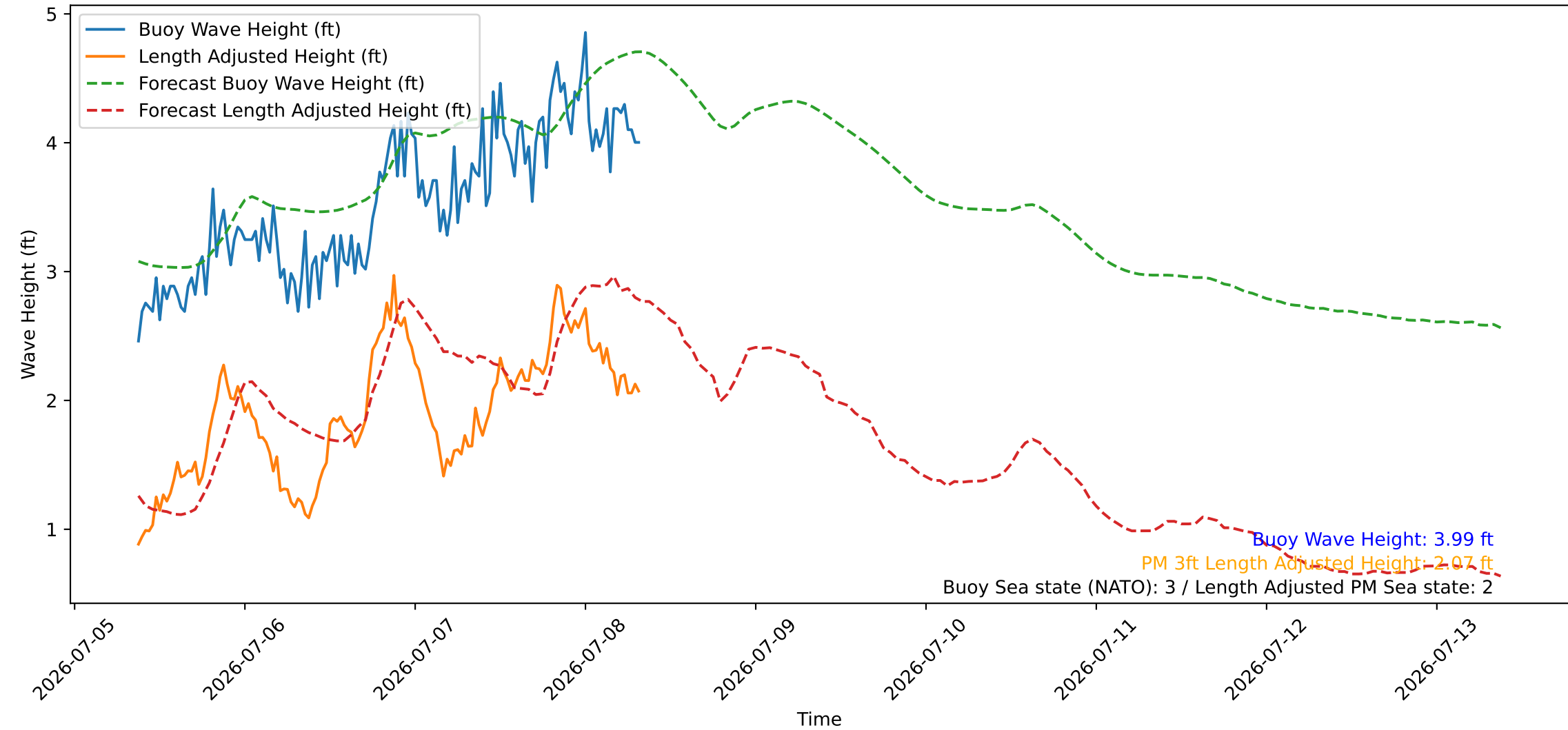
Wave Heights over Time for Red Beach at 2026-07-08 08:30:45
