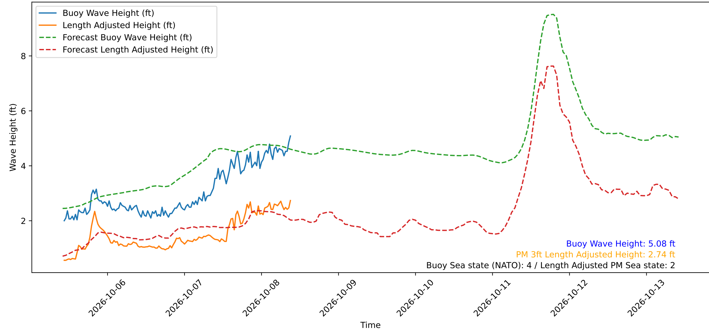
Wave Heights over Time for Green Beach at 2026-10-08 10:01:12
