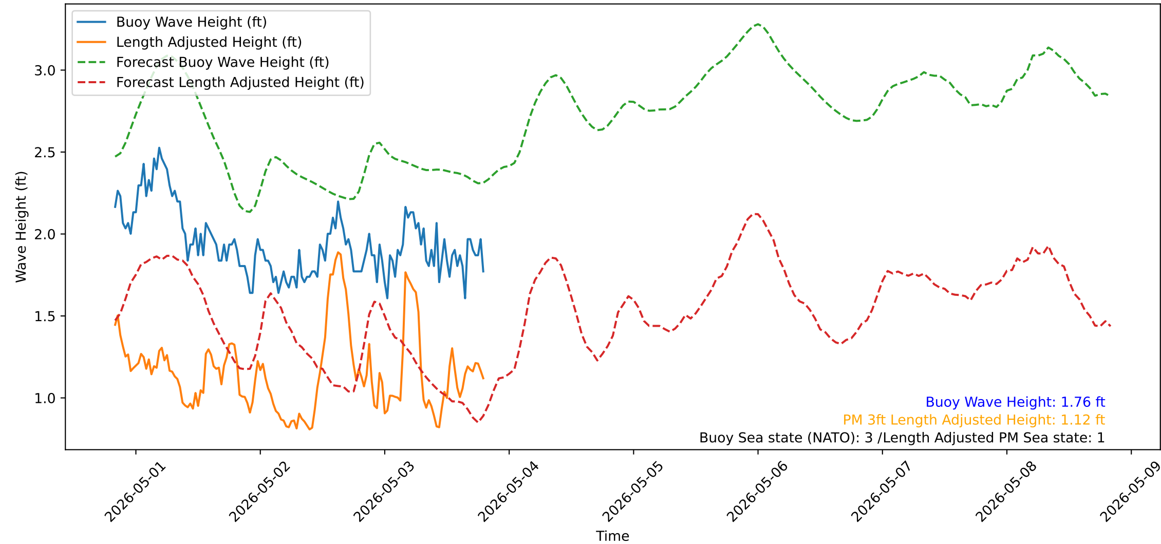
Wave Heights over Time for Red Beach at 2026-05-03 19:50:51
