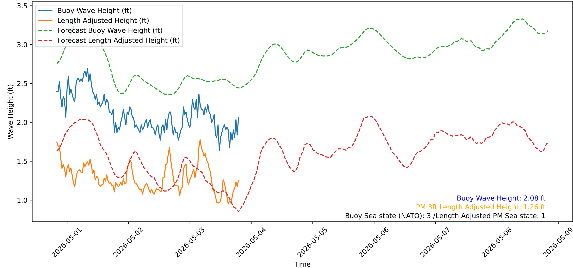
Wave Heights over Time for Oceanside Harbor at 2026-05-03 19:50:31
