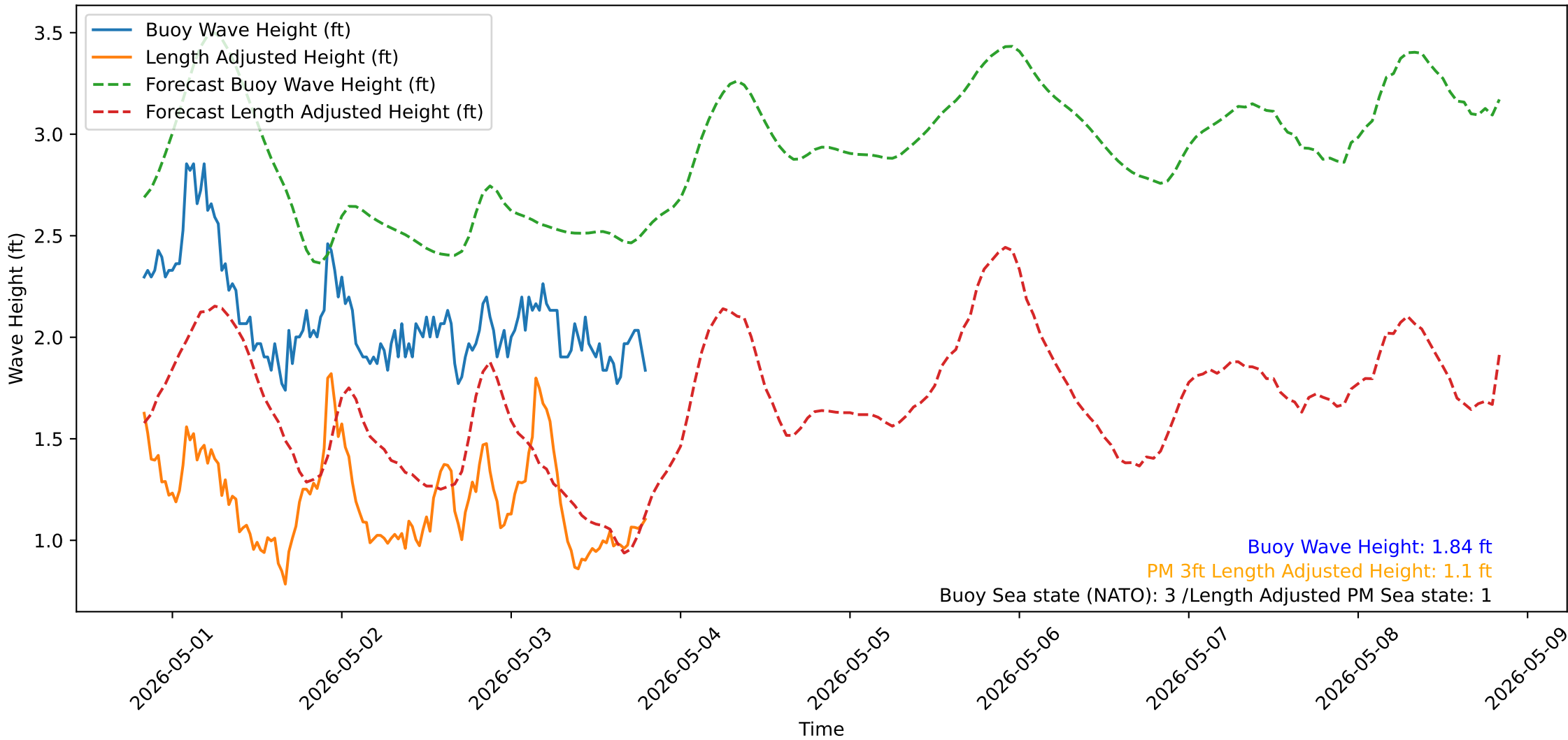
Wave Heights over Time for Green Beach at 2026-05-03 19:51:13
