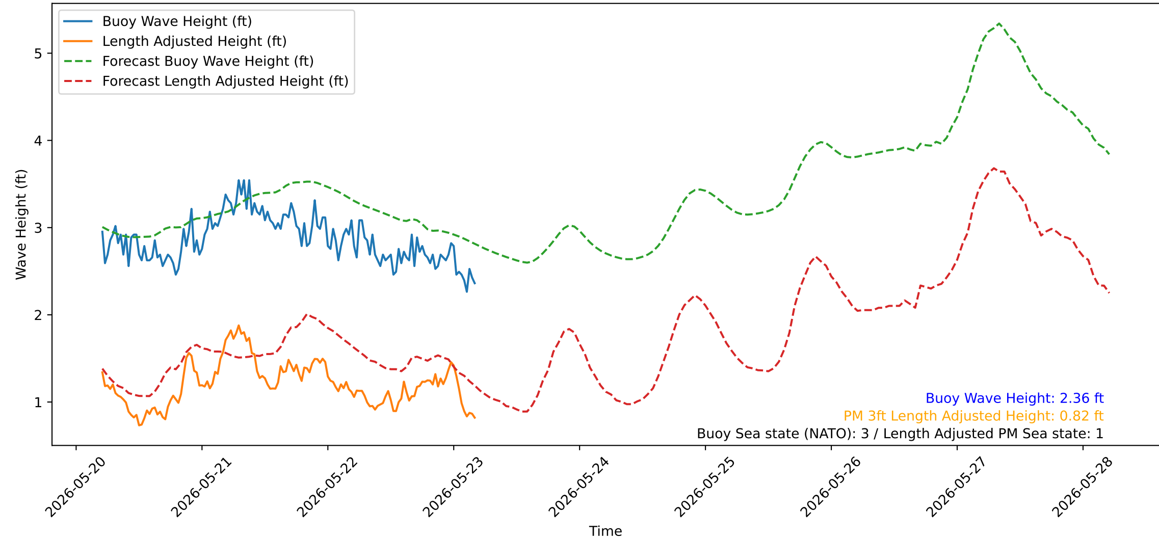
Wave Heights over Time for Green Beach at 2026-05-23 04:51:15
