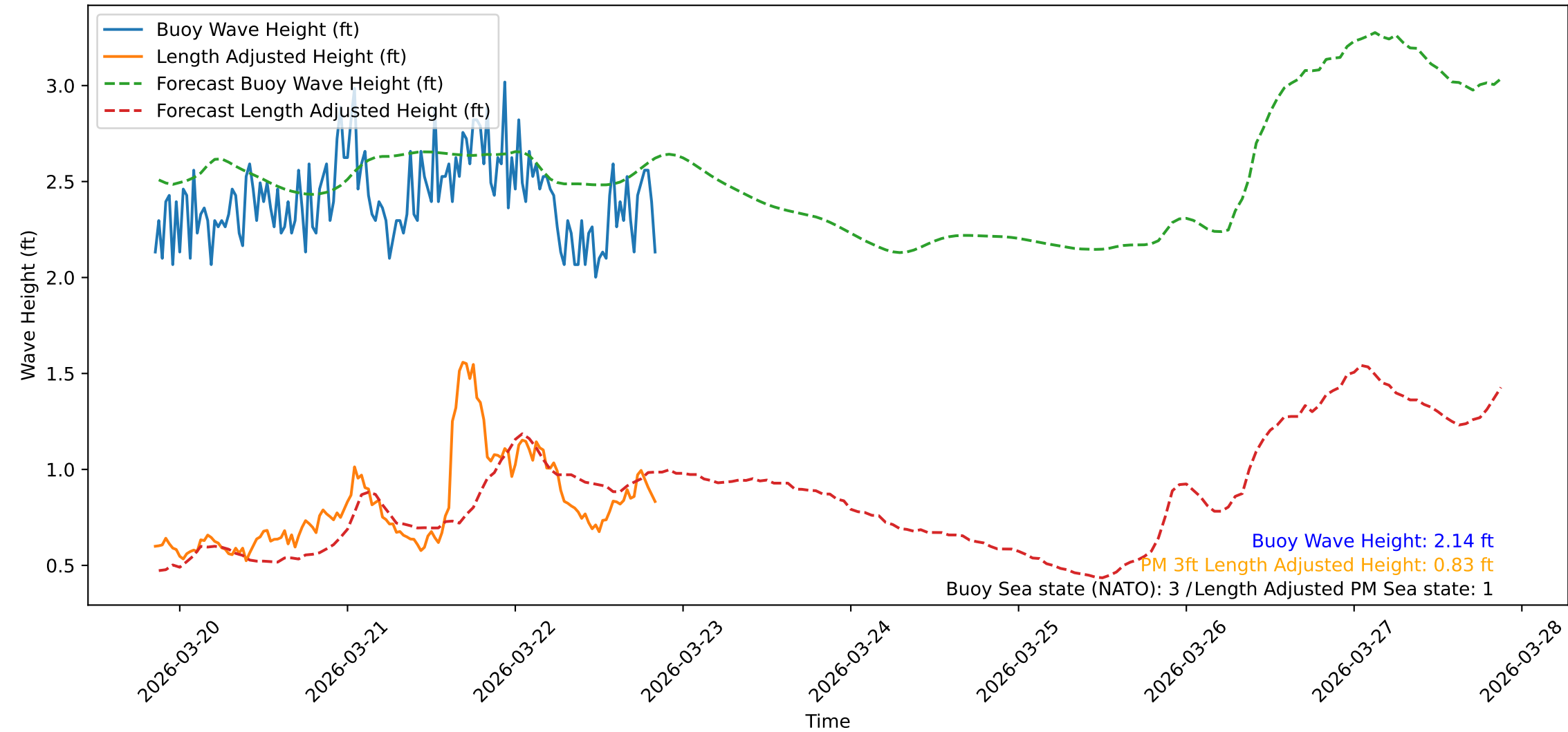
Wave Heights over Time for Oceanside Harbor at 2026-03-22 20:40:31
