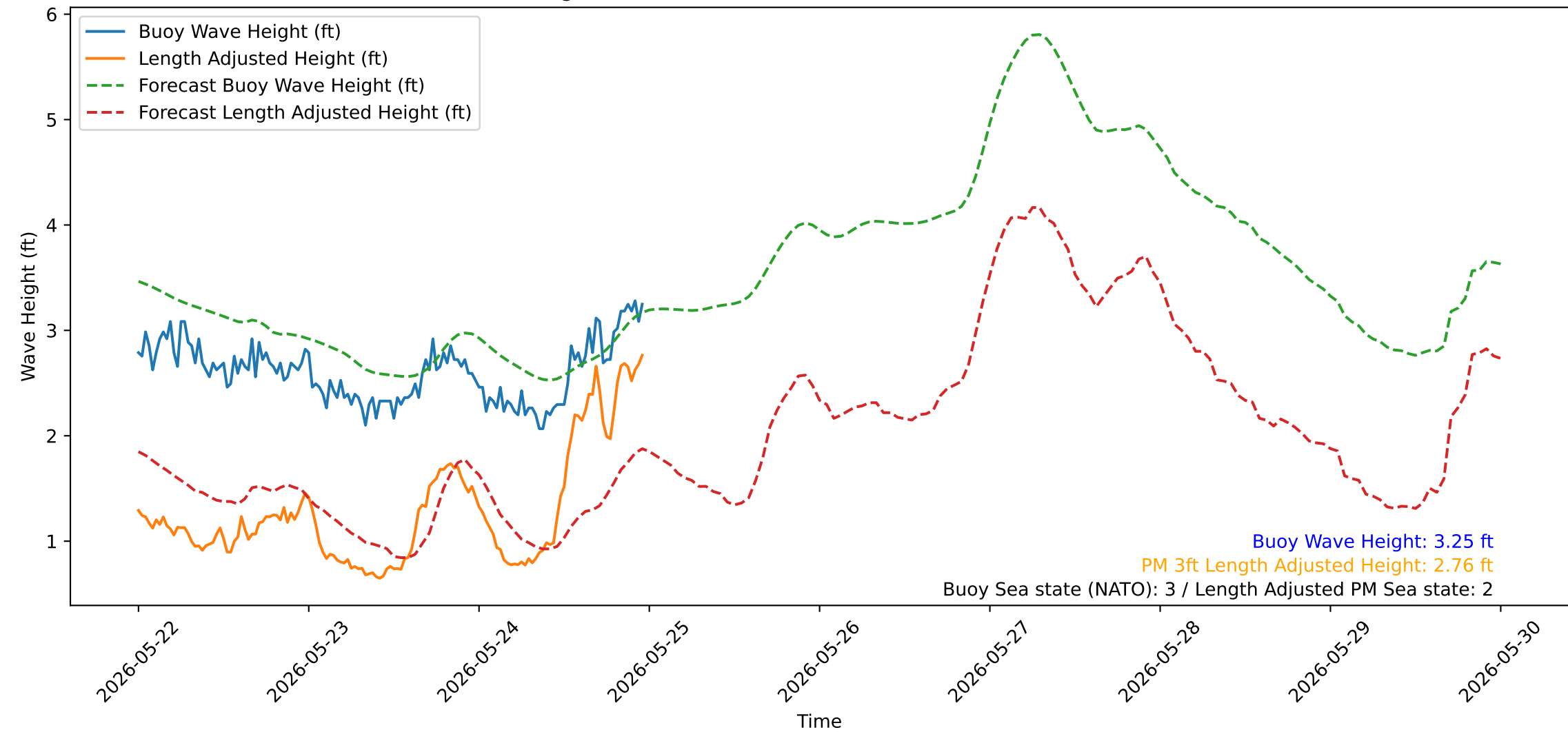
Wave Heights over Time for Green Beach at 2026-05-25 00:01:13
