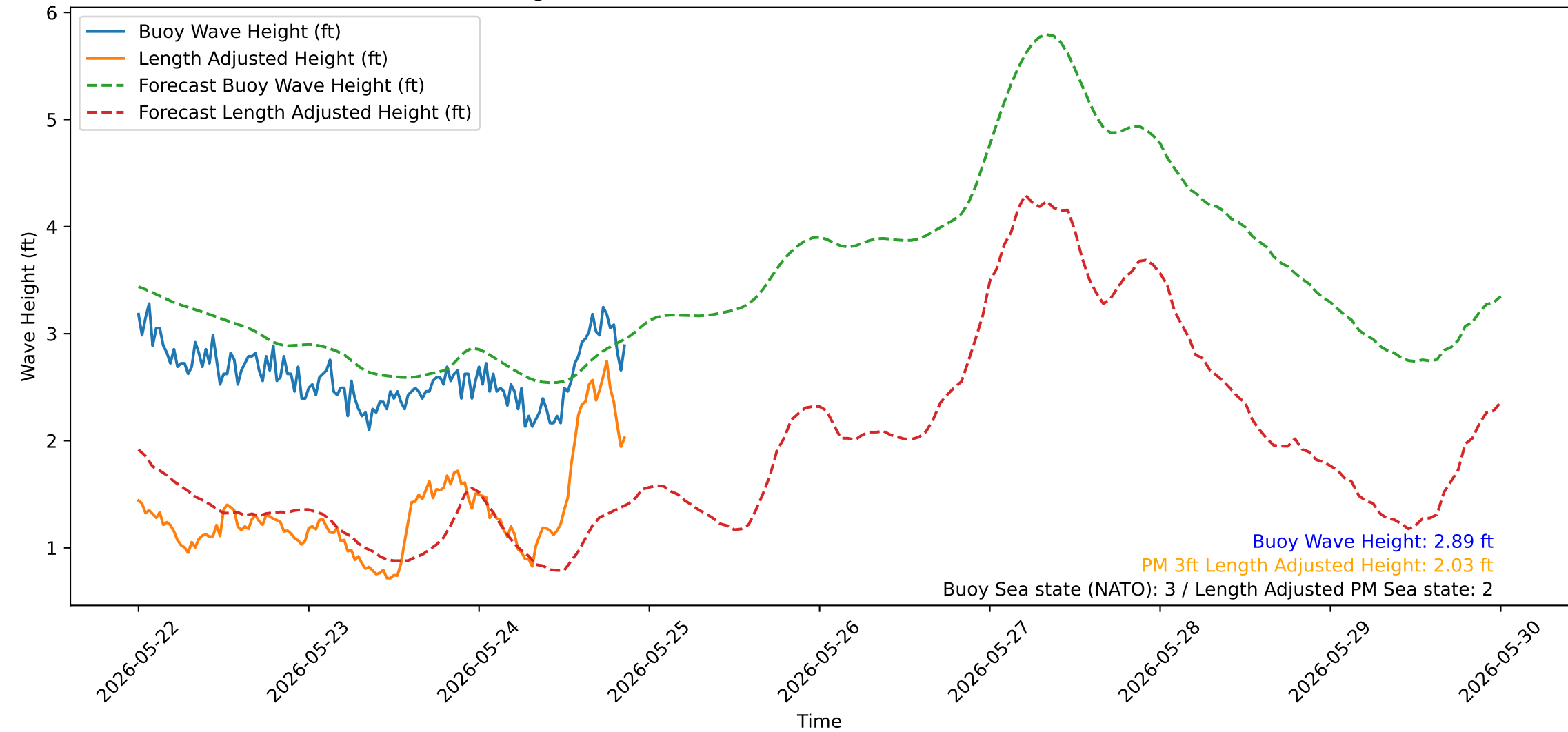
Wave Heights over Time for Oceanside Harbor at 2026-05-25 00:00:31
