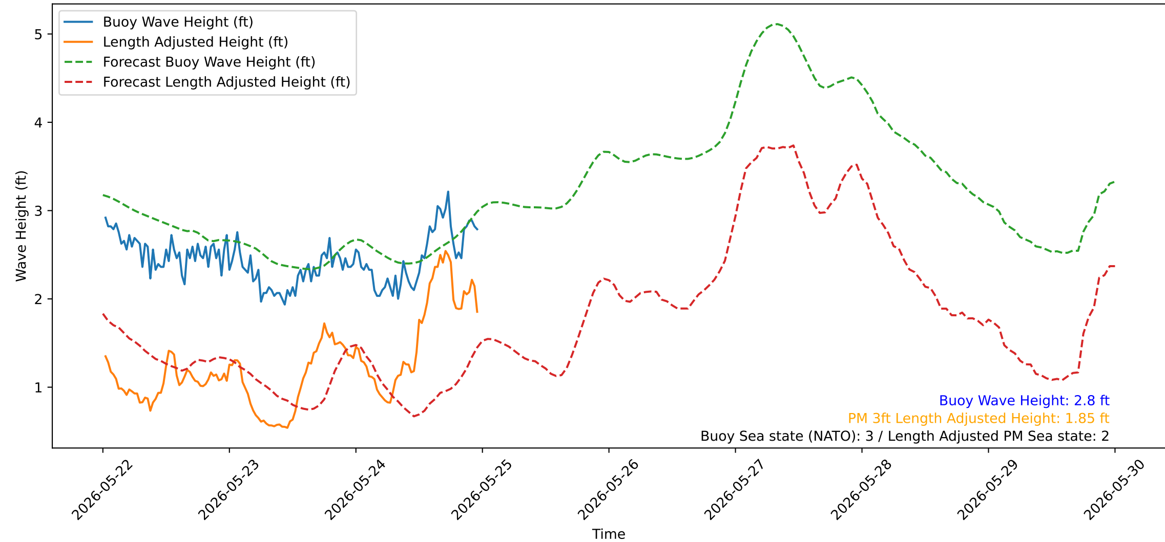
Wave Heights over Time for Red Beach at 2026-05-25 00:00:51
