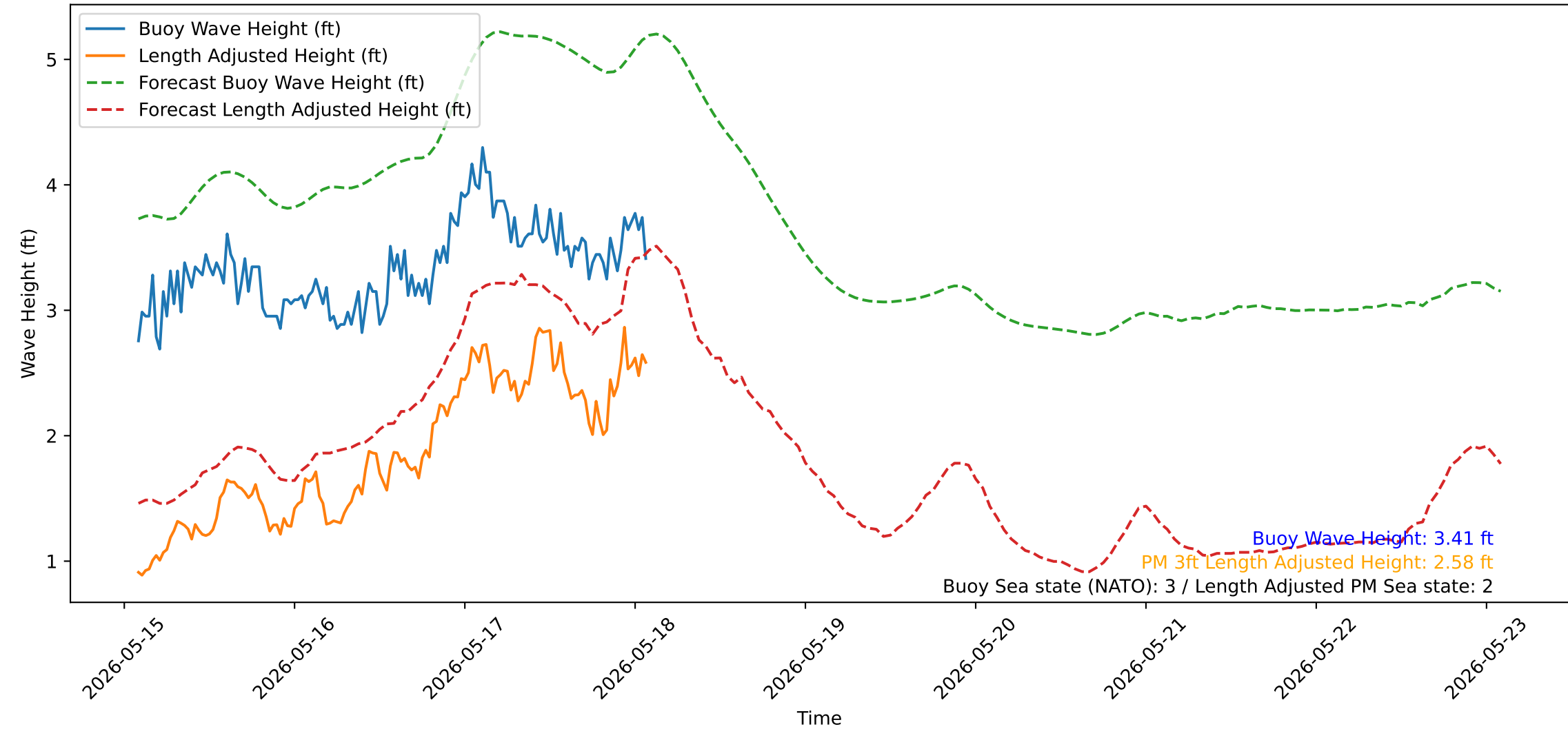
Wave Heights over Time for Oceanside Harbor at 2026-05-18 02:00:32
