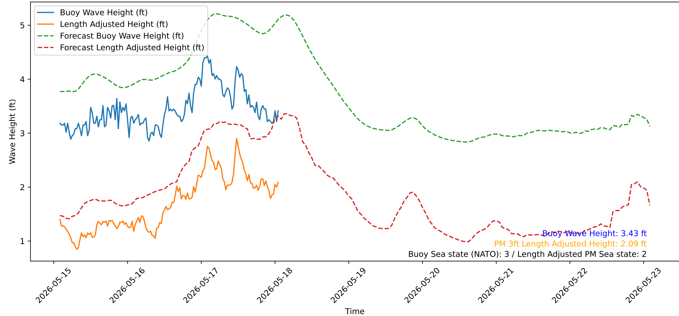
Wave Heights over Time for Green Beach at 2026-05-18 02:01:14
