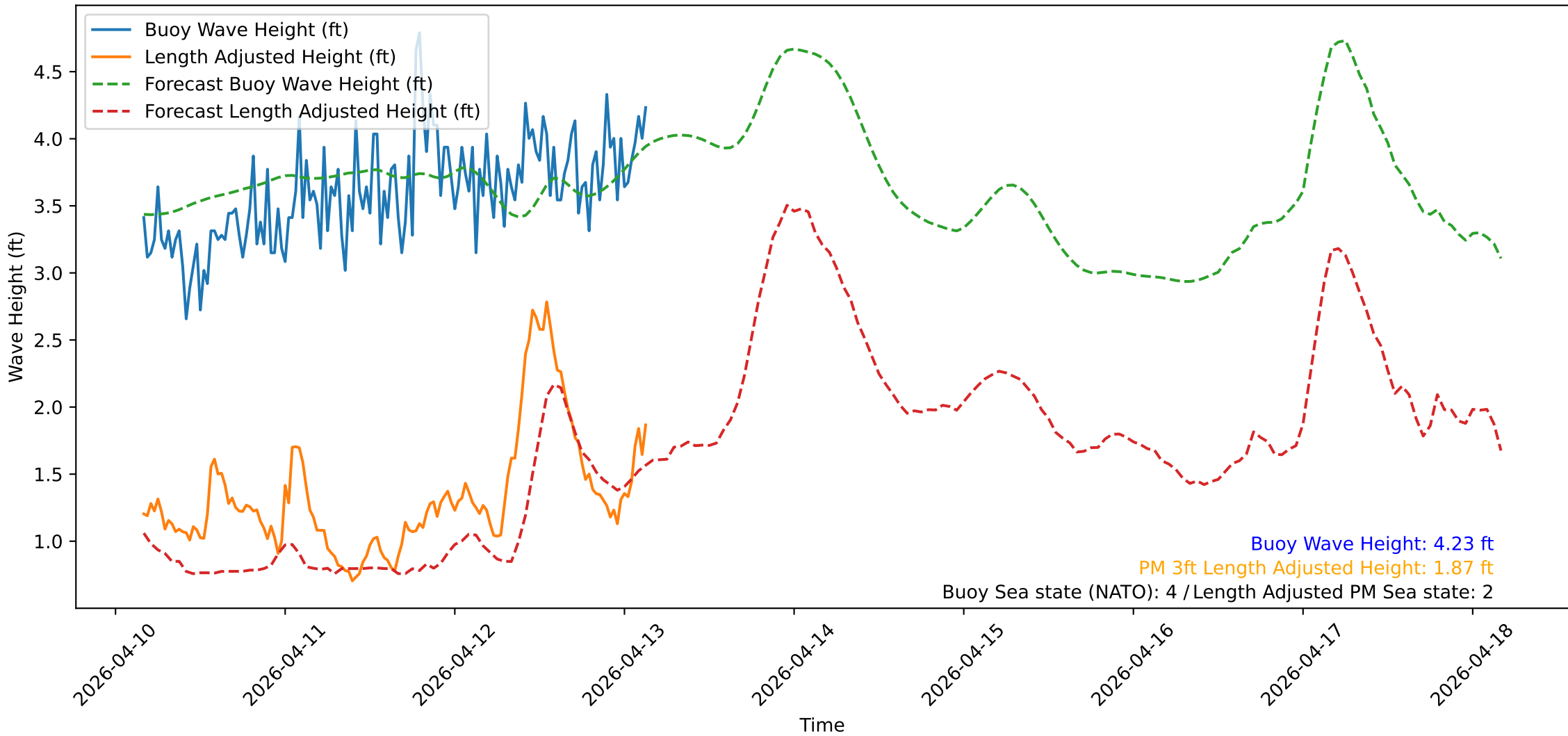
Wave Heights over Time for Oceanside Harbor at 2026-04-13 03:50:31
