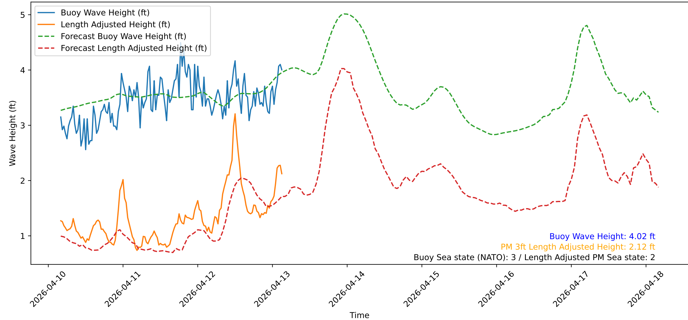
Wave Heights over Time for Green Beach at 2026-04-13 03:51:13
