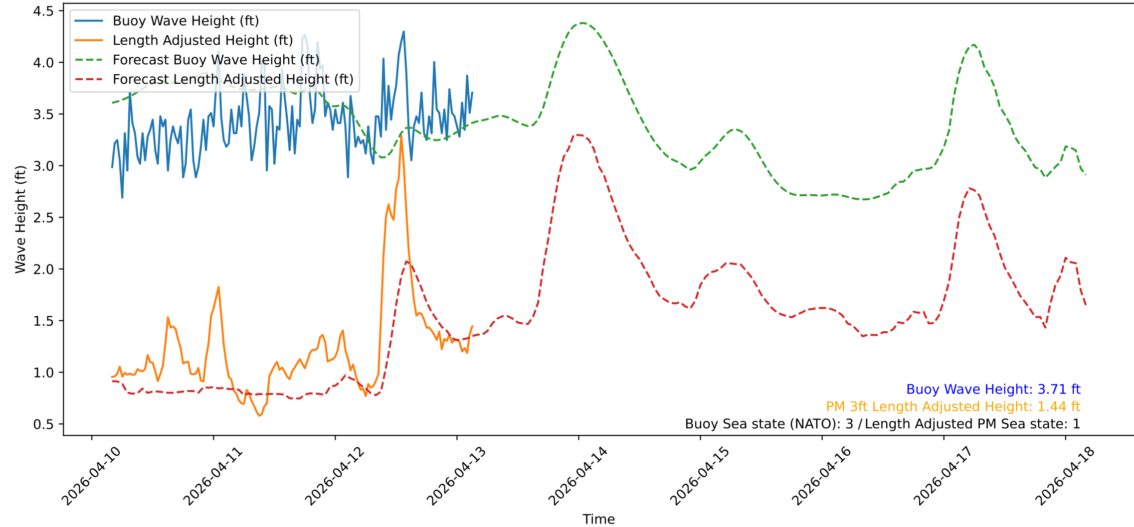
Wave Heights over Time for Red Beach at 2026-04-13 03:50:51
