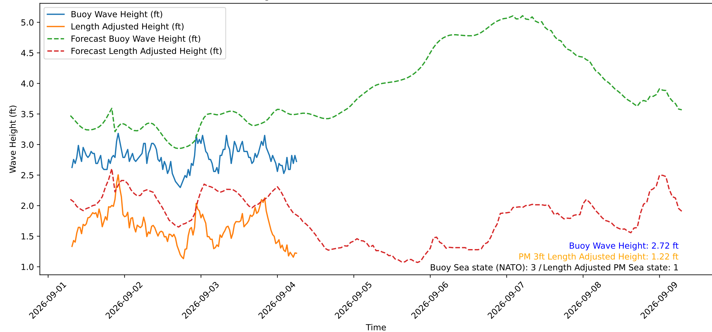
Wave Heights over Time for Red Beach at 2026-09-04 07:00:49
