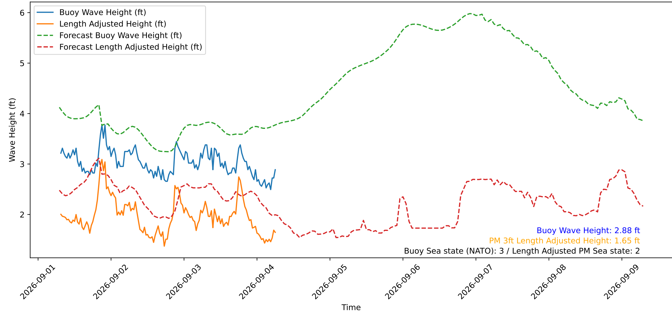
Wave Heights over Time for Green Beach at 2026-09-04 07:01:12
