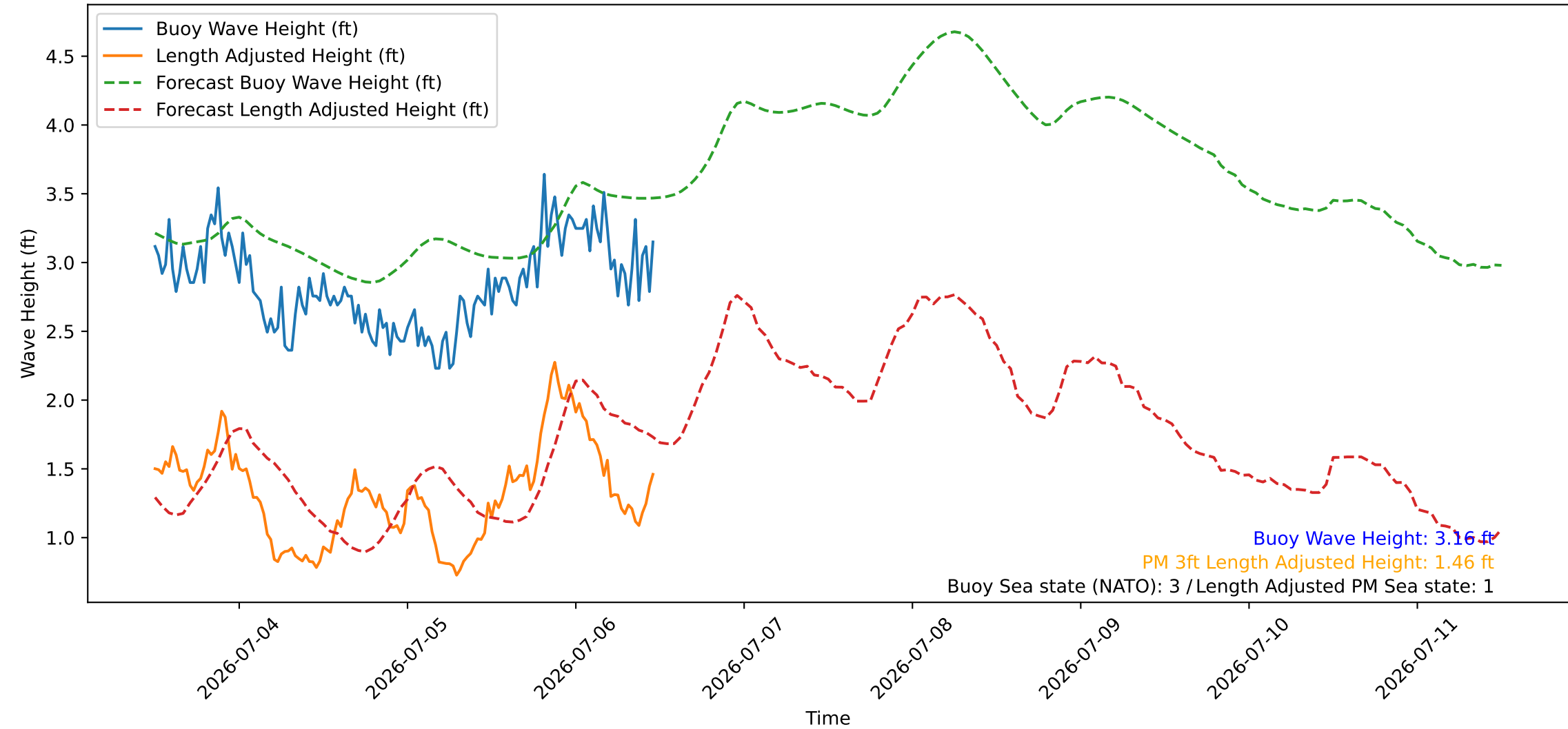
Wave Heights over Time for Red Beach at 2026-07-06 11:40:47
