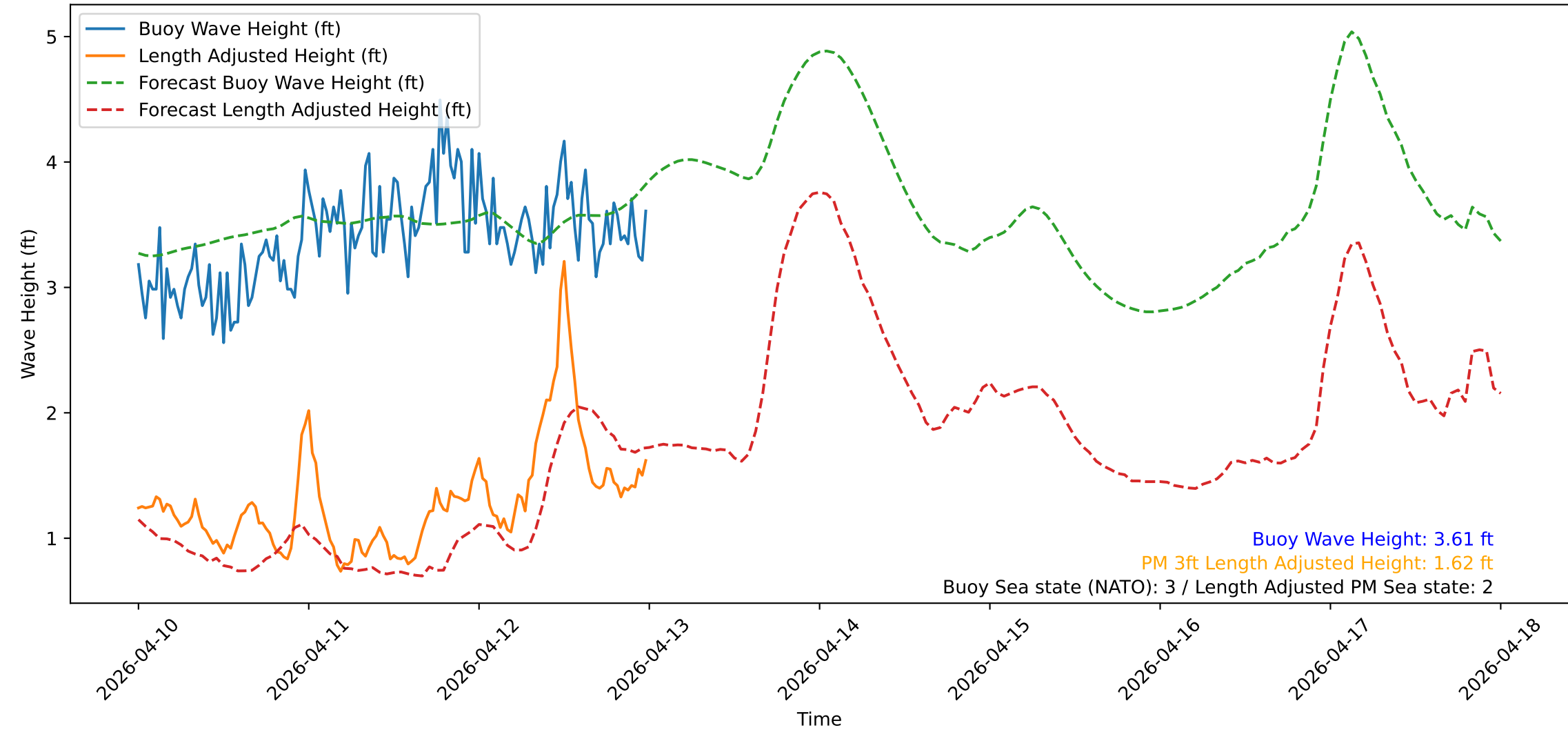
Wave Heights over Time for Green Beach at 2026-04-13 00:11:12
