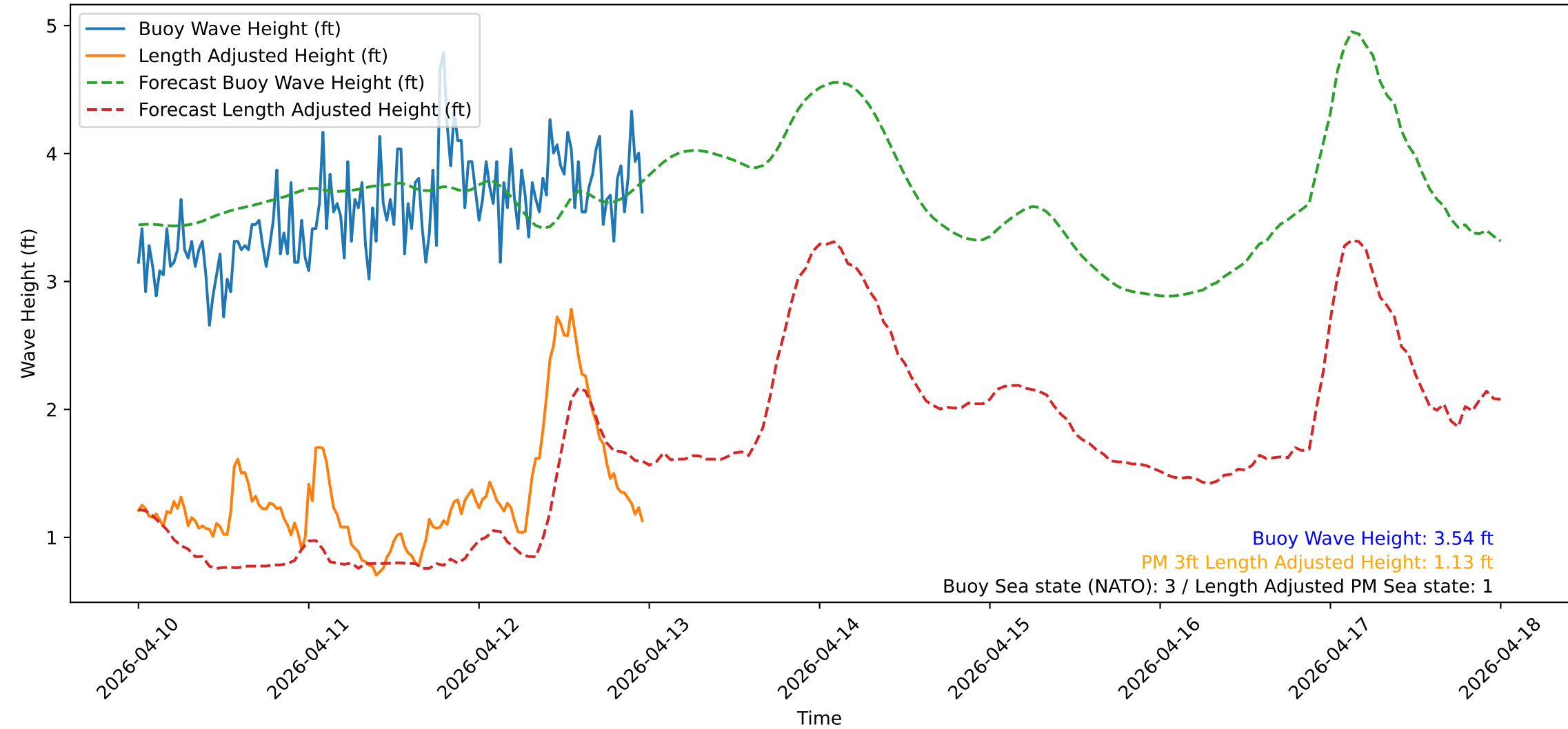
Wave Heights over Time for Oceanside Harbor at 2026-04-13 00:10:31
