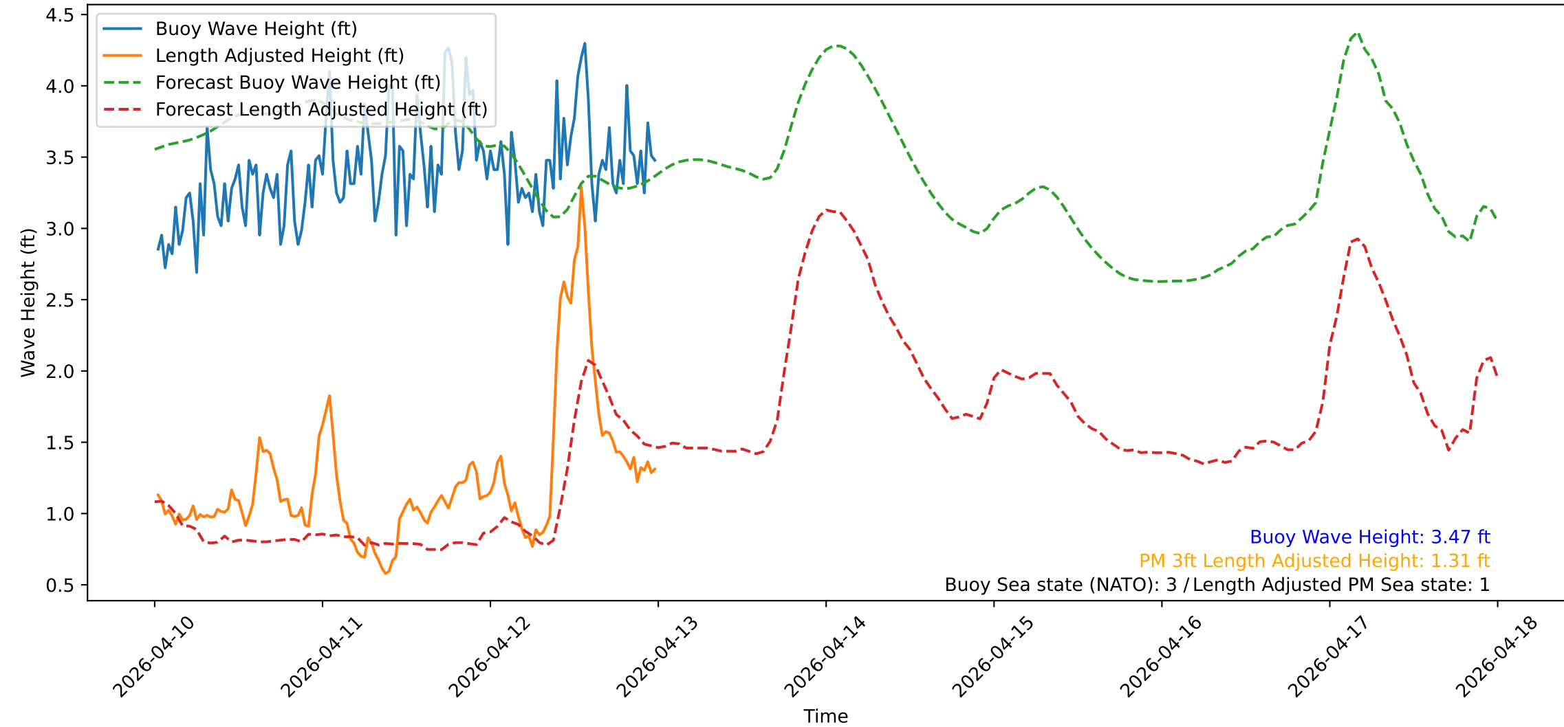
Wave Heights over Time for Red Beach at 2026-04-13 00:10:50
