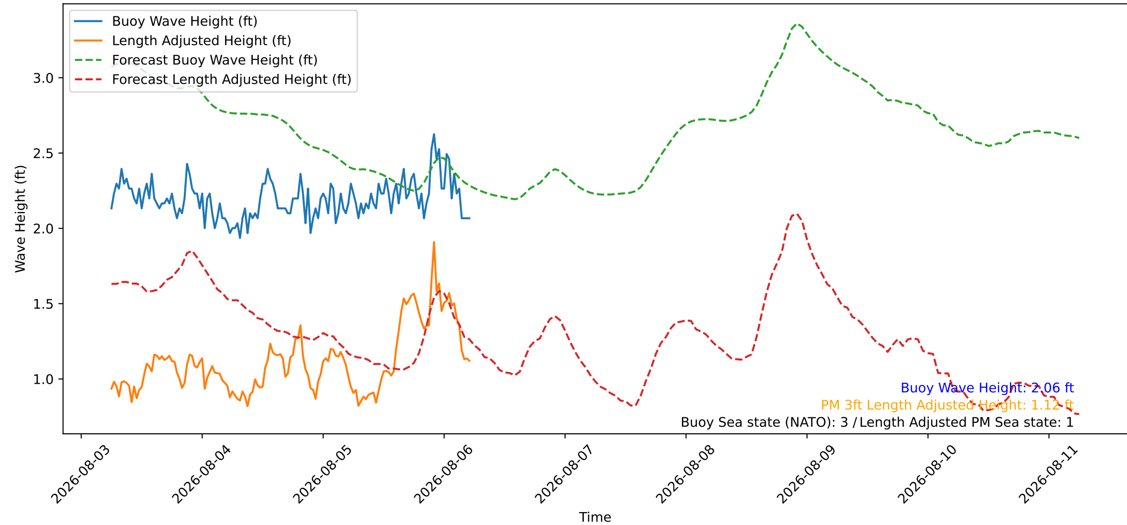
Wave Heights over Time for Green Beach at 2026-08-06 05:51:10
