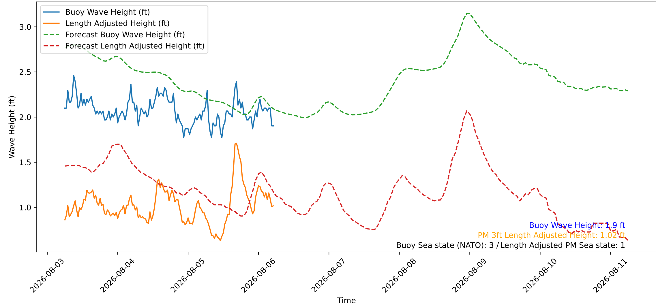
Wave Heights over Time for Red Beach at 2026-08-06 05:50:48
