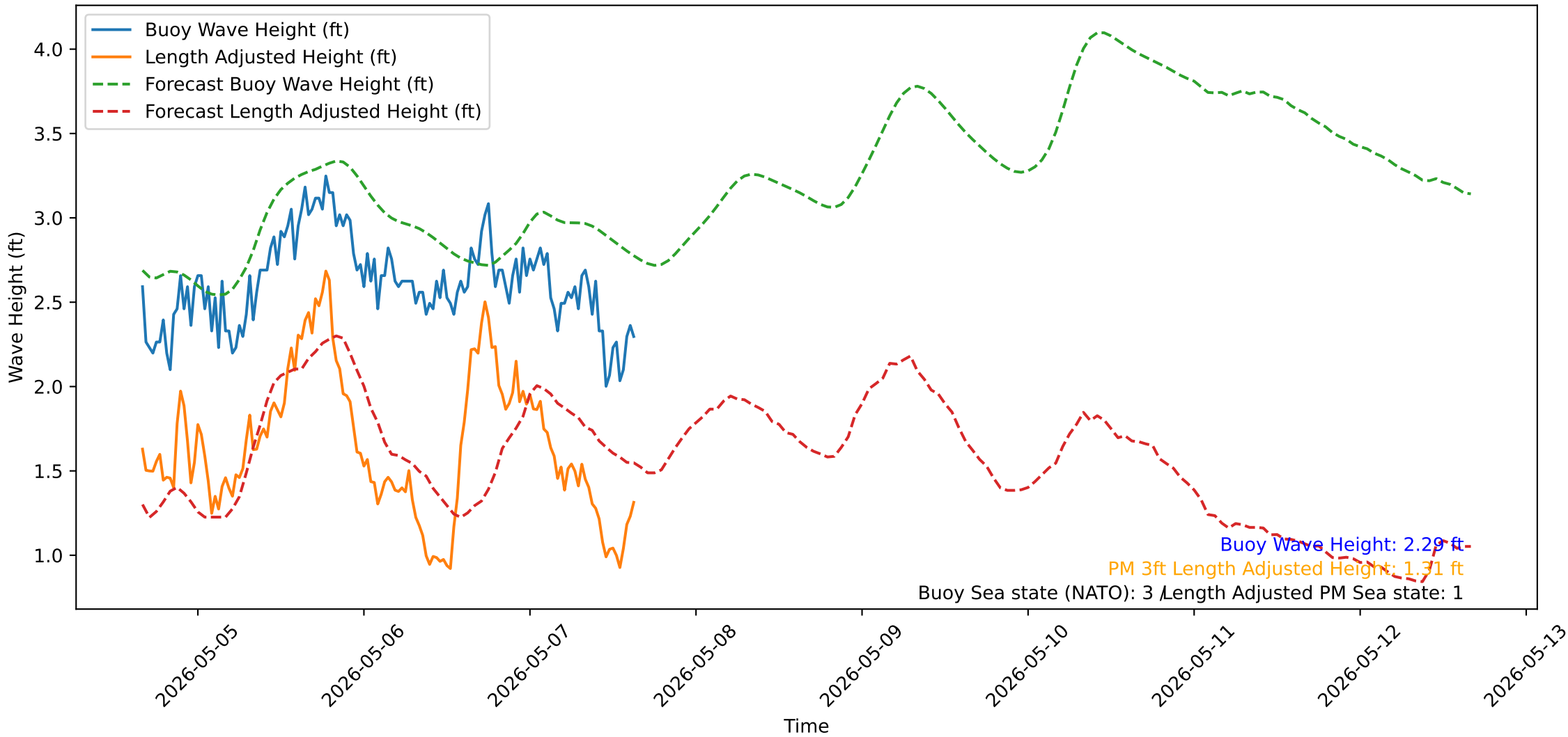
Wave Heights over Time for Oceanside Harbor at 2026-05-07 16:00:31
