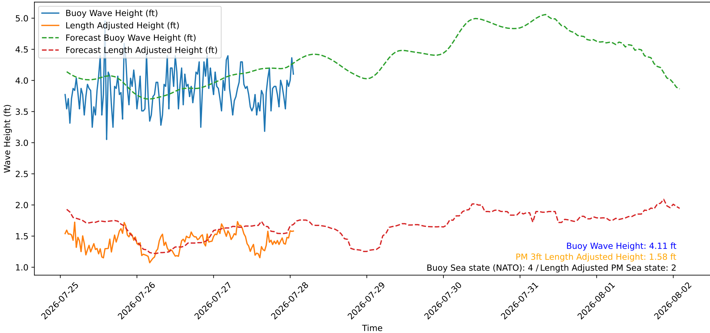
Wave Heights over Time for Oceanside Harbor at 2026-07-28 01:40:26
