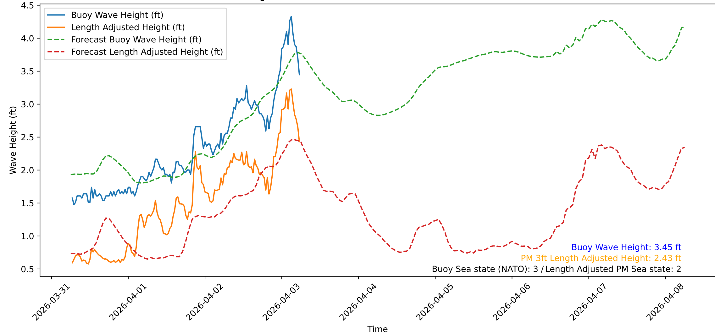
Wave Heights over Time for Green Beach at 2026-04-03 06:21:10
