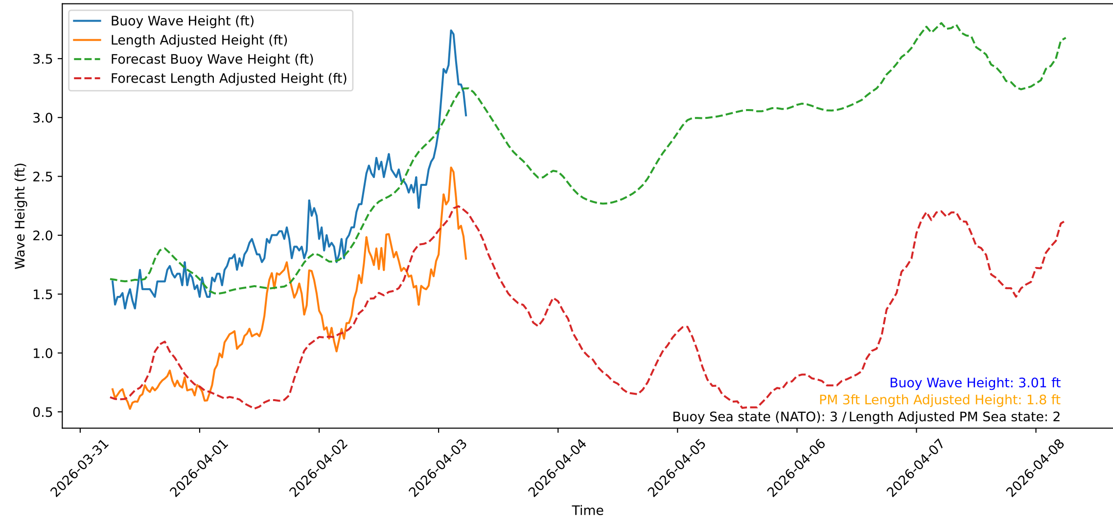
Wave Heights over Time for Red Beach at 2026-04-03 06:20:47
