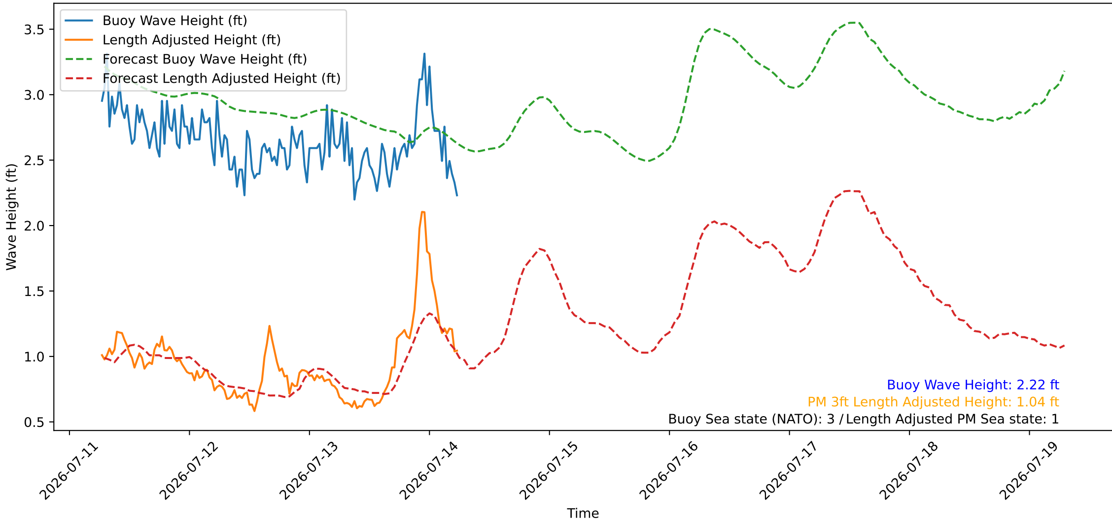
Wave Heights over Time for Green Beach at 2026-07-14 06:31:08
