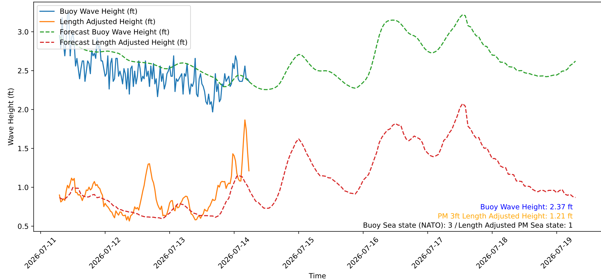
Wave Heights over Time for Red Beach at 2026-07-14 06:30:45
