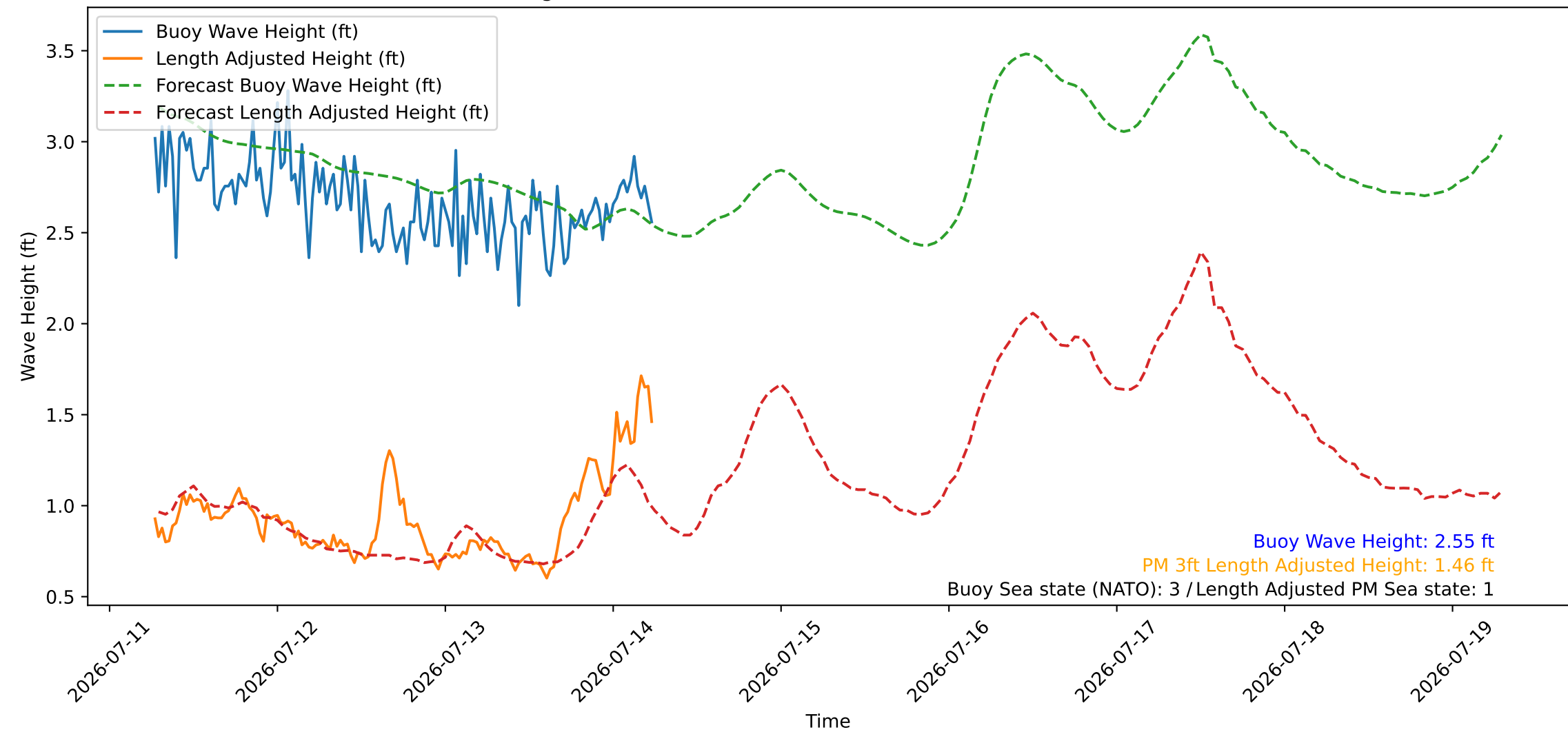
Wave Heights over Time for Oceanside Harbor at 2026-07-14 06:30:26
