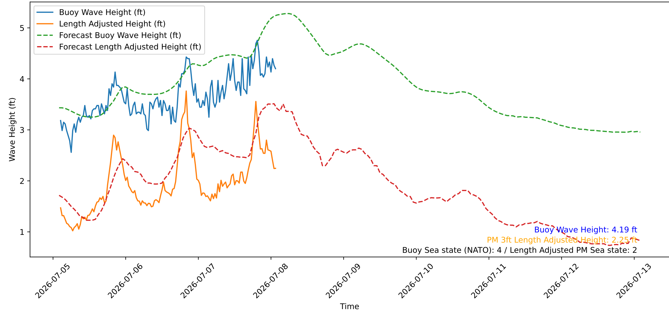
Wave Heights over Time for Green Beach at 2026-07-08 02:21:09
