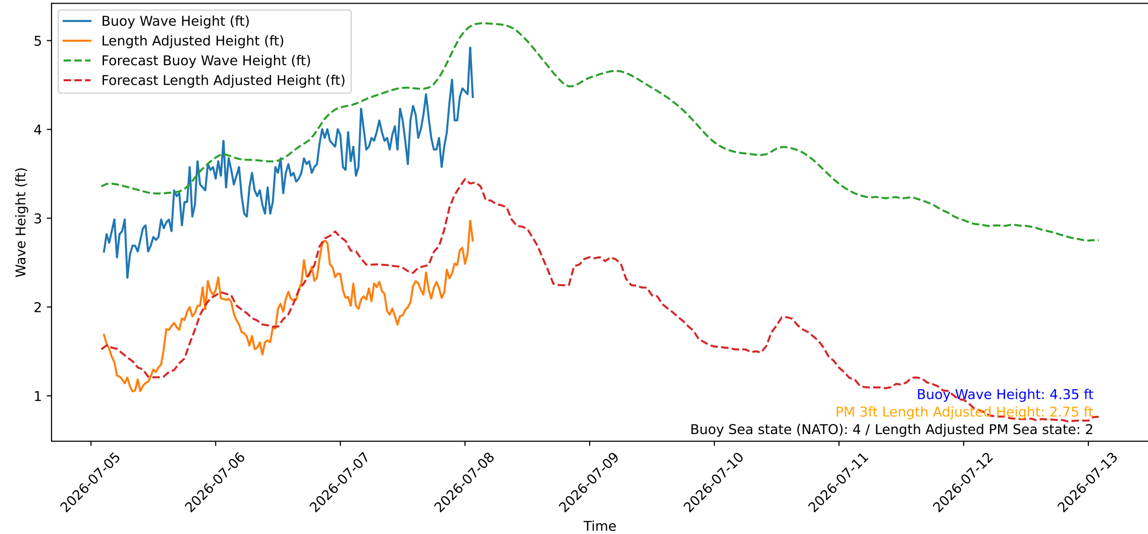
Wave Heights over Time for Oceanside Harbor at 2026-07-08 02:20:26
