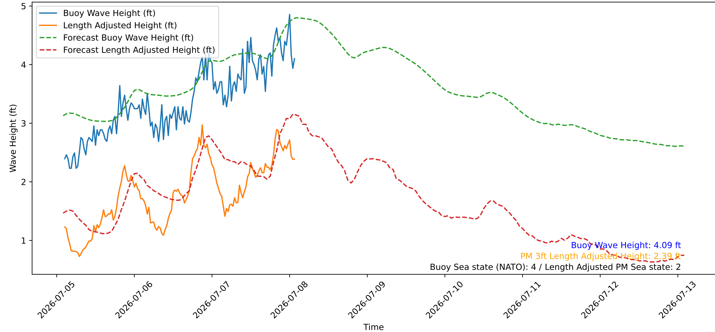
Wave Heights over Time for Red Beach at 2026-07-08 02:20:47
