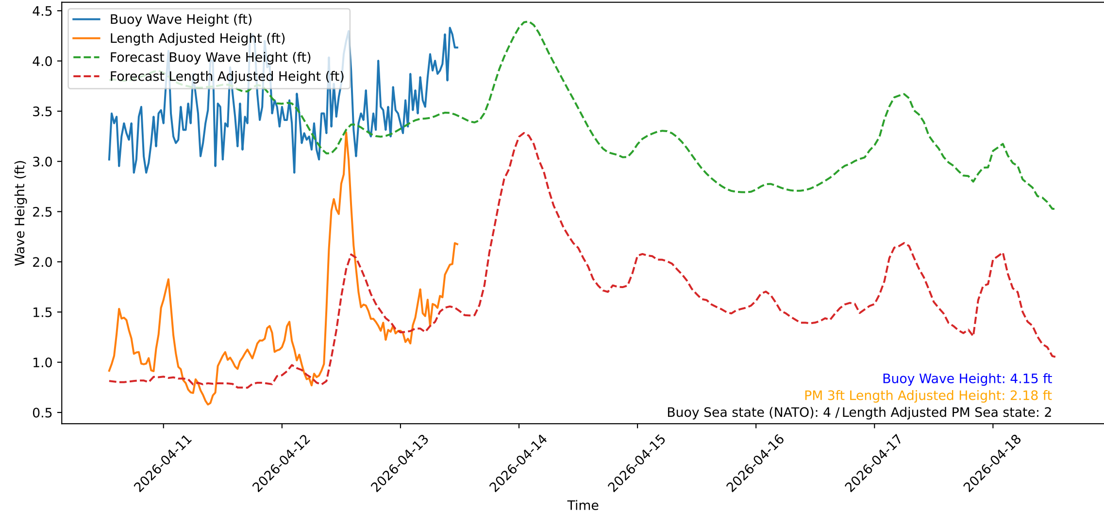
Wave Heights over Time for Red Beach at 2026-04-13 12:30:50
