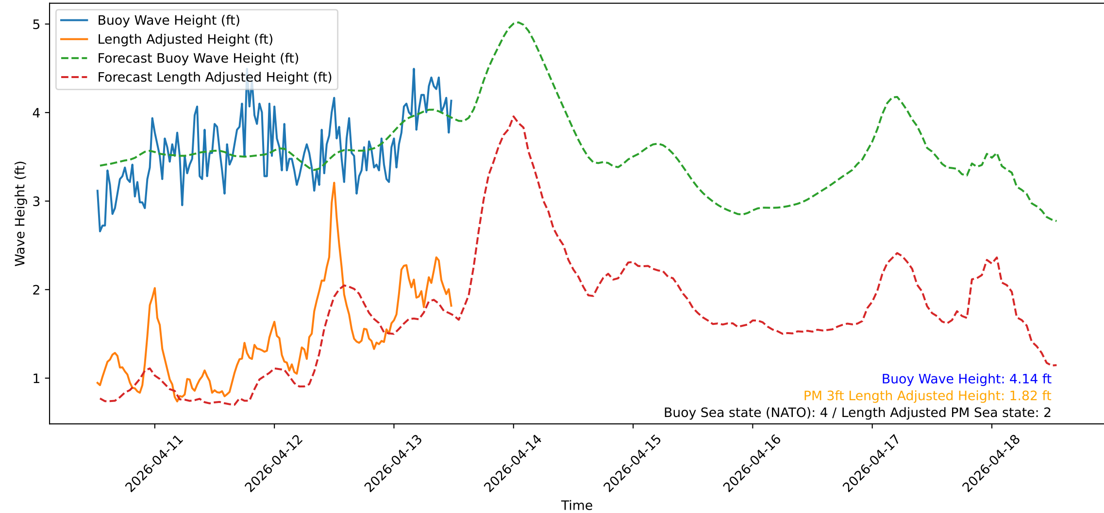
Wave Heights over Time for Green Beach at 2026-04-13 12:31:13
