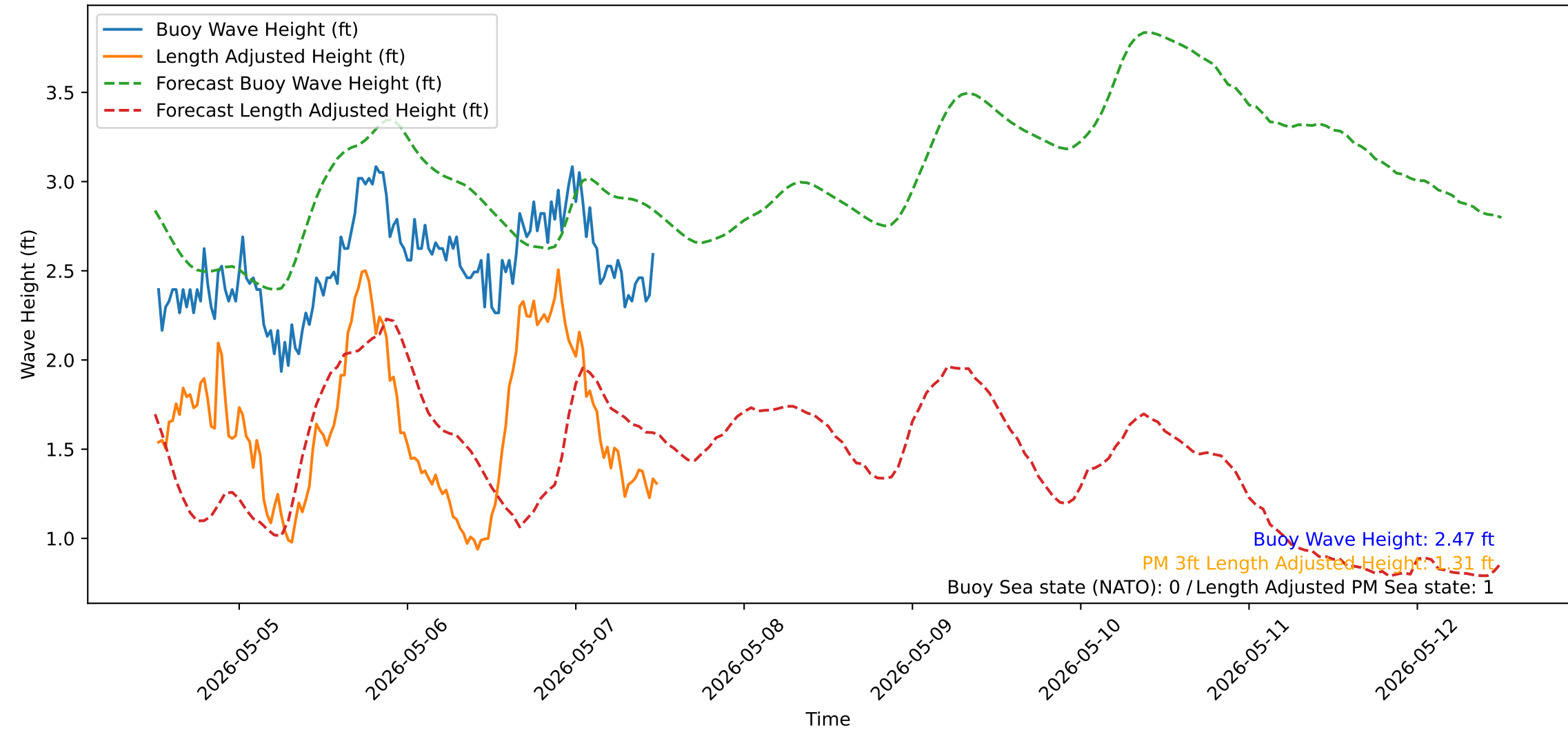
Wave Heights over Time for Red Beach at 2026-05-07 12:20:52
