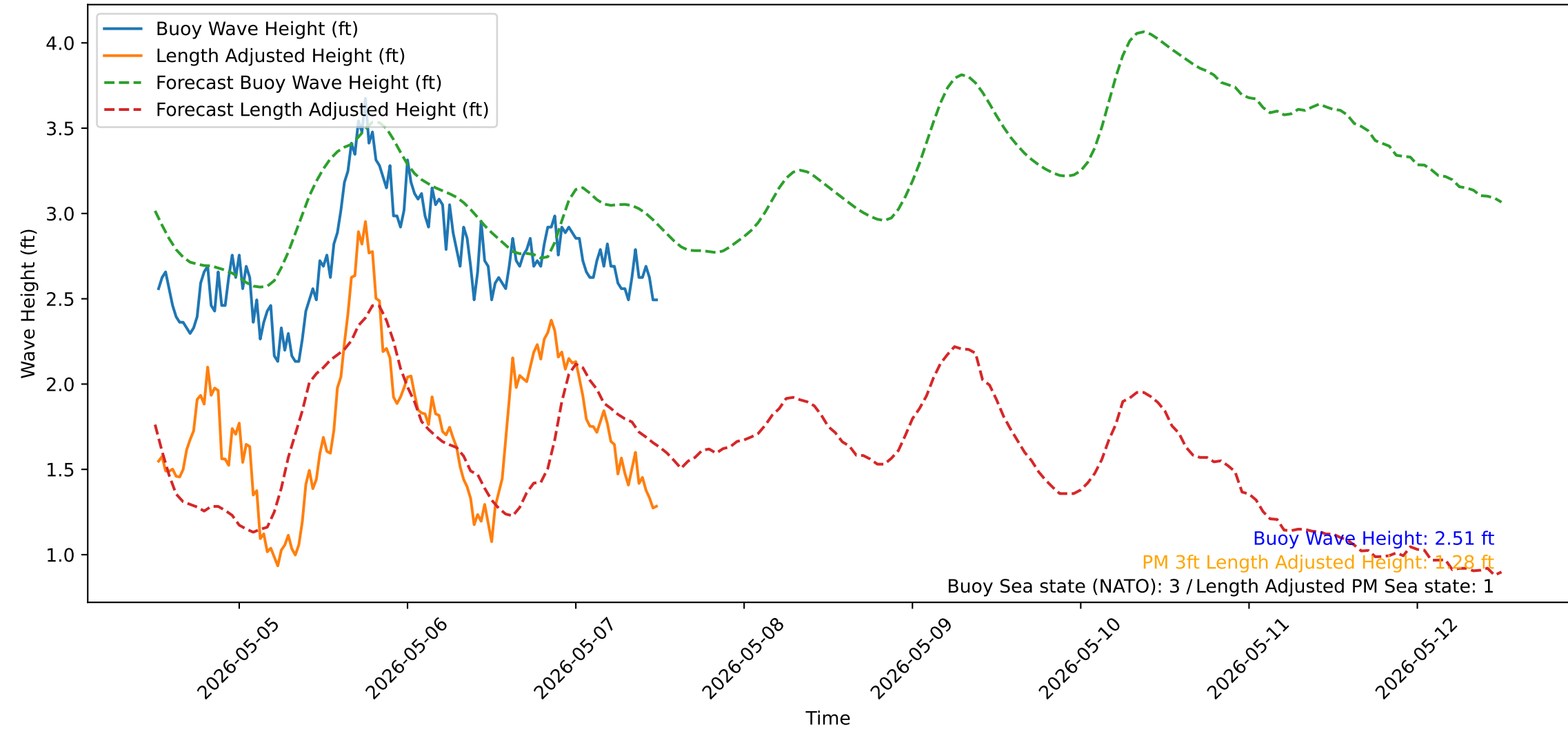
Wave Heights over Time for Green Beach at 2026-05-07 12:21:15
