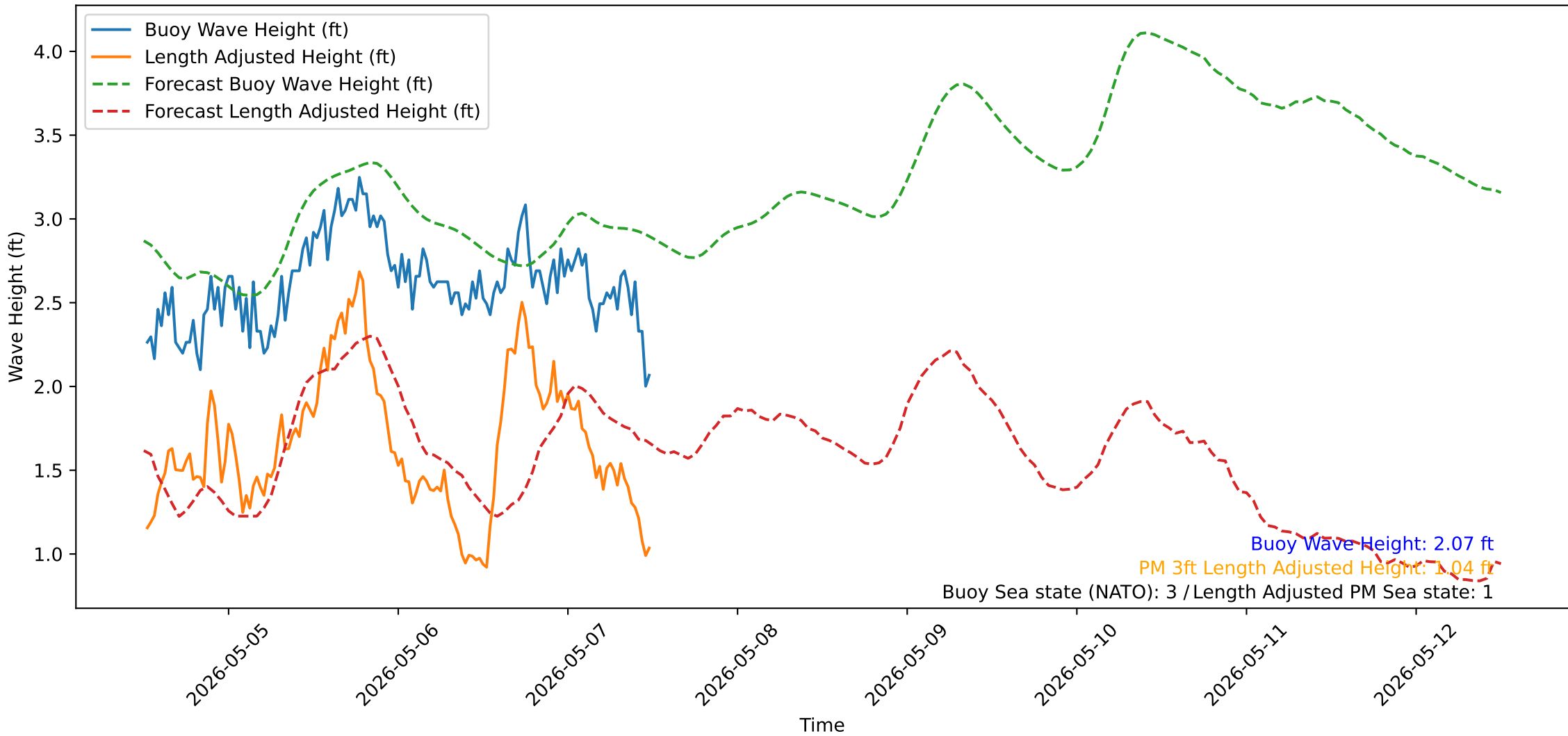
Wave Heights over Time for Oceanside Harbor at 2026-05-07 12:20:32
