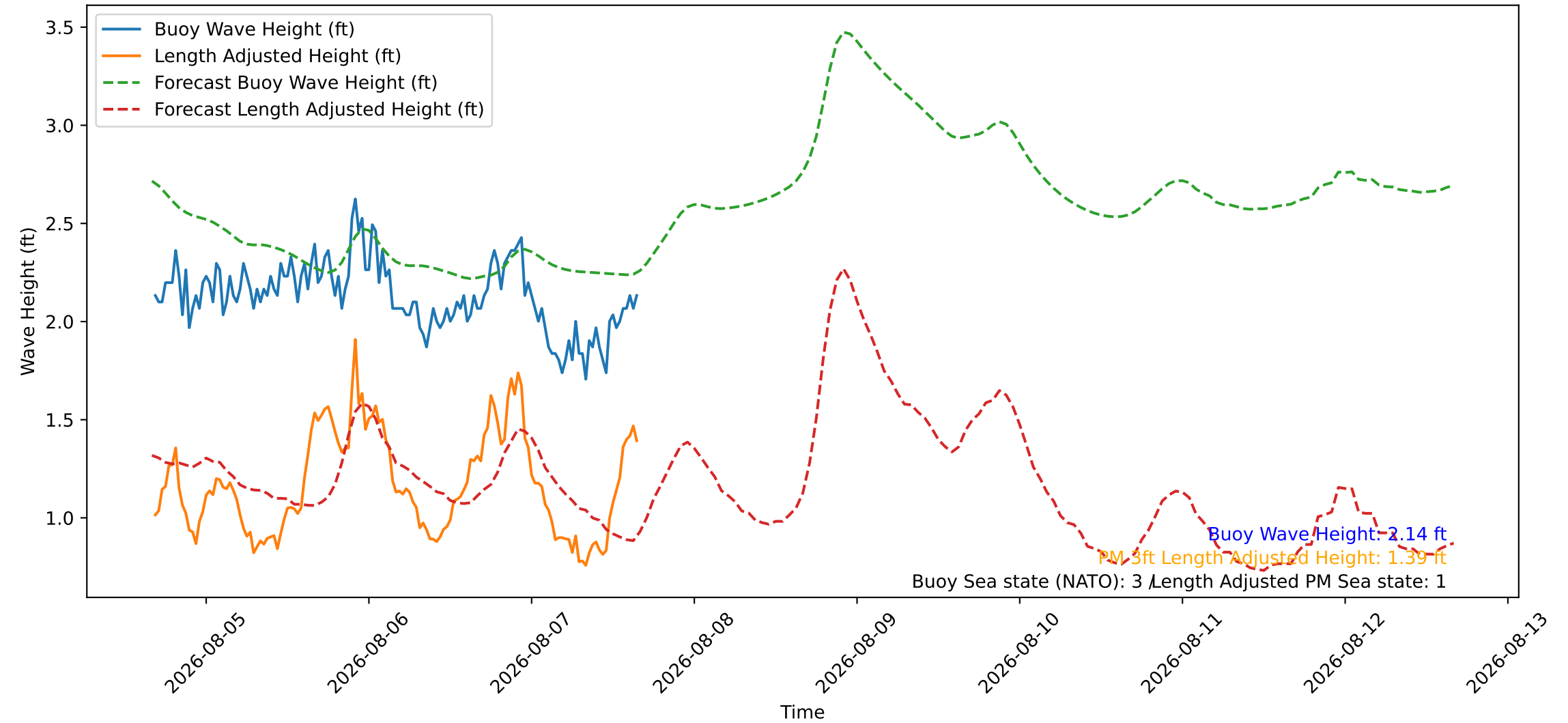
Wave Heights over Time for Green Beach at 2026-08-07 16:21:09
