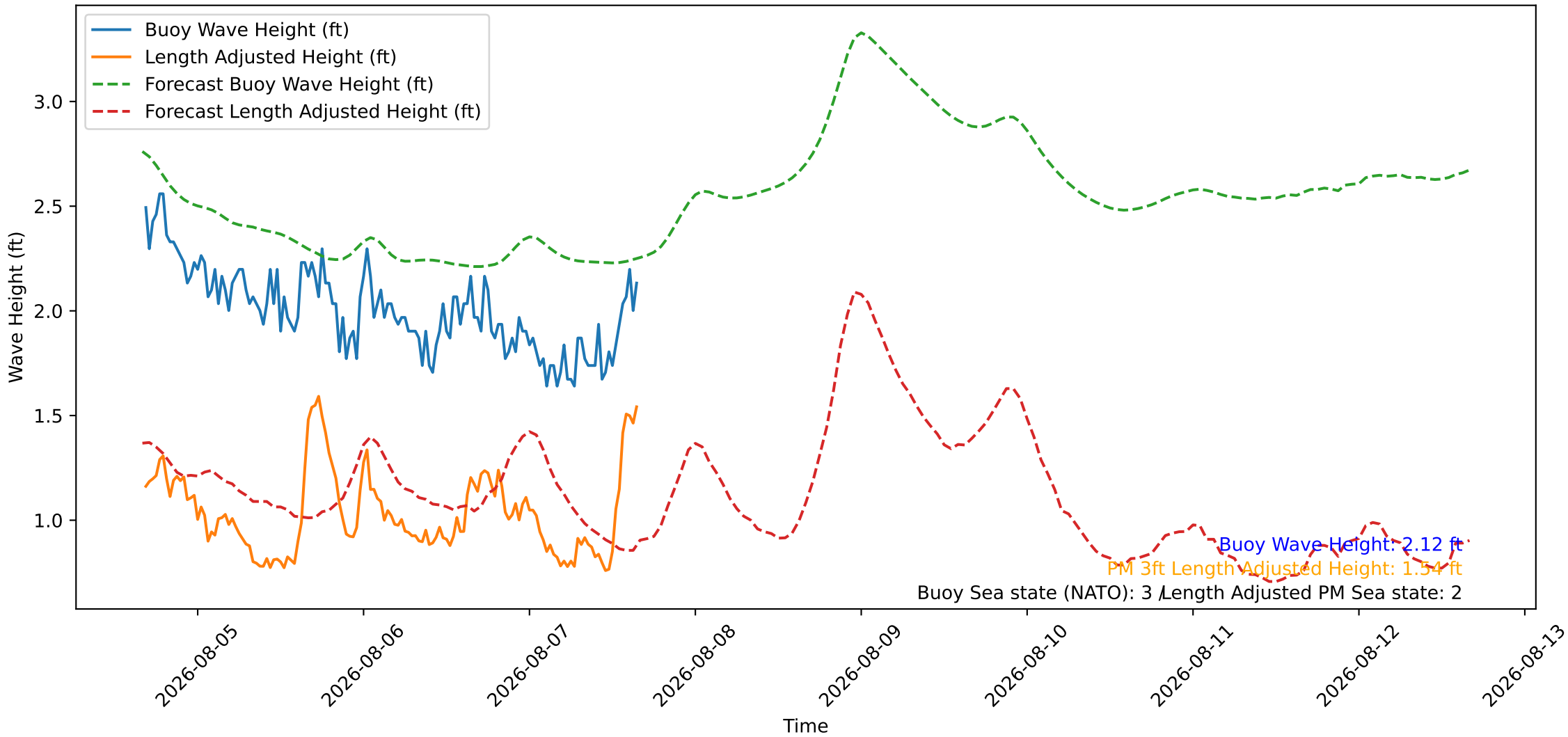
Wave Heights over Time for Oceanside Harbor at 2026-08-07 16:20:26
