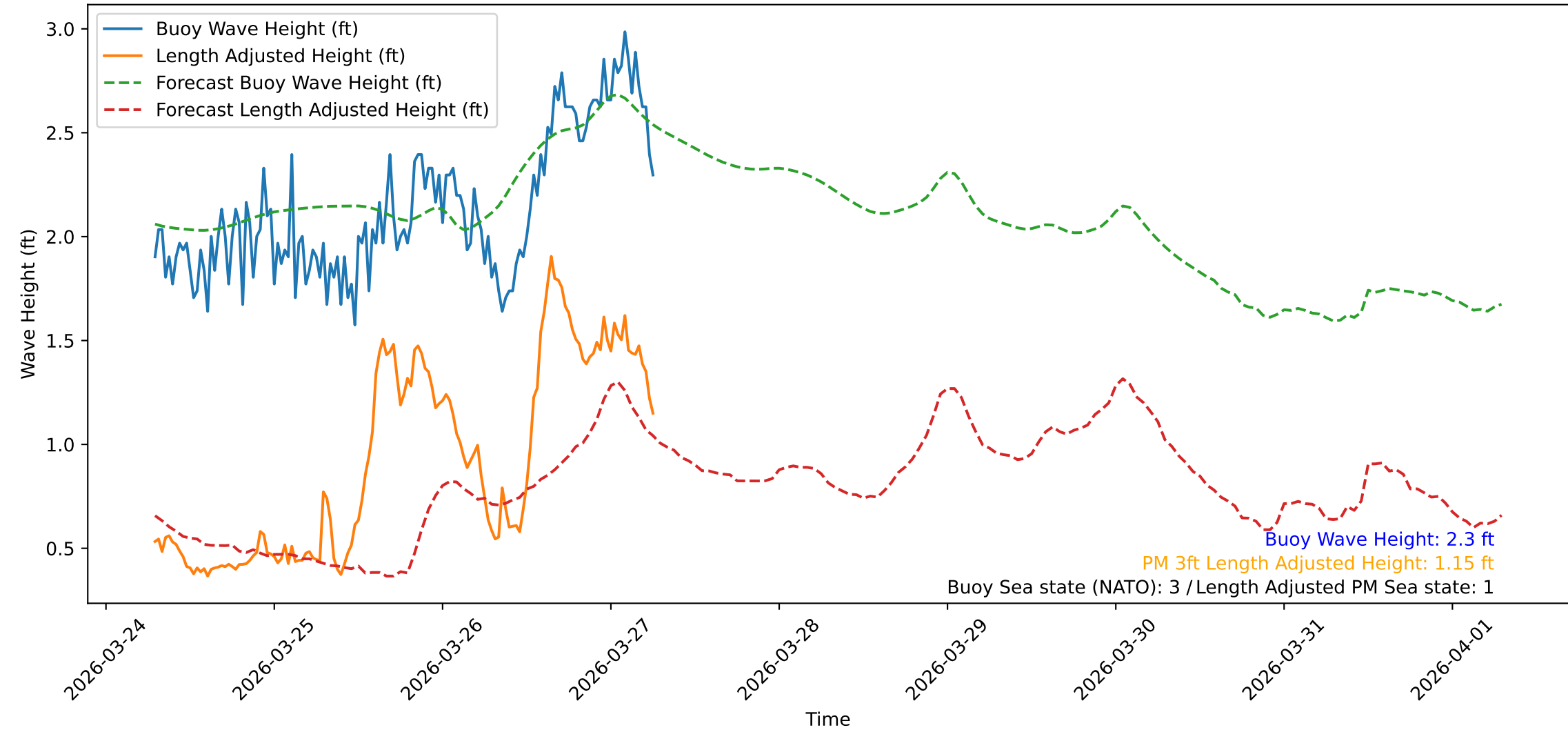
Wave Heights over Time for Red Beach at 2026-03-27 06:40:47
