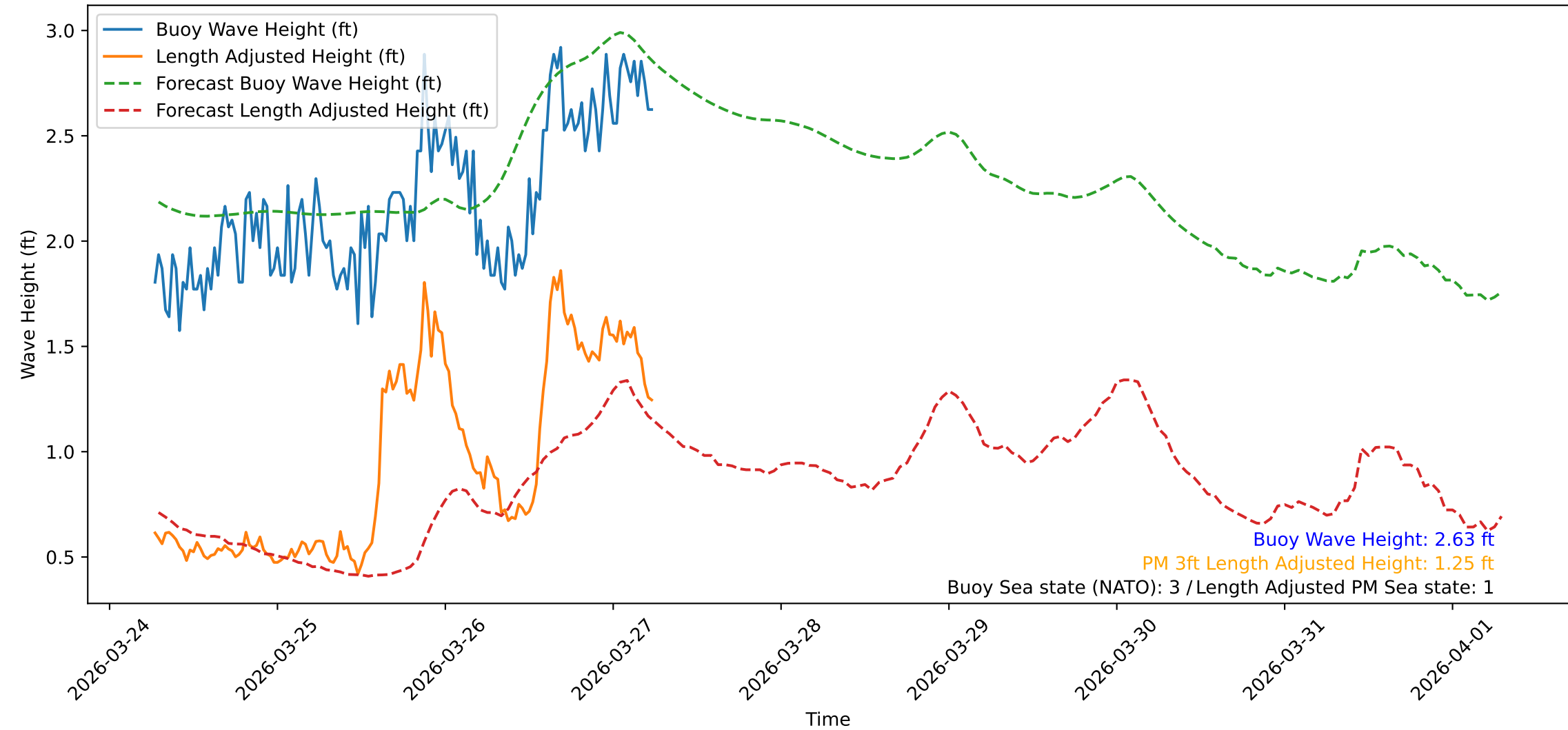
Wave Heights over Time for Oceanside Harbor at 2026-03-27 06:40:31
