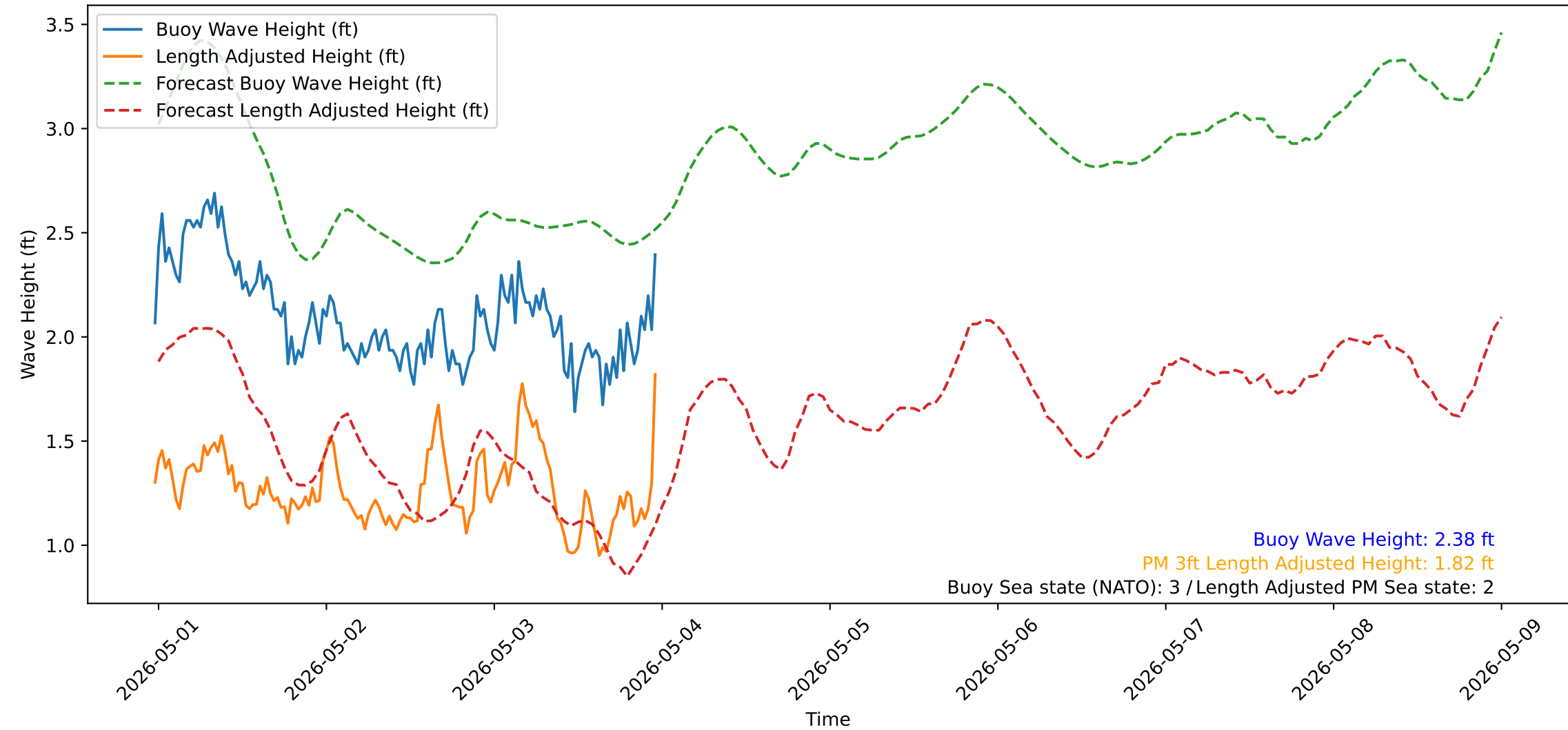
Wave Heights over Time for Oceanside Harbor at 2026-05-03 23:40:32
