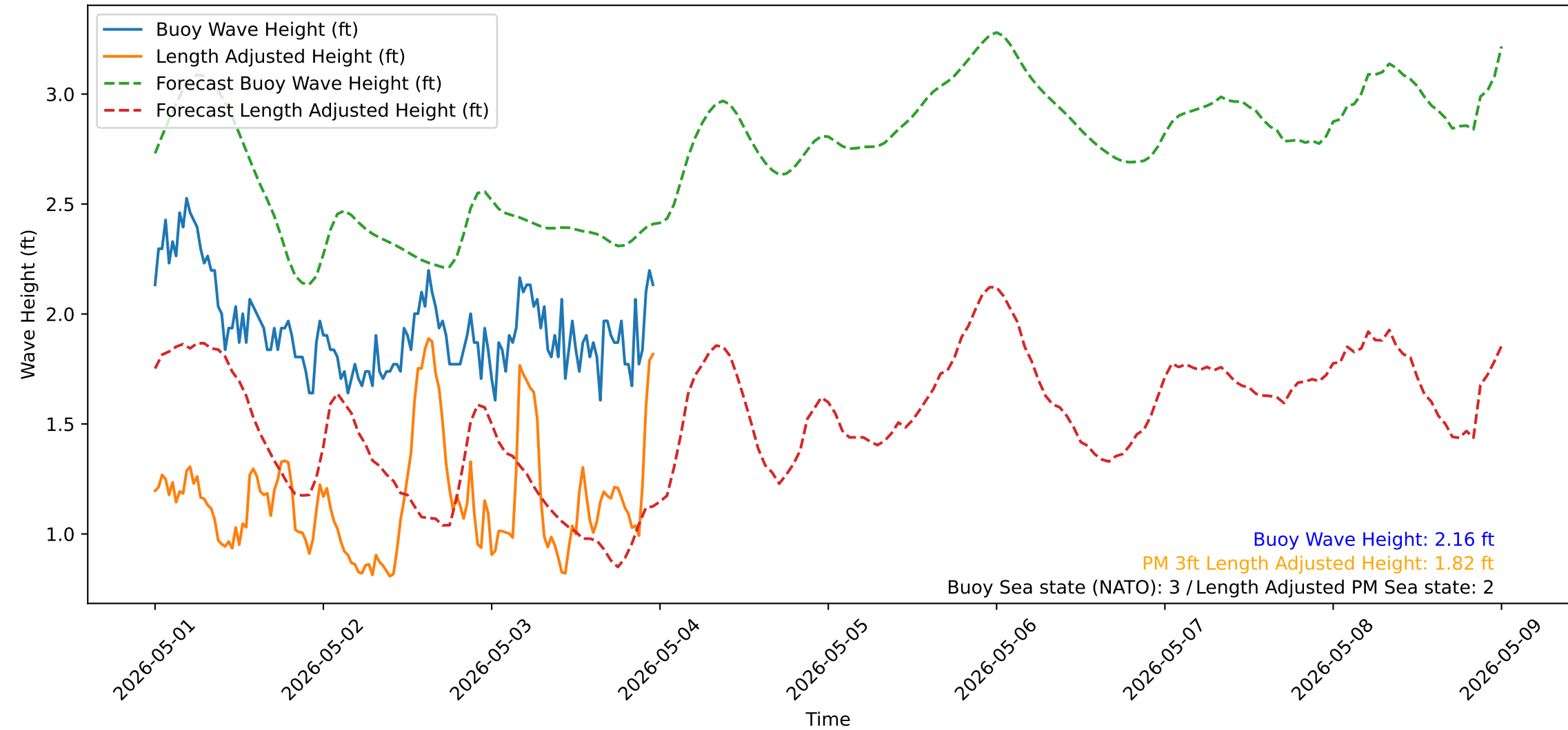
Wave Heights over Time for Red Beach at 2026-05-03 23:40:51
