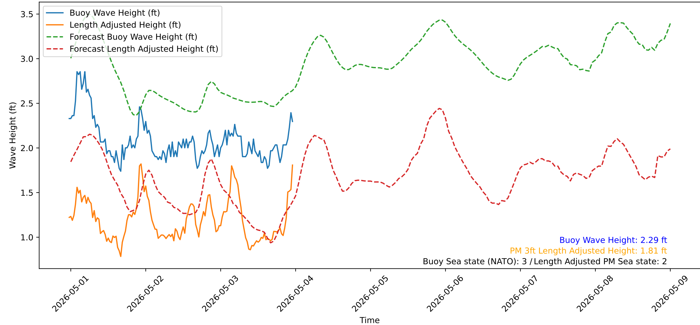
Wave Heights over Time for Green Beach at 2026-05-03 23:41:14
