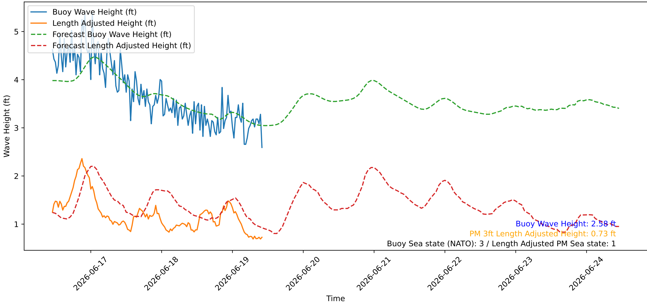
Wave Heights over Time for Red Beach at 2026-06-19 10:50:46
