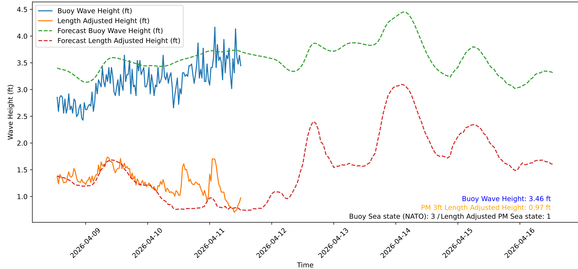
Wave Heights over Time for Oceanside Harbor at 2026-04-11 12:50:31
