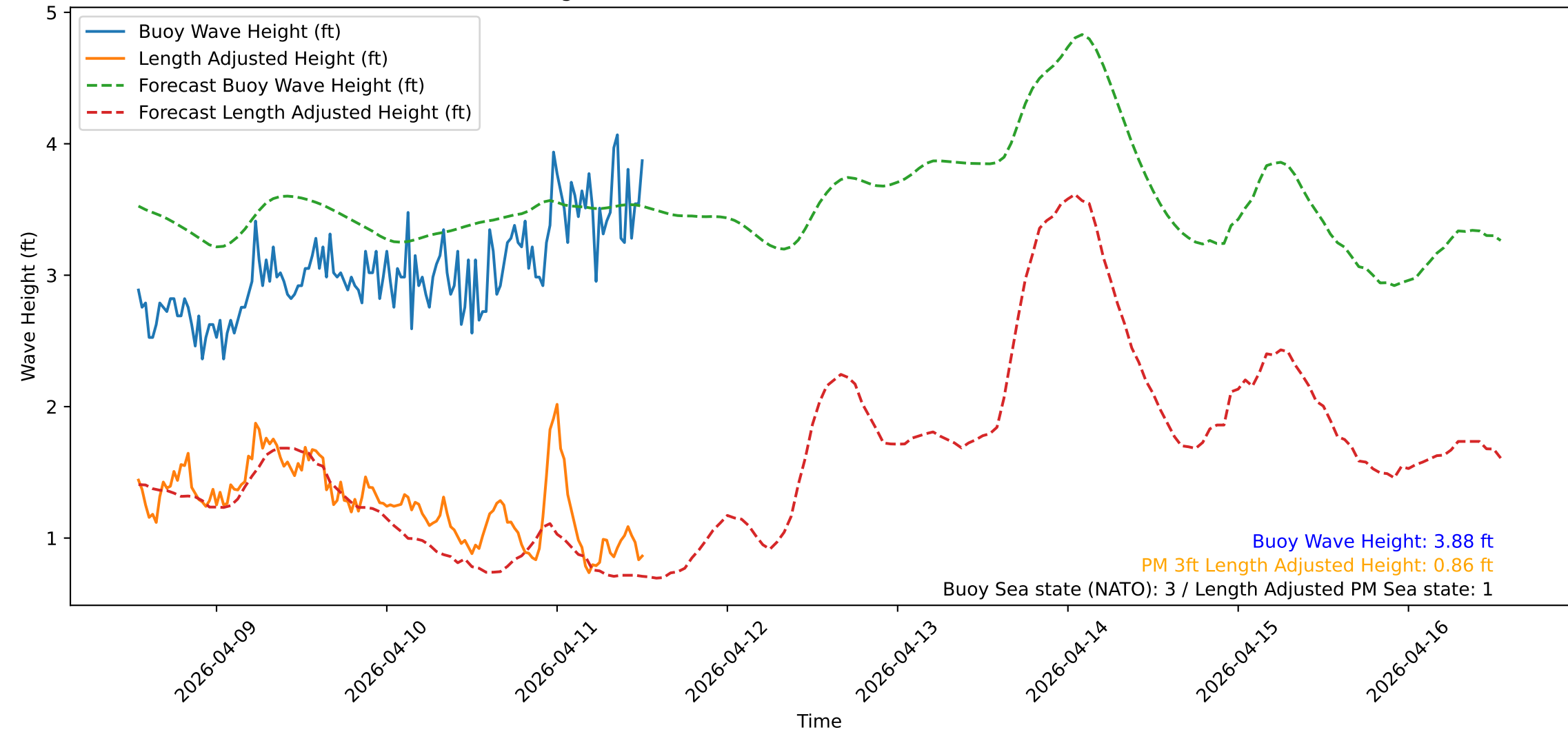
Wave Heights over Time for Green Beach at 2026-04-11 12:51:13
