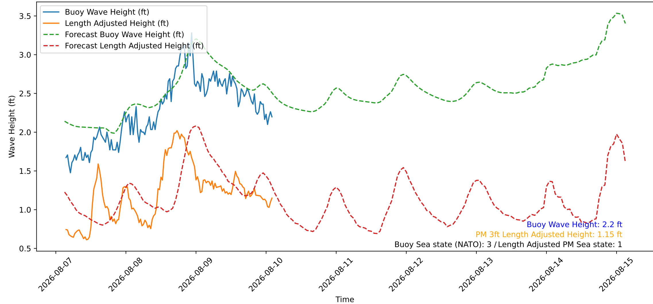
Wave Heights over Time for Red Beach at 2026-08-10 03:00:46
