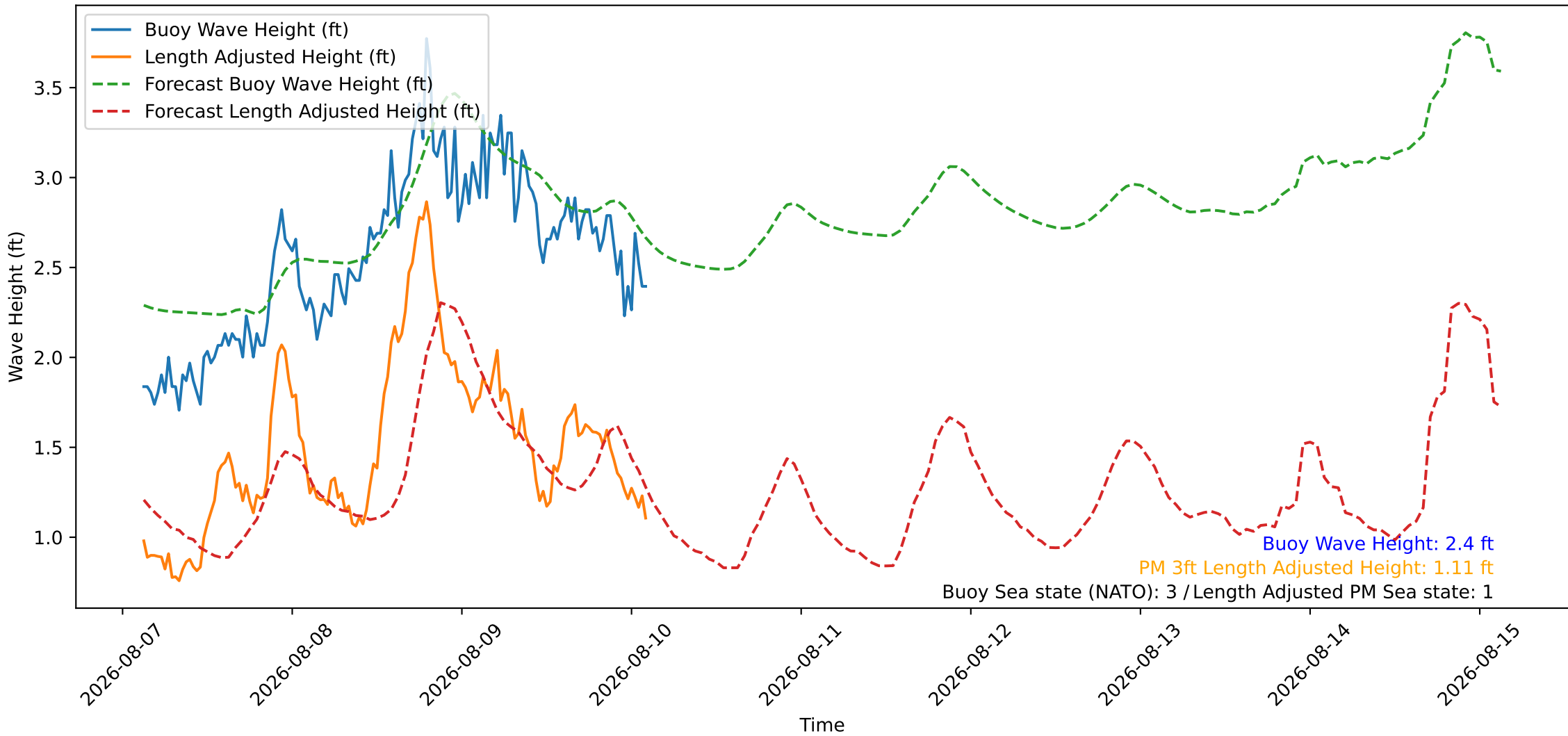
Wave Heights over Time for Green Beach at 2026-08-10 03:01:09
