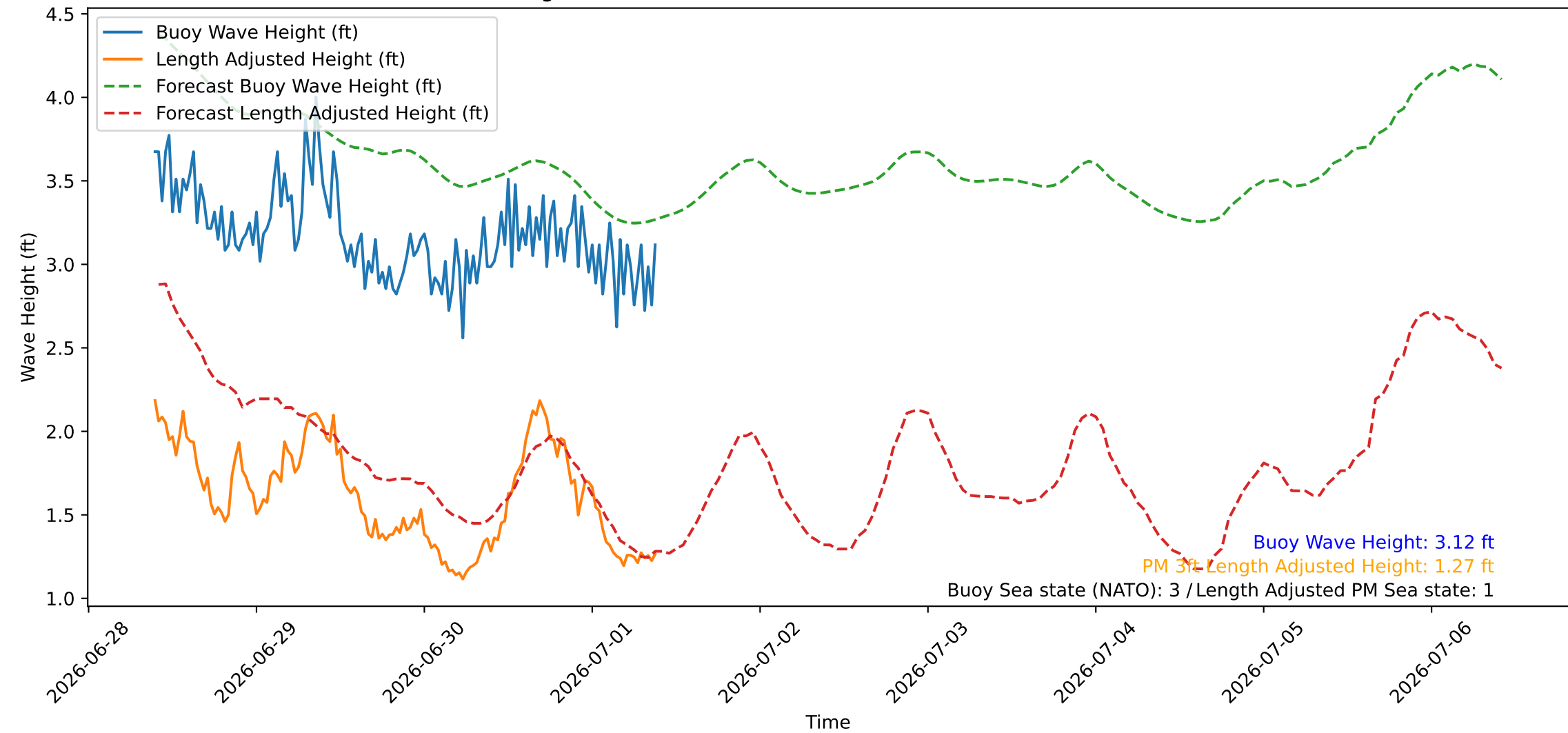
Wave Heights over Time for Oceanside Harbor at 2026-07-01 09:30:26
