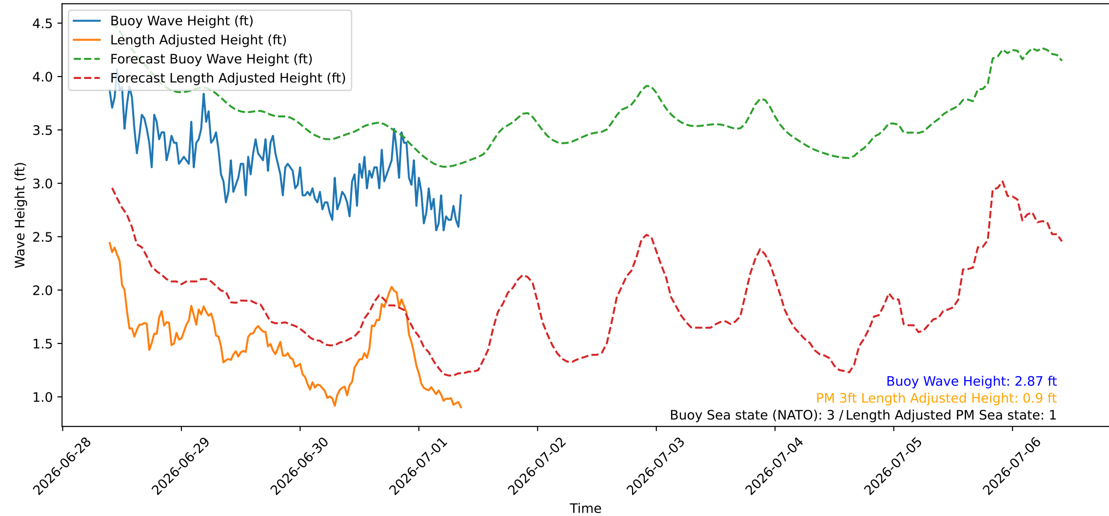
Wave Heights over Time for Green Beach at 2026-07-01 09:31:07
