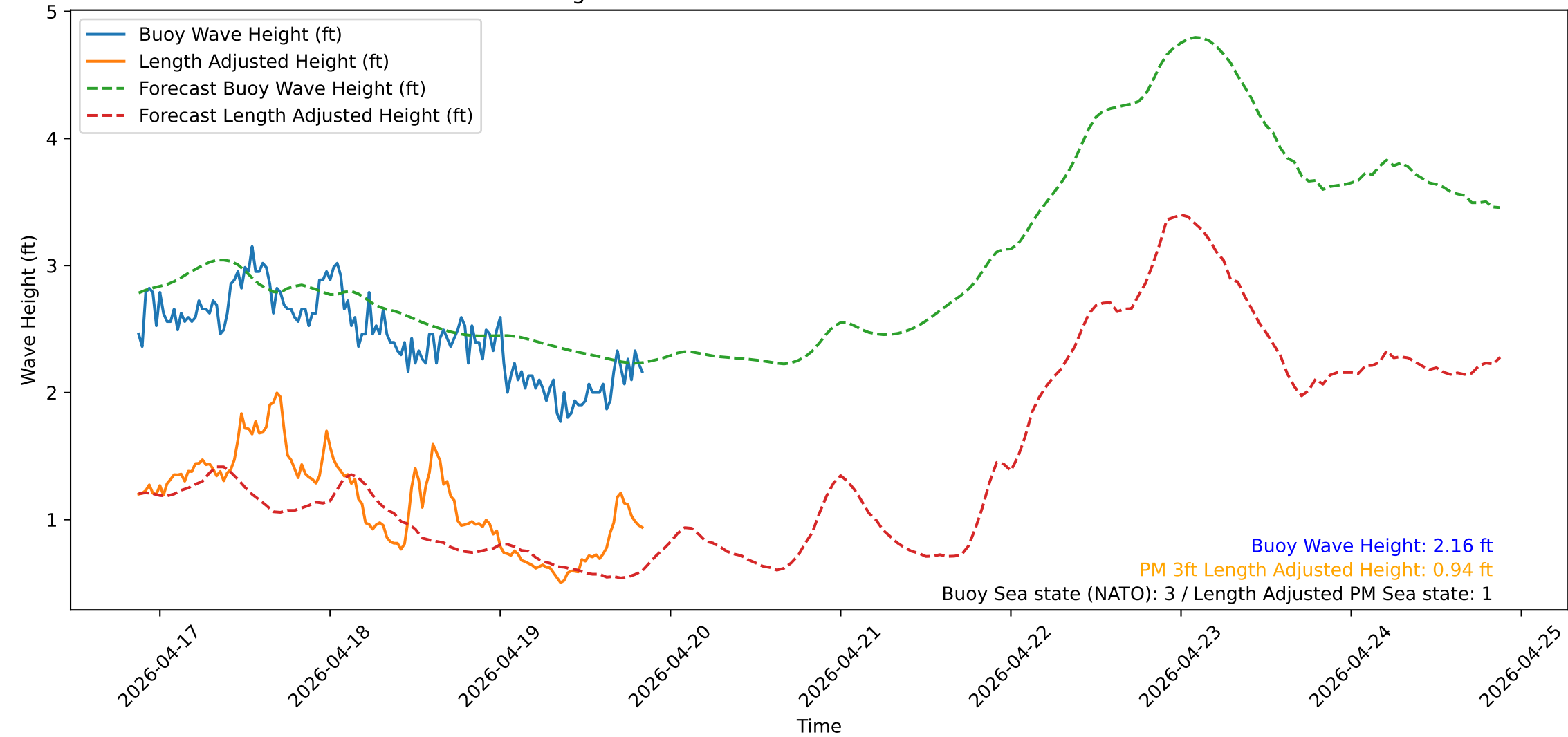
Wave Heights over Time for Red Beach at 2026-04-19 20:50:52
