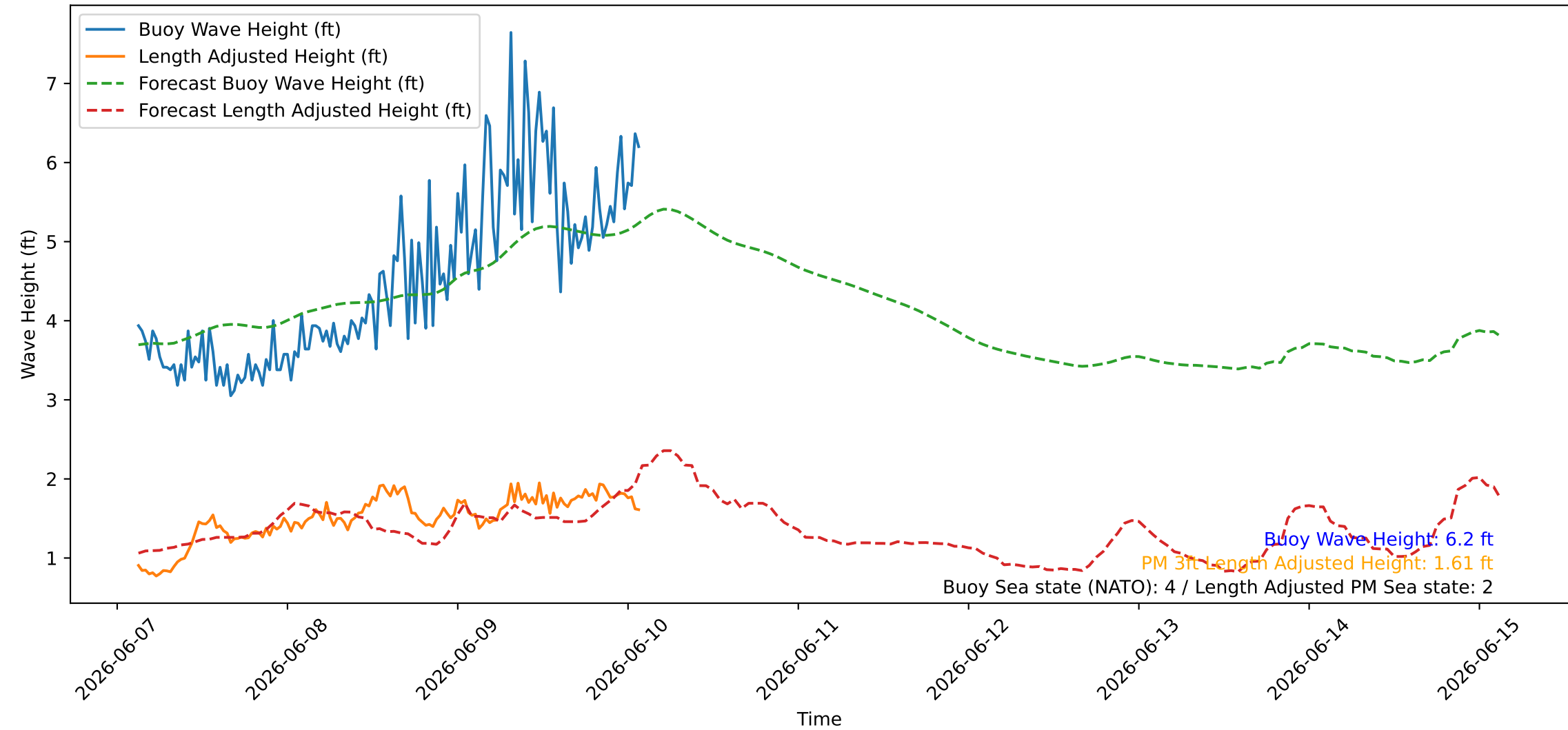
Wave Heights over Time for Red Beach at 2026-06-10 02:30:47
