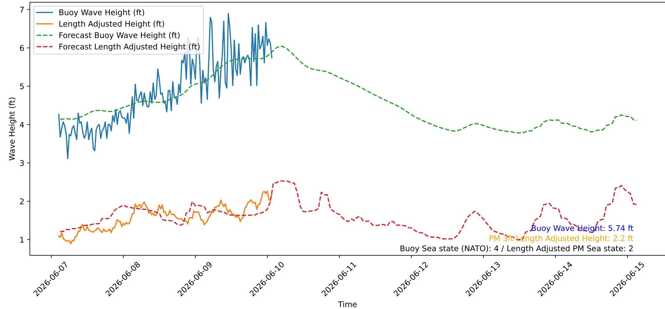
Wave Heights over Time for Green Beach at 2026-06-10 02:31:10
