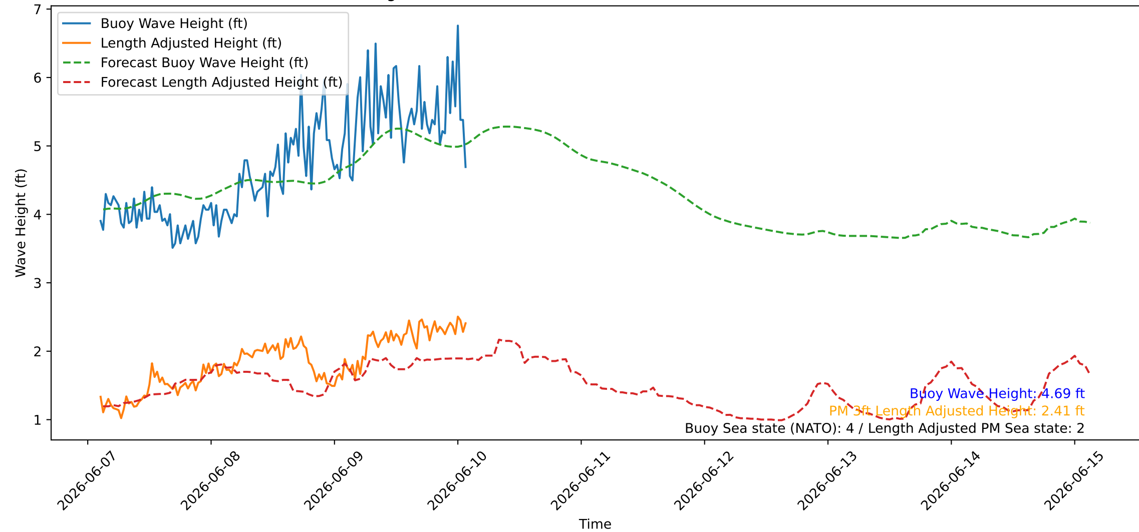
Wave Heights over Time for Oceanside Harbor at 2026-06-10 02:30:27
