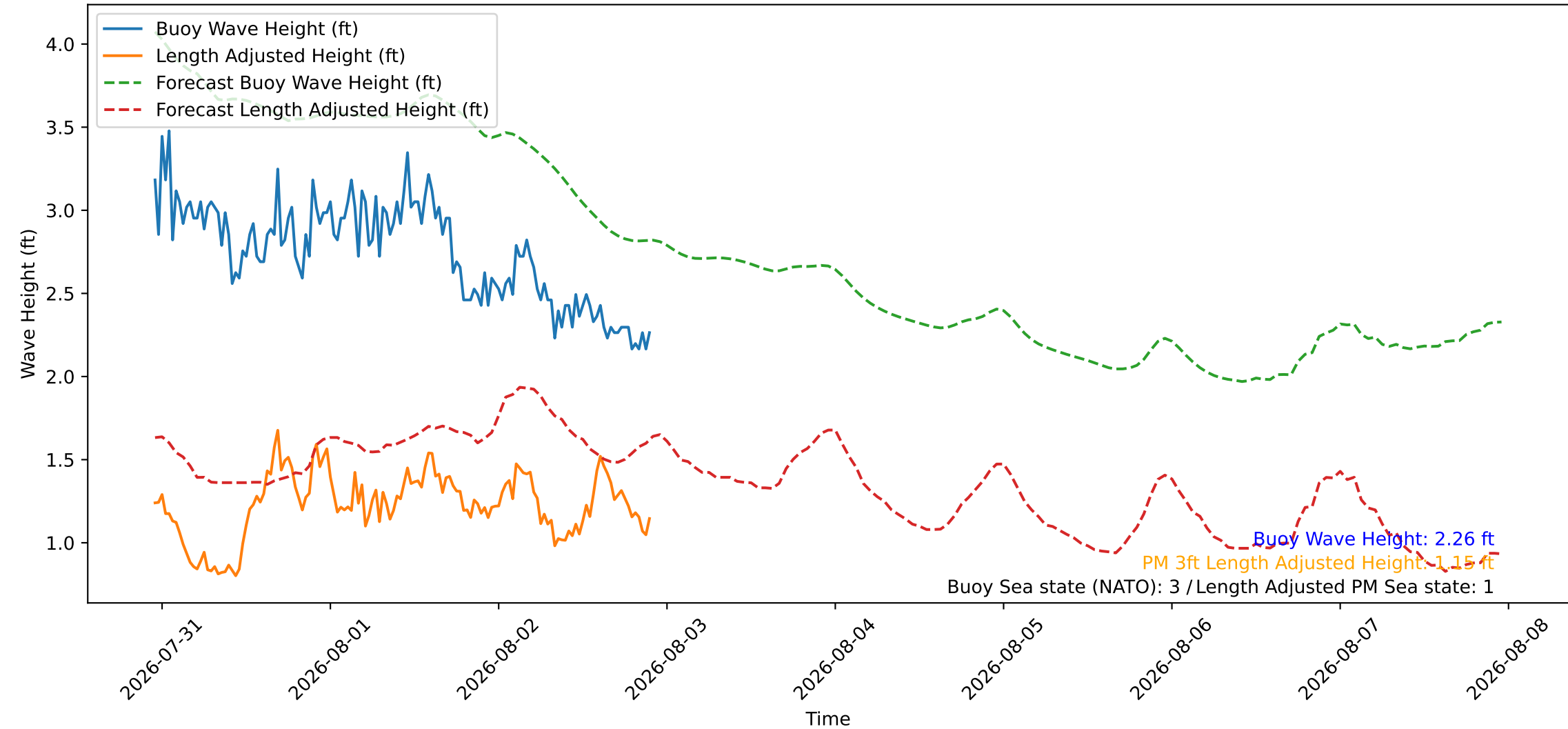
Wave Heights over Time for Red Beach at 2026-08-02 22:30:46
