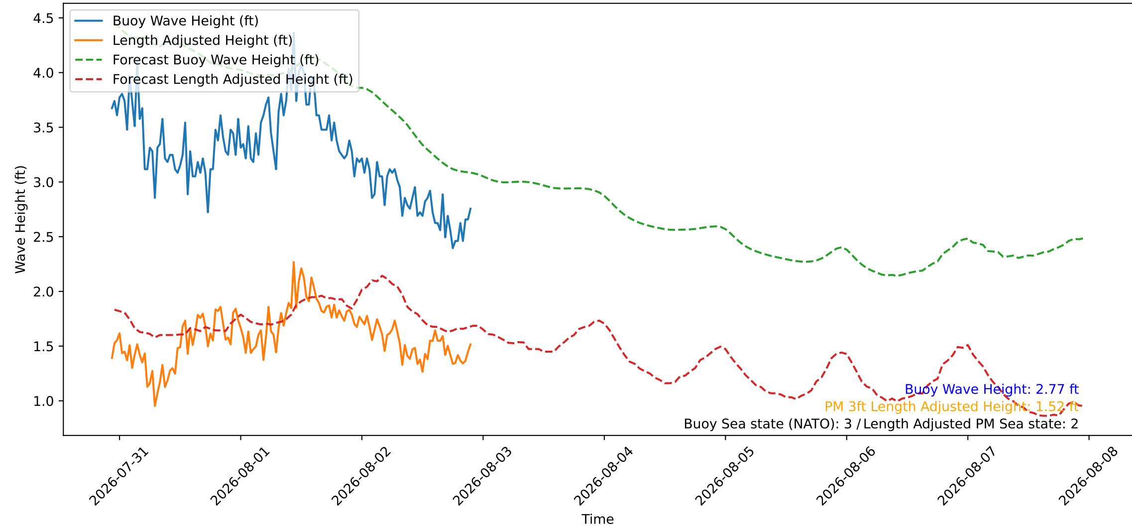
Wave Heights over Time for Oceanside Harbor at 2026-08-02 22:30:26
