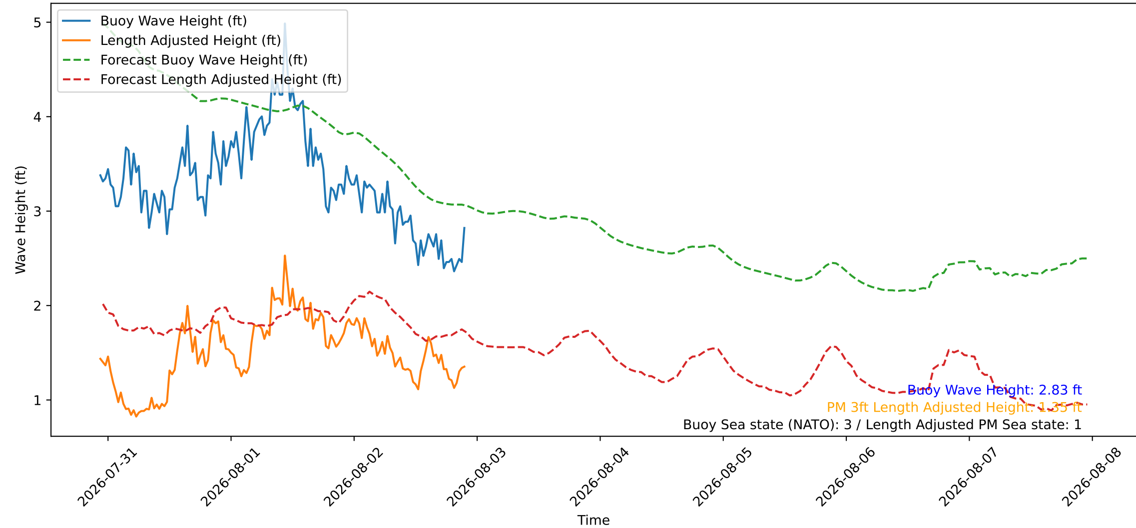
Wave Heights over Time for Green Beach at 2026-08-02 22:31:08
