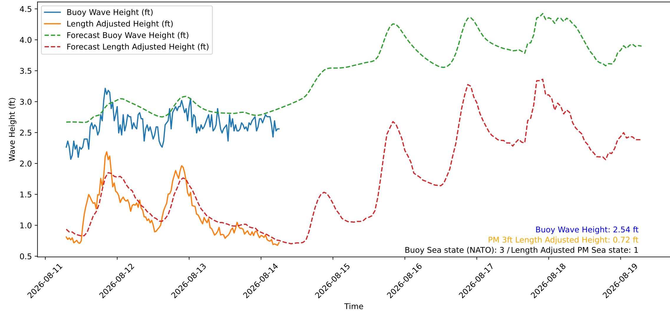
Wave Heights over Time for Green Beach at 2026-08-14 07:01:09
