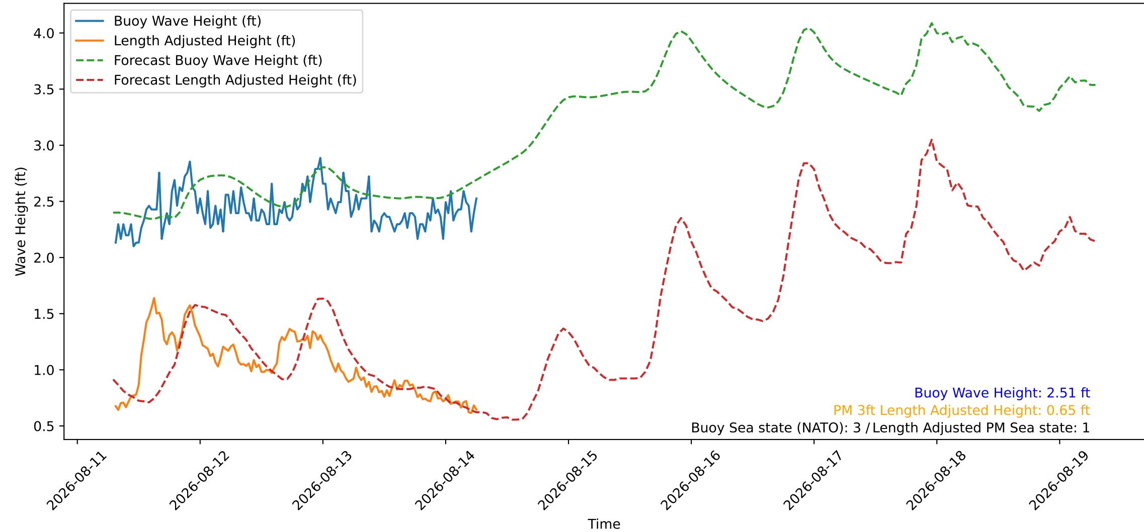
Wave Heights over Time for Red Beach at 2026-08-14 07:00:46
