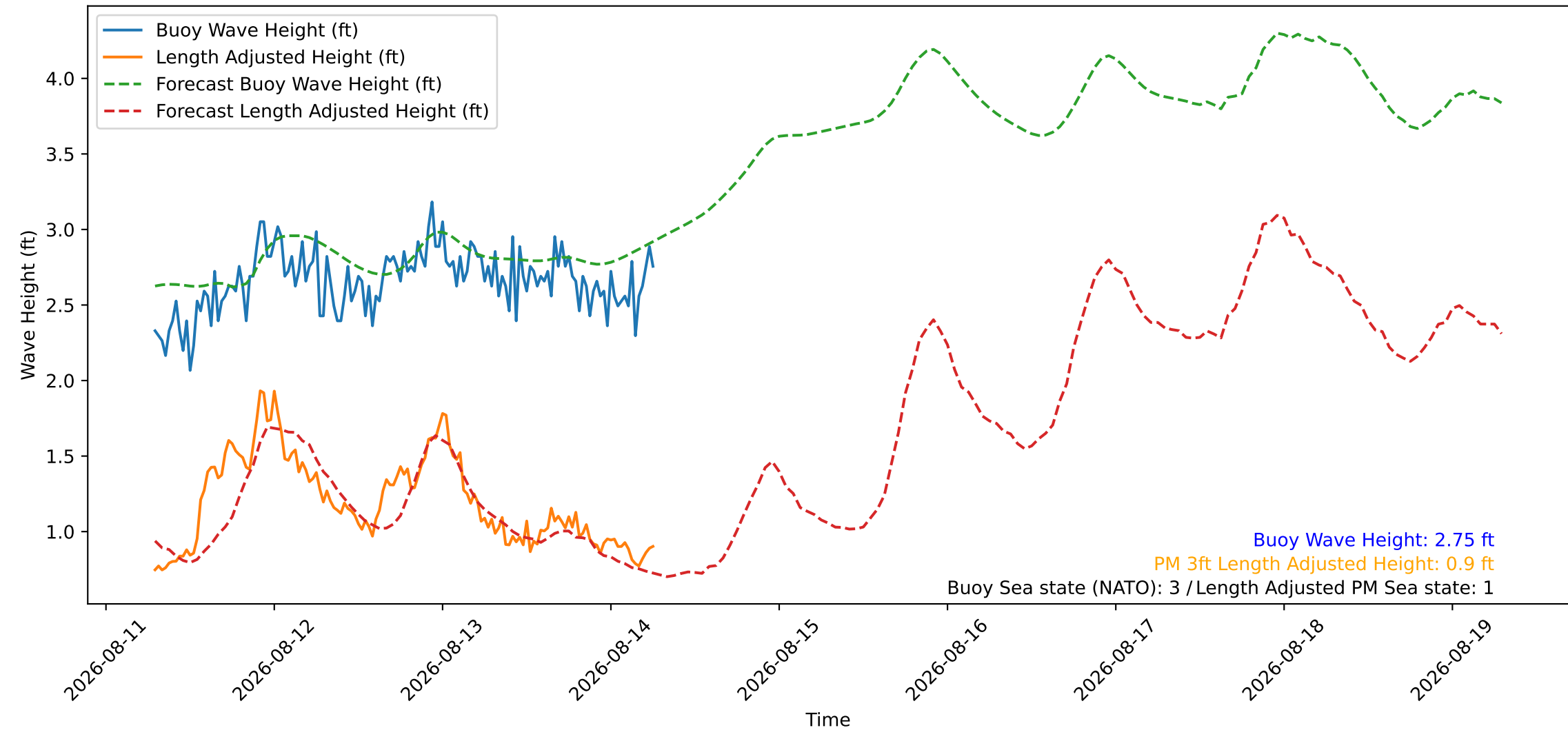
Wave Heights over Time for Oceanside Harbor at 2026-08-14 07:00:26
